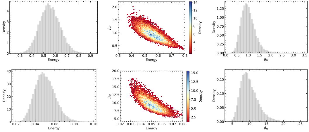
Figure 2. Thermodynamic observables of the one-dimensional U(1) lattice gauge theory on a lattice with 48 sites. The figure presents histograms of the energy (left), the measured inverse temperature \beta_M (right), and scatter plots in the form of a heat-map illustrating the relationship between energy and \beta_M (middle). The top three plots correspond to \beta = 10 , while the bottom three are for \beta = 1 . These plots highlight the fluctuations around the average values, with the heat-map scatter plots demonstrating how energy shifts as the temperature deviates from the true value.
