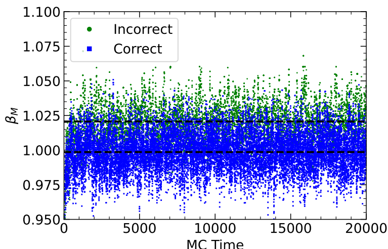
Figure 9. Comparison of the extracted \beta_M from simulations using the correct and incorrect Metropolis updates, performed at input \beta = 1.0 . The estimator captures the deviation in the incorrect case, demonstrating its sensitivity to errors in the algorithm.
