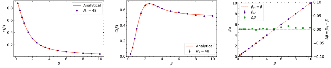
Figure 1. Thermodynamic observables for the one-dimensional U(1) lattice theory on a 48 site lattice. The energy E(\beta) (left), specific heat C(\beta) (middle), and the measured inverse temperature \beta_M (right) are plotted against the input \beta . E(\beta) and C(\beta) are benchmarked against the analytical results given in eqs. (3.15) and (3.16), respectively. The plot of \beta_M against \beta shows the expected behavior.
