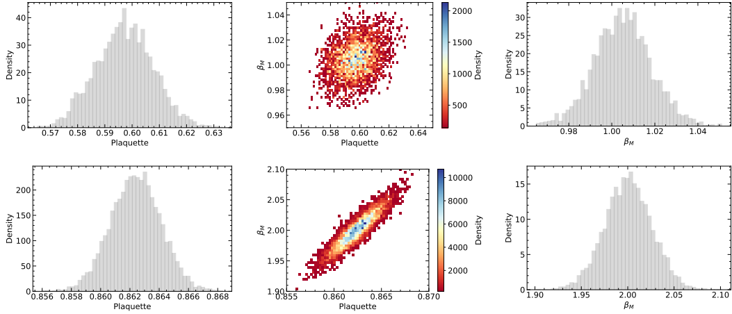
Figure 7. Thermodynamic observables for the four-dimensional U(1) lattice theory with V = 8^4 . The figure presents histograms of the plaquette (left), the measured inverse temperature \beta_M (right), and a scatter plot in the form of a heat-map illustrating the relationship between plaquette and \beta_M (middle). The top three plots correspond to \beta = 1.005 , the critical \beta , while the bottom three are for \beta = 2.0 .
