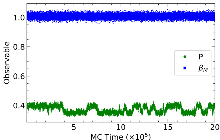
Figure 10. Monte Carlo time histories of the plaquette and \beta_M at the critical coupling \beta = 1.0075 on an 8^4 lattice.
