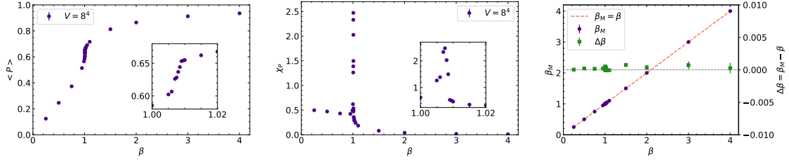
Figure 6. Thermodynamic observables for the four-dimensional U(1) lattice theory on an 8^4 lattice. The plaquette \langle P \rangle (left), the plaquette susceptibility \chi_P (middle), and the estimated inverse temperature \beta_M (right) are plotted against the input temperature \beta .
