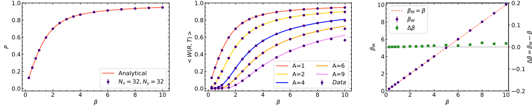
Figure 4. Two-dimensional U(1) lattice gauge theory. The expectation value of plaquette, Wilson loops of sizes A = R \times T and estimated inverse temperature \beta_M as functions of input \beta are shown on a 32 \times 32 lattice.
