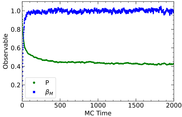
Figure 8. The initial part of Monte Carlo time history, including thermalization, of the plaquette and \beta_M on an 8^4 lattice at \beta = 1.0 .
