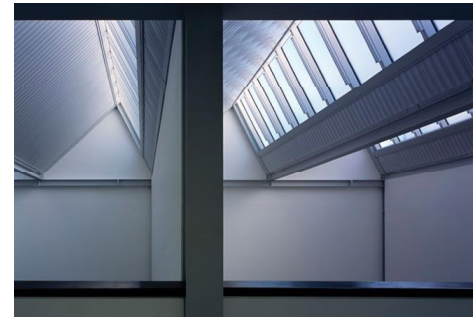
Fig 100, New lightweight steel roof structure allowing daylighting into studio spaces
