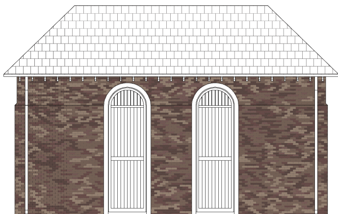
Front Elevation, Double Giraffe House
