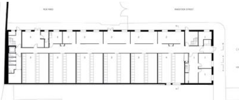
Fig 101, Floor Plan, existing brickwork enclosure with new internal divisions
