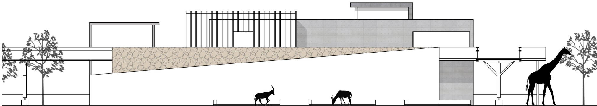
North Elevation
