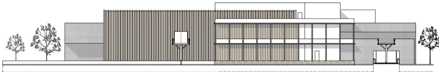
East Elevation 0 1 3 5 10m
