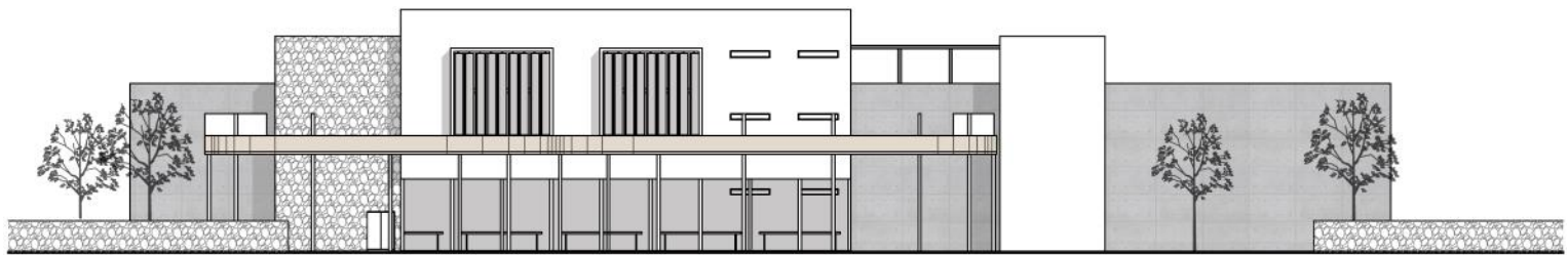
West Elevation 0 1 3 5 10m
