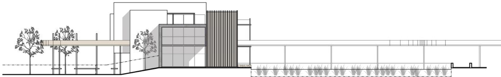
South Elevation 0 1 3 5 10m
