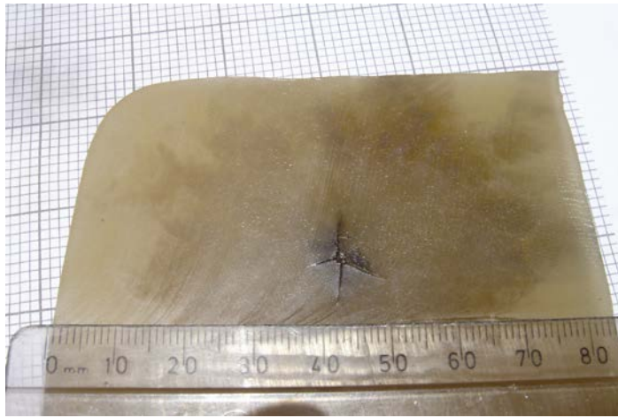
Figure 4.11: Axial view. Corbin's gel. 10 kV. (7,30 kA). Temporary cavity formation demonstrated in the harder gelatine media. Small fissure fracture noted similar to that seen in projectile testing experiments. The current strength measured 7,30 kA.
