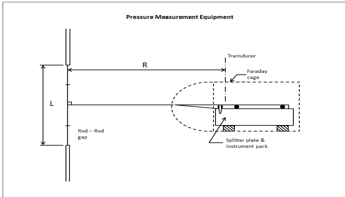
Figure 2.2: The experimental layout of McKelvie, Page and Mackerras' experiment. (7 th Australasian Hydraulics and Fluid Mechanics Conference, Brisbane, 18-22 August, 1980).
