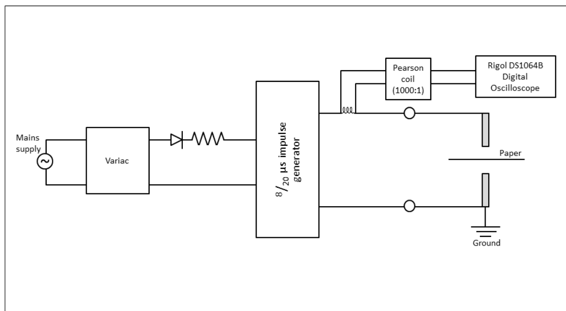
Figure 4.14: The 2014 'sixth mechanism paper experiment': Physical layout of current impulse generator and test object (graph paper)
