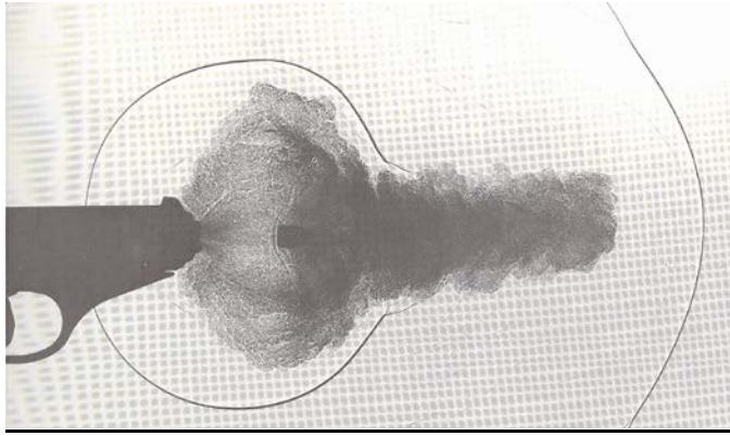
Figure 4.2: Gas flows at a muzzle having just fired a shot. Note the shock wave at the tail of the bullet, showing the high gas velocity (Sellier & Kneubuehl, 1994).
