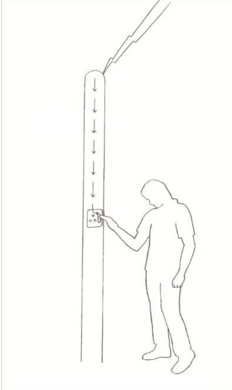
Figure 1.2: The second mechanism of lightning injury: Indirect strike.
