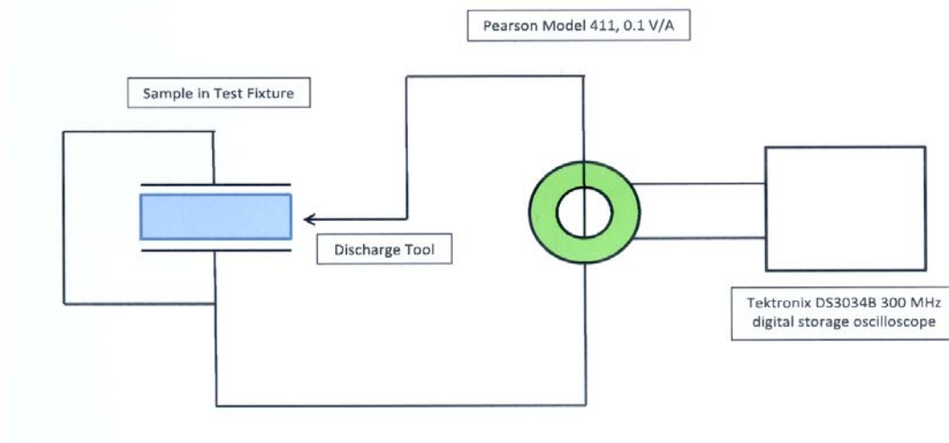
Figure 2.6: Schematic diagram of Hickman's experiment.
