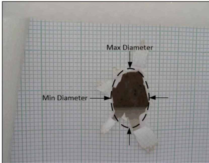
Figure 4.17: Tearing and tattering of dry graph paper to a maximum diameter of 29 mm. 15 kV. 24 kA.
