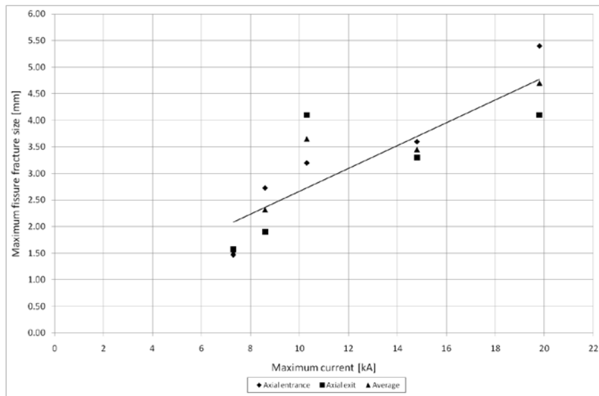
Figure 4.13: Graph demonstrating incremental fissure/fracture cracks in Corbin's gel. As the current increased through the wire, the size of the temporary cavity also increased in a directly proportional manner
