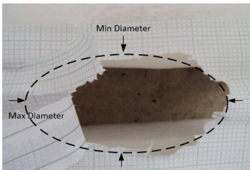
Figure 4.18: Tearing and tattering of saline-soaked graph paper to a maximum diameter of 80 mm. 20 kV. 32,8 kA.
