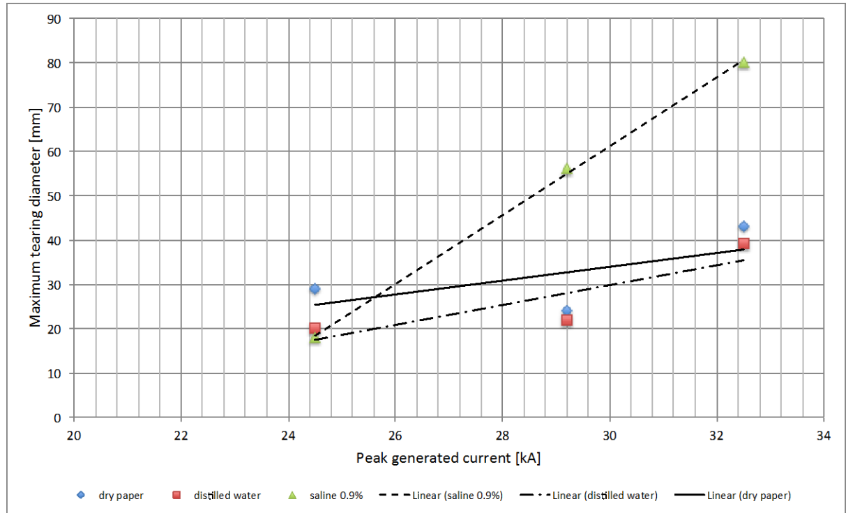
Figure 4.19: Trend lines showing significantly higher tearing of the paper soaked in 0.9% saline solution.
