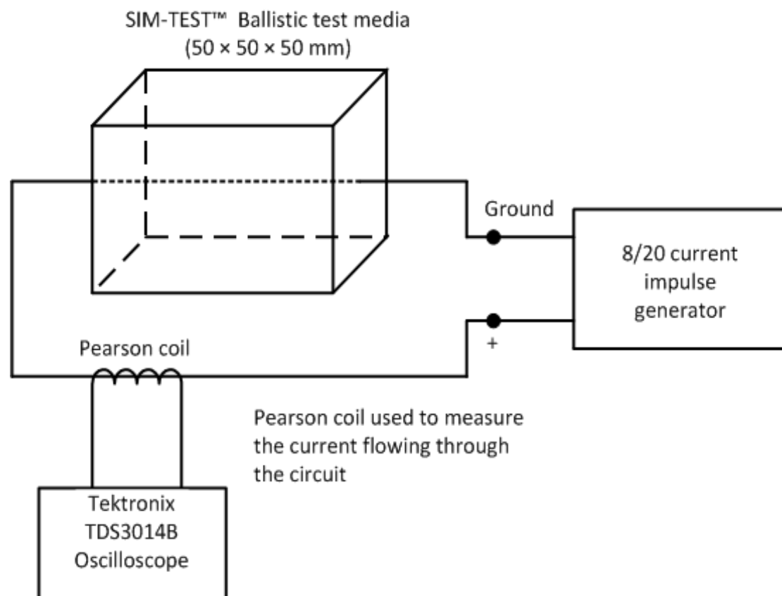
Figure 4.4: The 2012 ‘sixth mechanism gel experiment’: Physical layout of current impulse generator and test object (the gelatine block).
