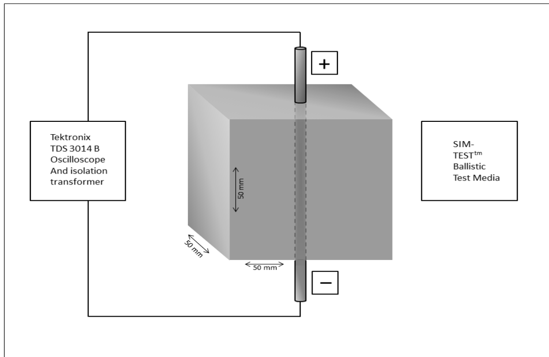
Figure 4.5: Three dimensional view of the 2012 'sixth mechanism gel experiment'.
