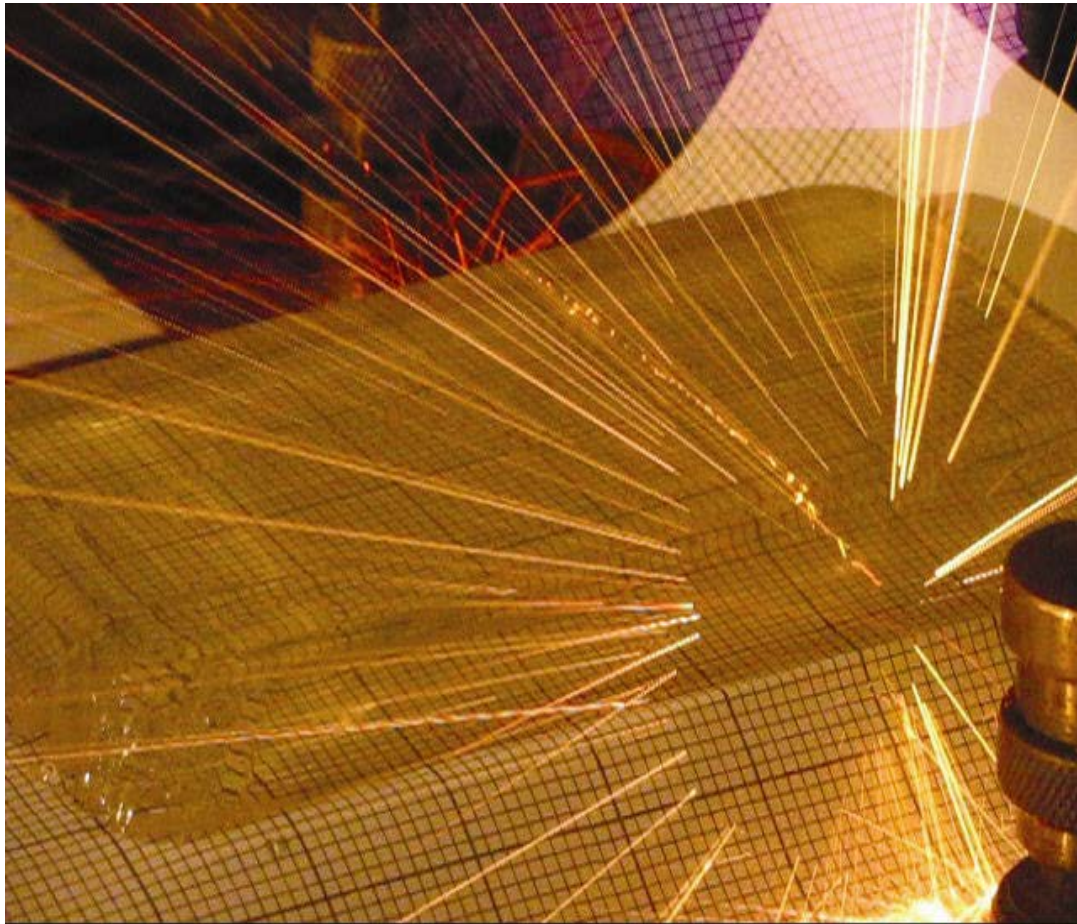
Figure 4.6: High-speed camera footage showing the moment of impulse generation. Note the radial explosion from the wire. The propagation mode of the blast wave through the jelly was visibly noted. Current impulse generated through gel showing radial explosion.
