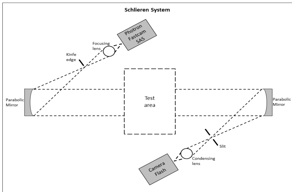
Figure 6.1: Proposed Z-configuration Schlieren test to photograph the lightning blast wave around a spark.
