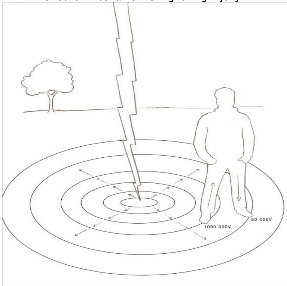
Figure 1.4: The fourth mechanism of lightning injury: Step potential.
