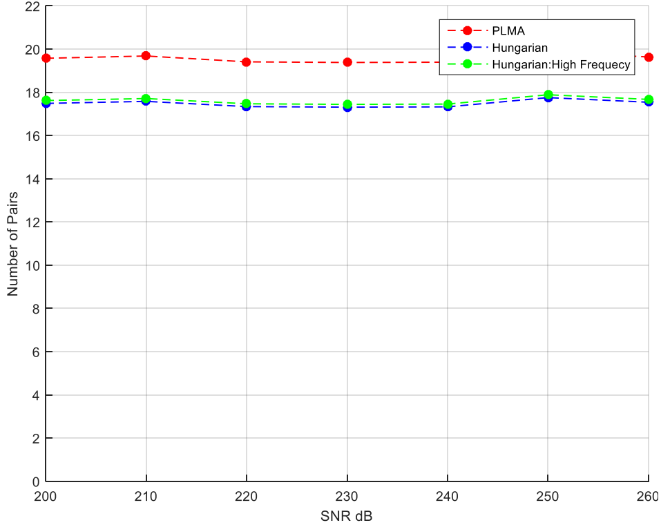
Figure 5. 15 Number of SU_k and SU_l user pairs among different SNR levels using Lagrange based power allocation.
