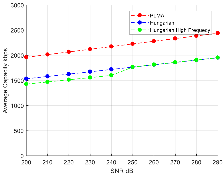
Figure 5. 14 PLMA algorithm performance with the bound based power allocation scheme.
