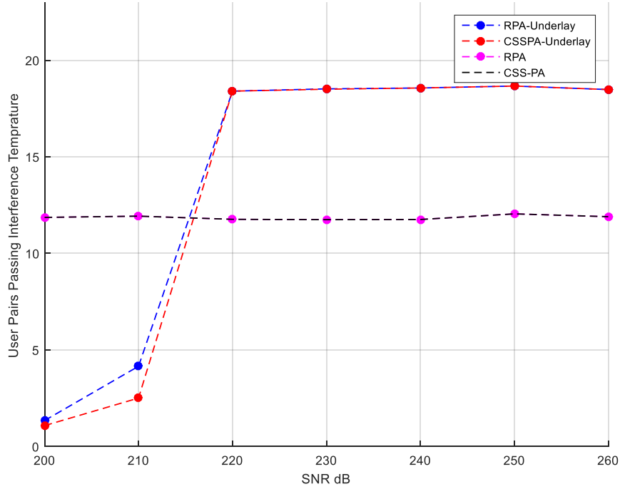
Figure 5. 7 Number of SU_k and SU_l user pairs passing PU interference test using bound based power allocation scheme for Underlay schemes.
