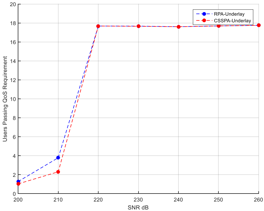
Figure 5. 9 Users that pass the underlay QoS requirements using the bound based power allocation scheme for Underlay schemes.
