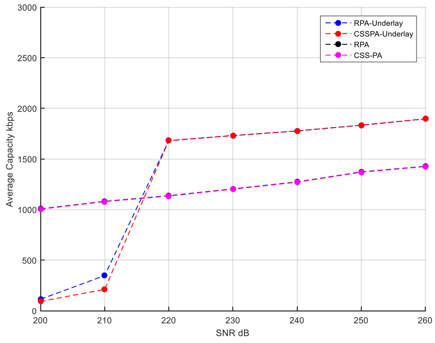
Figure 5. 2 Average Capacities for each pairing algorithm Lagrange based power allocation scheme for Underlay schemes.
