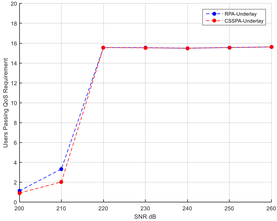
Figure 5. 8 Users that pass the underlay QoS requirements using Lagrange based power allocation scheme for Underlay schemes.
