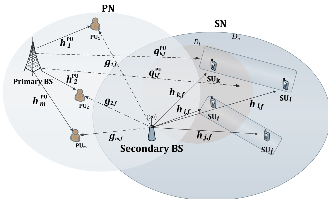
Figure 4. 1 The system model showing users SU_k and SU_l in a CR-NOMA system.
