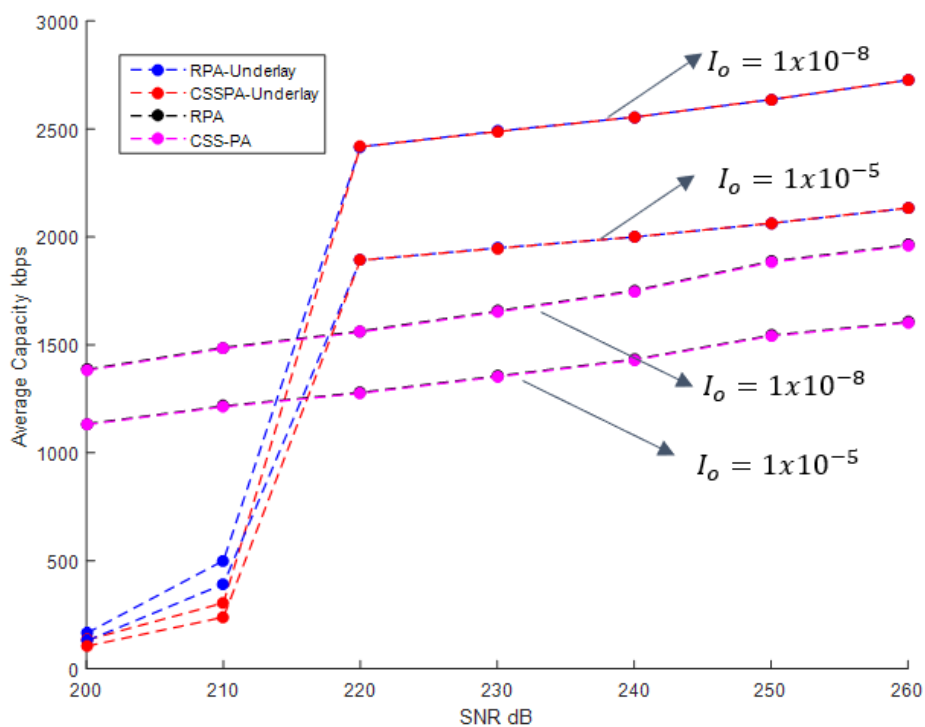
Figure 5.10 How the change of the constant I_o affects the average user capacity.
