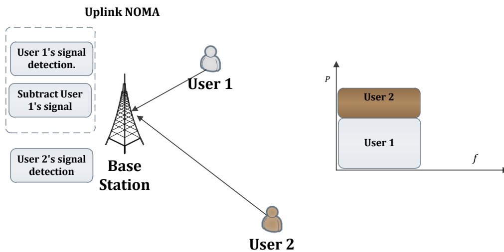
Figure 2. 4 Uplink NOMA with SIC
