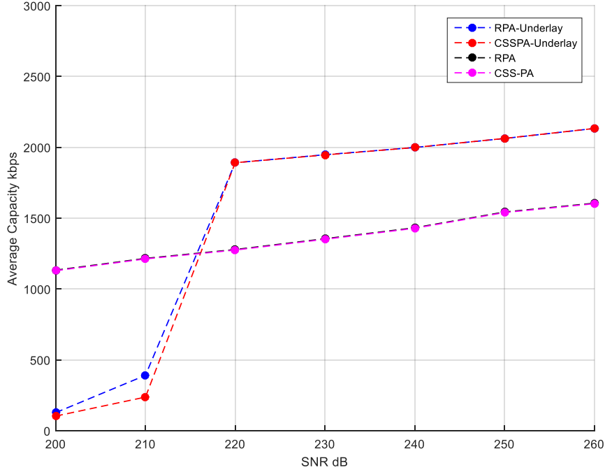
Figure 5. 3 Average Capacities for each pairing algorithm using bound based power allocation for underlay schemes.
