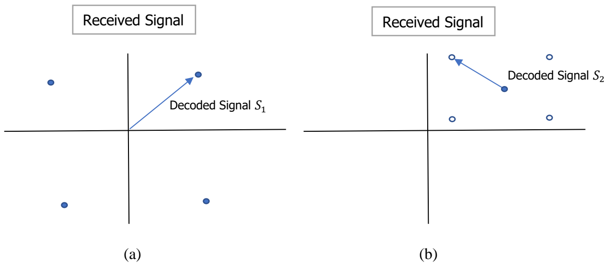
Figure 2. 2 NOMA receiver end decoding scheme.
