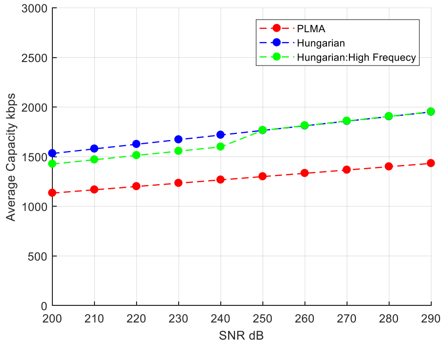
Figure 5.12 PLMA algorithm performance with Lagrange based power allocation scheme.
