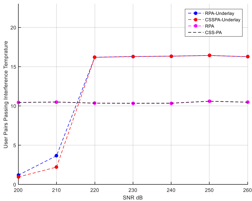
Figure 5. 6 Number of SU_k and SU_l user pairs passing PU interference test using Lagrange based power allocation scheme for Underlay schemes.
