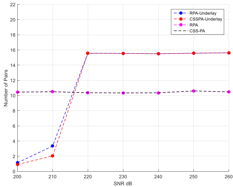
Figure 5.4 Number of SU_k and SU_l user pairs among different SNR levels using Lagrange based power allocation scheme for Underlay schemes.
