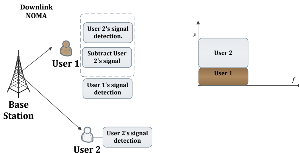
Figure 2. 3 Downlink NOMA with SIC
