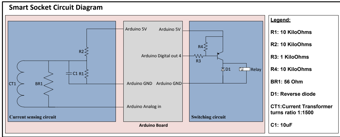
Figure 4: Smart Socket Circuit Diagram
