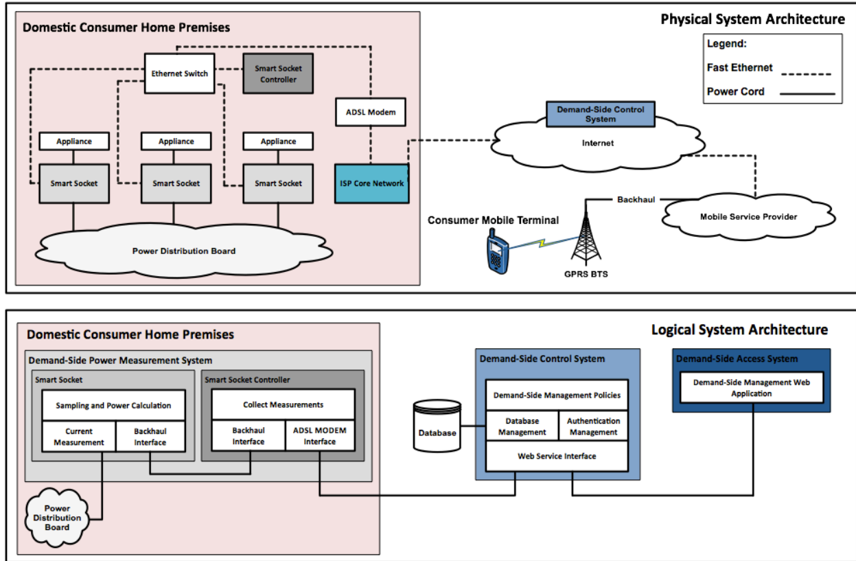
Figure 3: Physical and Logical system diagram
