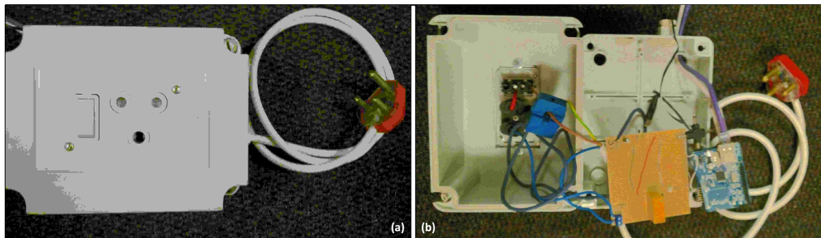
Figure 5: Smart Socket Snapshots
