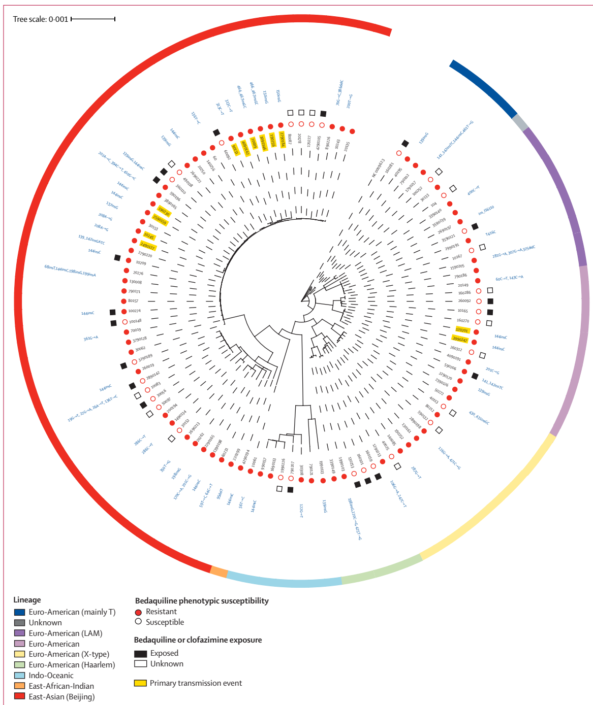
Figure 2: Maximum likelihood phylogenetic tree of 104 baseline Mycobacterium tuberculosis strains 104 strains are shown: 76 baseline bedaquiline-resistant strains and 34 strains with either a documented or unknown exposure to bedaquiline or clofazimine before bedaquiline treatment initiation. From inner ring to the outer, the figure shows the study identifier for each strain, bedaquiline susceptibility, bedaquiline or clofazimine exposure, Rv0678 mutations detected, and lineage. Primary transmission events are highlighted in yellow.
