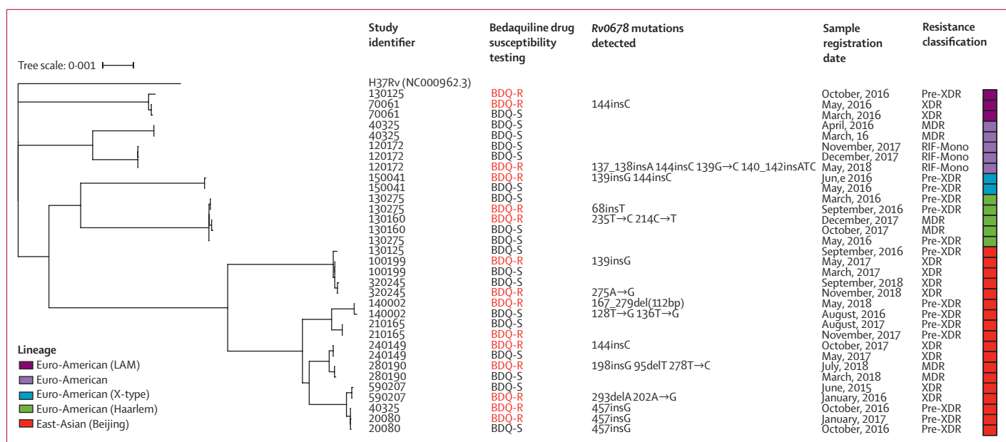
Figure 3: Maximum likelihood phylogenetic tree of 34-paired baseline and post-baseline patient isolates
