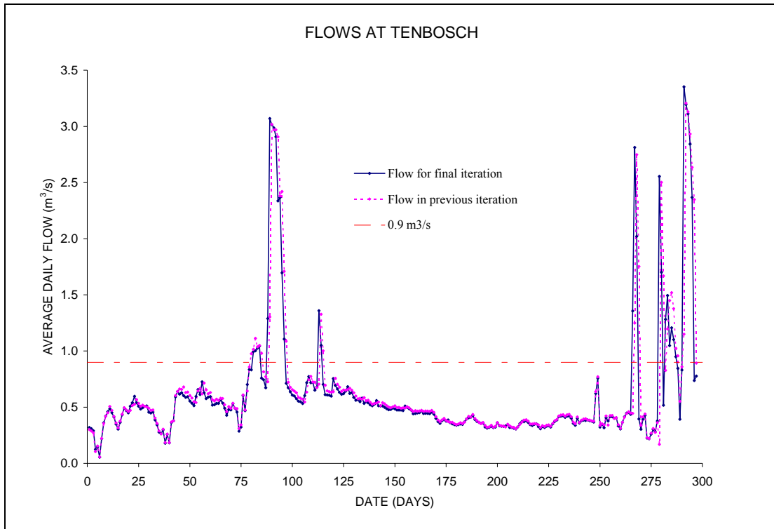
Figure 5.3: Iterative determination of daily flow at Tenbosch with 3.78\text{m}^3/\text{s} release from Kwena dam
