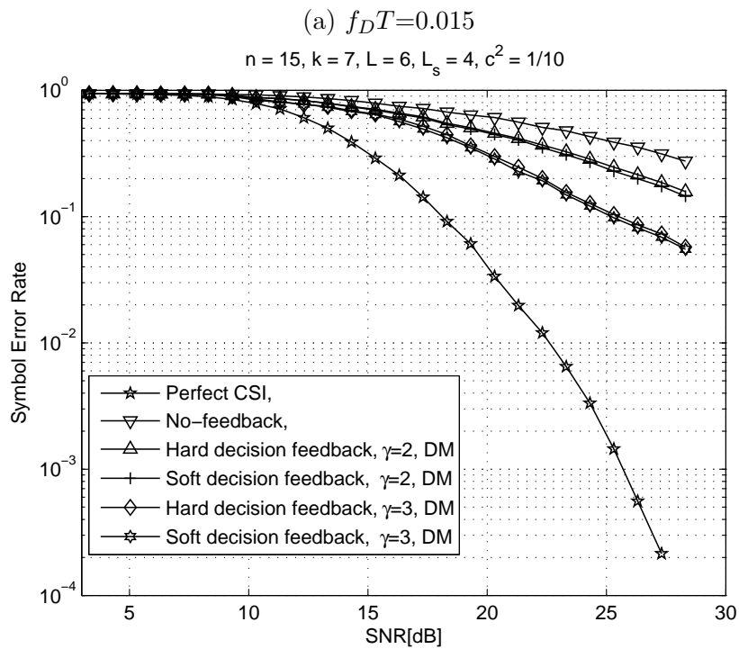
FIGURE 4.5: Receiver performance in terms of SER versus SNR using the DM method
