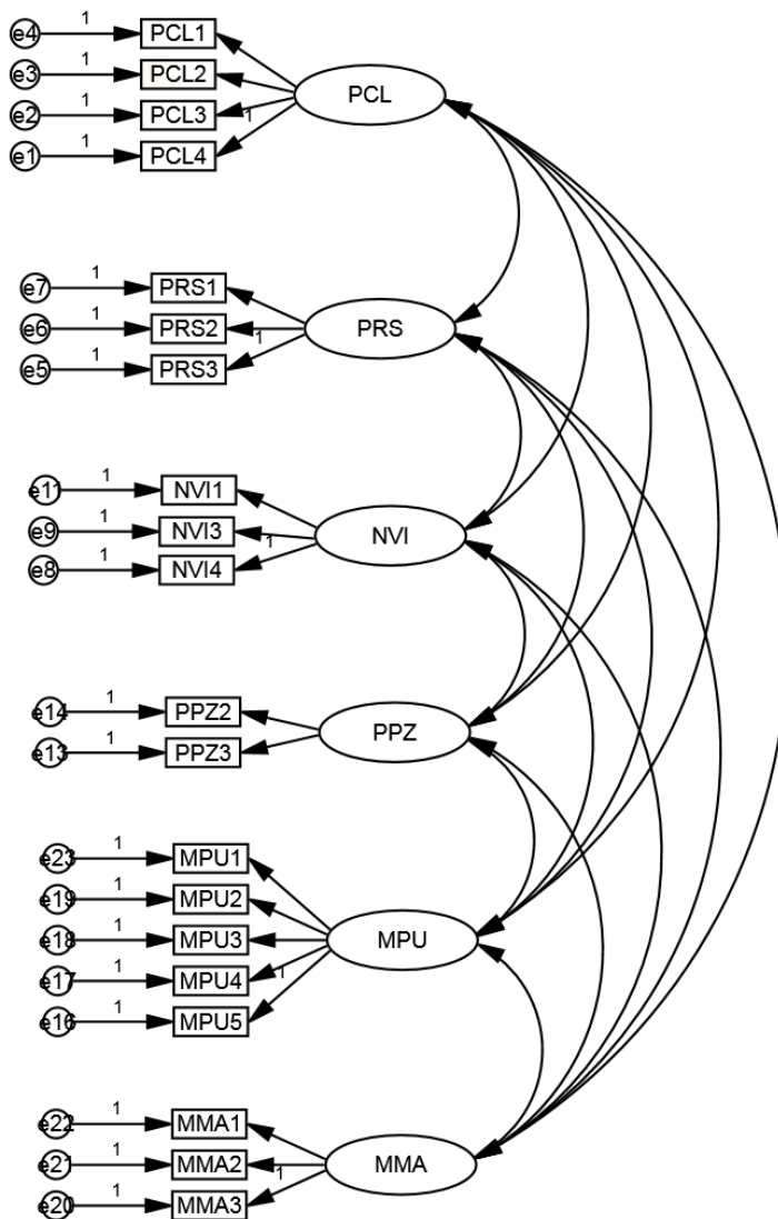
Figure 3: CFA Model
