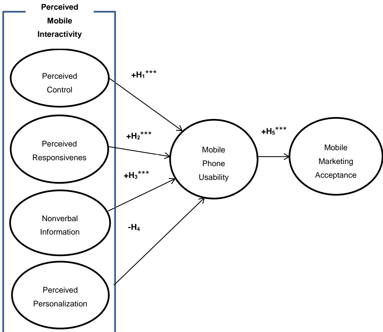
Figure 5: Proposed Model
