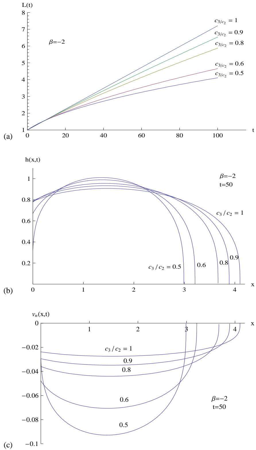
Figure 4.9.7: Graphs for \beta = -2 and a selection of values of \frac{c_3}{c_2} : (a) Fracture length L(t) plotted against time; (b) Fracture half-width h(x, t) plotted against x at time t = 50 ; (c) Leak-off fluid velocity v_n(x, t) plotted against x at time t = 50 .
