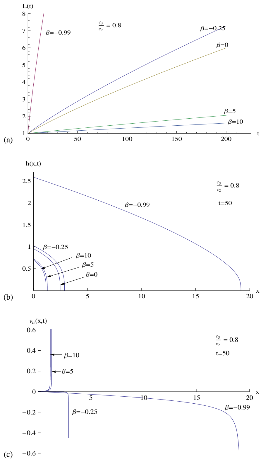
Figure 5.8.5: Graphs for \frac{c_3}{c_2} = 0.8 and a selection of values of \beta : (a) Fracture length L(t) plotted against time; (b) Fracture half-width h(x,t) plotted against x at time t = 50 ; (c) Leak-off fluid velocity v_n(x,t) plotted against x at time t = 50 .
