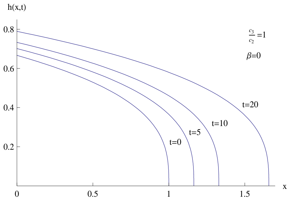
Figure 4.6.6: Fracture half-width, h(x, t) , given by (4.5.19) plotted against x for a range of values of t and for \frac{c_3}{c_2} = 1 , \beta = 0 . The leak-off velocity at the fluid/rock interface, v_n(x, t) , given by (4.5.20), is zero.
