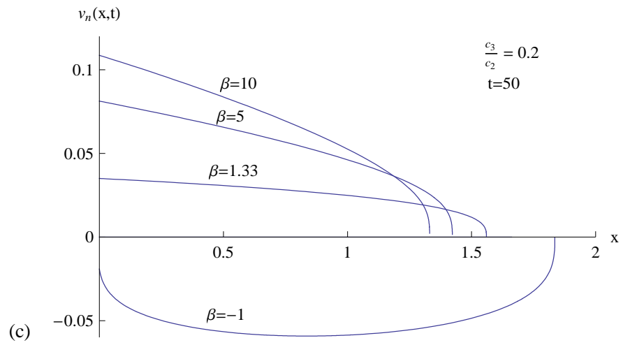
Figure 4.9.3: Graphs for \frac{c_3}{c_2} = 0.2 and a selection of values of \beta : (a) Fracture length L(t) plotted against time; (b) Fracture half-width h(x, t) plotted against x at time t = 50 ; (c) Leak-off fluid velocity v_n(x, t) plotted against x at time t = 50 .
