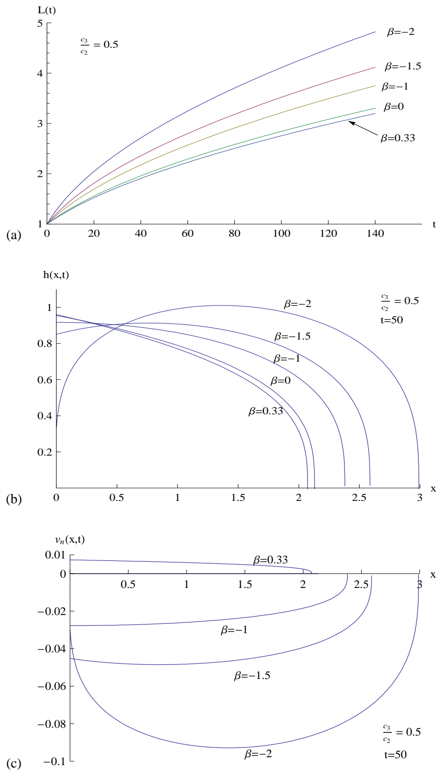
Figure 4.9.4: Graphs for \frac{c_3}{c_2} = 0.5 and a selection of values of \beta : (a) Fracture length L(t) plotted against time; (b) Fracture half-width h(x, t) plotted against x at time t = 50 ; (c) Leak-off fluid velocity v_n(x, t) plotted against x at time t = 50 .
