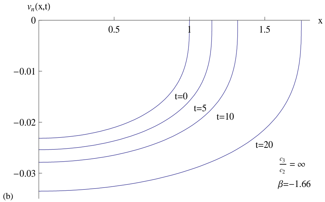
Figure 4.4.10: (a) Fracture half-width, h(x,t) , given by (4.3.25) and (b) leak-off velocity at the fluid/rock interface, v_n(x,t) , given by (4.3.26), plotted against x for a range of values of t and for \frac{c_3}{c_2} = \infty , \beta = -1.66 .
