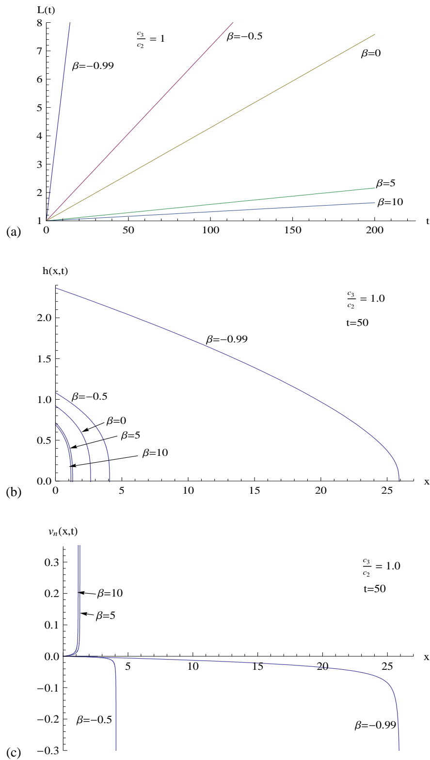
Figure 5.8.6: Graphs for \frac{c_3}{c_2} = 1 and a selection of values of \beta : (a) Fracture length L(t) plotted against time; (b) Fracture half-width h(x, t) plotted against x at time t = 50 ; (c) Leak-off fluid velocity v_n(x, t) plotted against x at time t = 50 .
