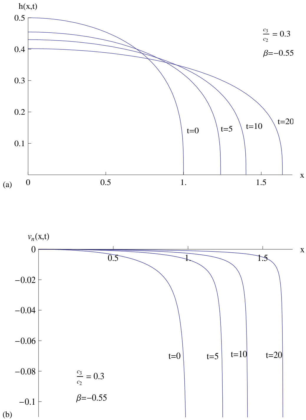
Figure 5.3.6: (a) Fracture half-width, h(x,t) , given by (5.3.17) and (b) leak-off velocity at the fluid/rock interface, v_n(x,t) , given by (5.3.18), plotted against x for a range of values of t and for \frac{c_3}{c_2} = 0.3, \beta = -0.55 .
