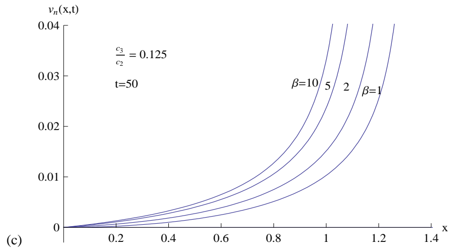
Figure 5.8.2: Graphs for \frac{c_3}{c_2} = 0.125 and a selection of values of \beta : (a) Fracture length L(t) plotted against time; (b) Fracture half-width h(x, t) plotted against x at time t = 50 ; (c) Leak-off fluid velocity v_n(x, t) plotted against x at time t = 50 .
