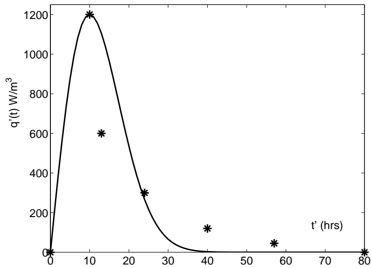
Figure 2: Typical adiabatic heat rate data and approximation given by equation (3)
