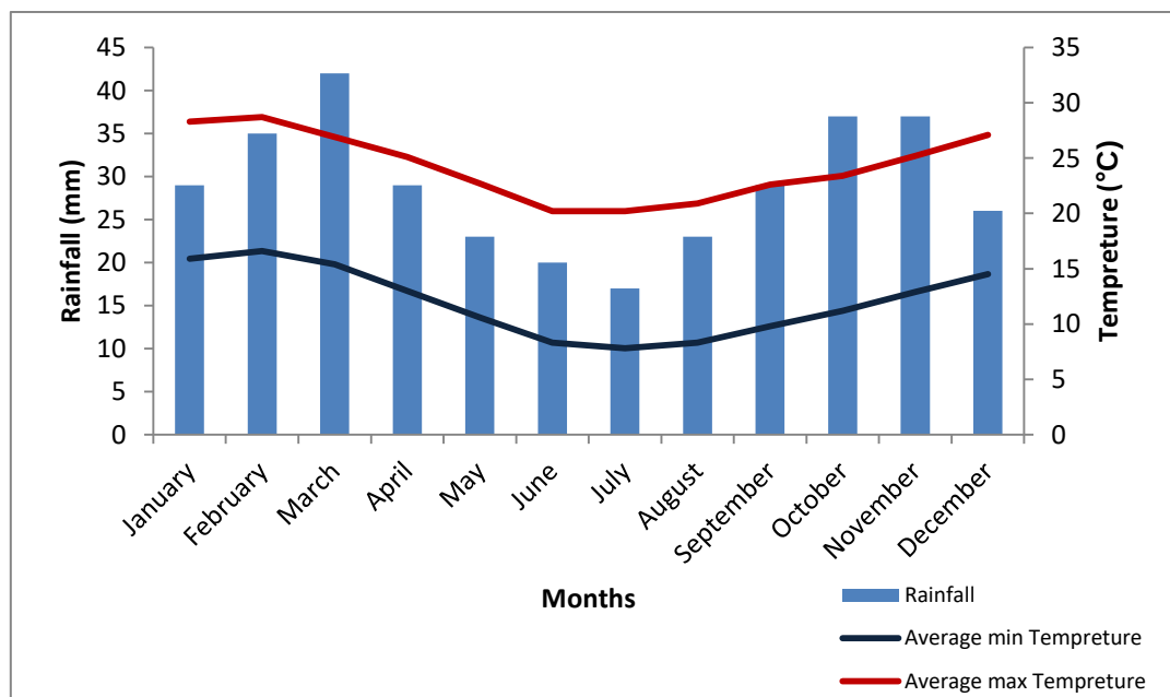
Figure 3. 2: Monthly average climate variables calculated over 25 years in Shamwari Private Game Reserve (Schulze, 2007).
