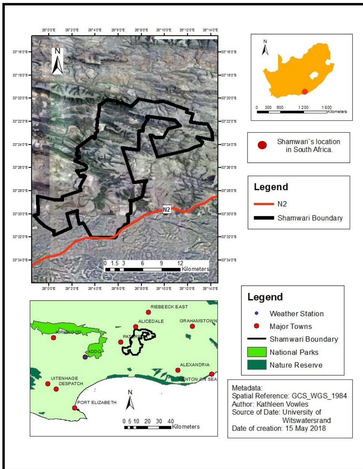
Figure 3. 1: Location of Shamwari Private Game Reserve in the Eastern Cape, South Africa.
