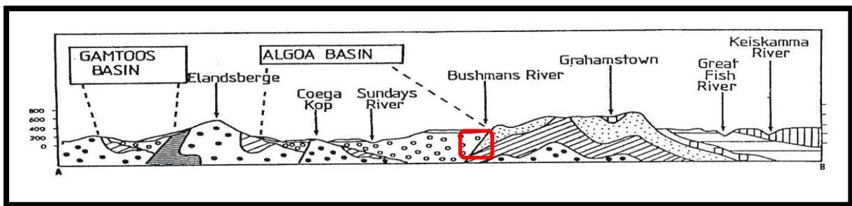
Figure 3. 3: Cross section from the Gamtoos Basin to beyond the Fish River (Büttner et al. , 2015). Research site indicated by red square, legend for this figure provided below in Figure 3.4.
