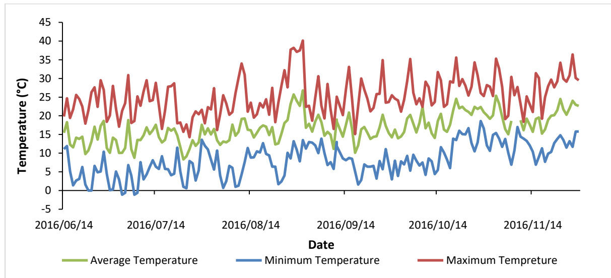
Figure 5. 1: Daily average, maximum, and minimum temperature over the study period (June–November 2016).
