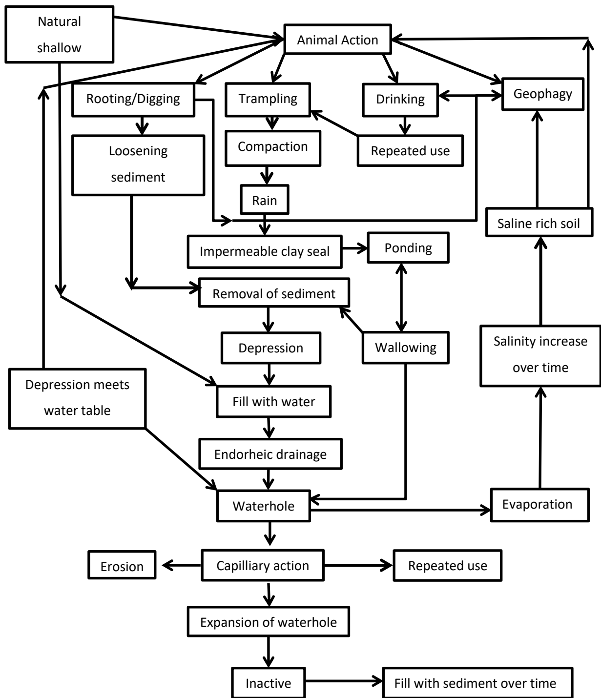
Figure 2. 1: Model of the formation of naturally-forming waterholes.
