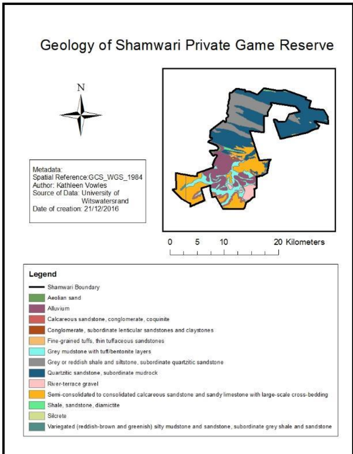
Appendix 1: Geological map of Shamwari Private Game Reserve. Specific site locations were withheld due to the unfortunate reality of poaching in South Africa.
