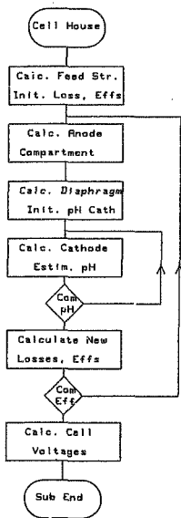
Figure 6. Flowchart of Cell House Section.
