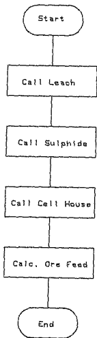
Figure 2. Model Flowchart
