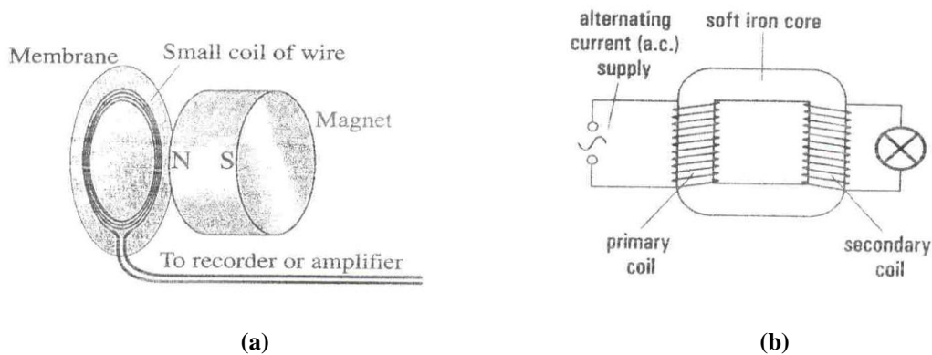
Figure 5.5: Diagrams of a microphone (Giancoli, 2005) and a transformer (Broster et al. , 2006)
