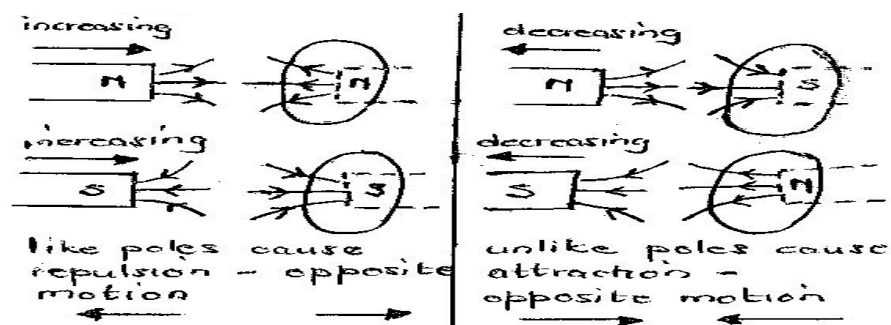
Figure 6.12: Diagrams showing the motion of conductor and magnet for increasing flux and decreasing flux.
