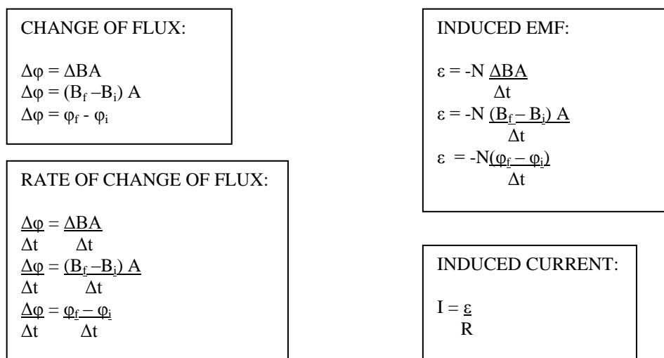
Figure 5.7: Related equations of EMI
