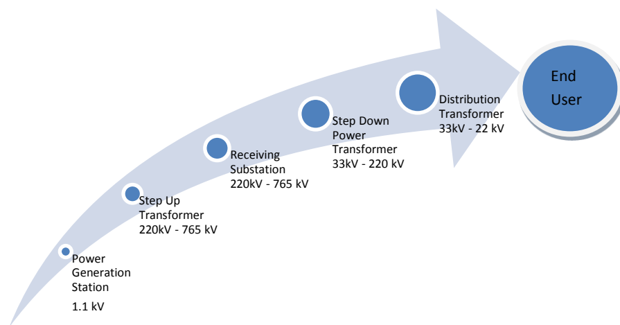
Figure1; Electric Power Distribution (Generation to End Consumption)
