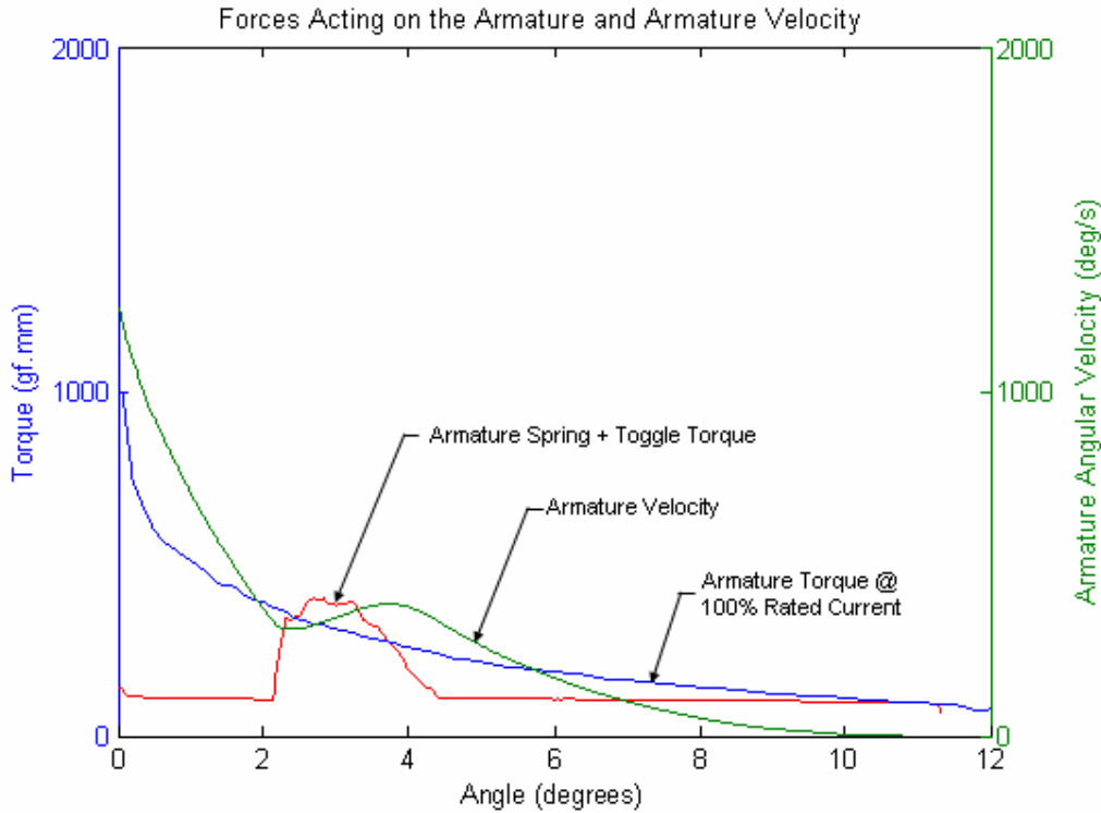
Figure 5.2: Armature Motion at the ARP.
