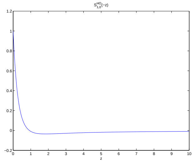
Figure 4.4: The symbol of the fifth order scheme, S_{1,0}^{HO}(-z) .
