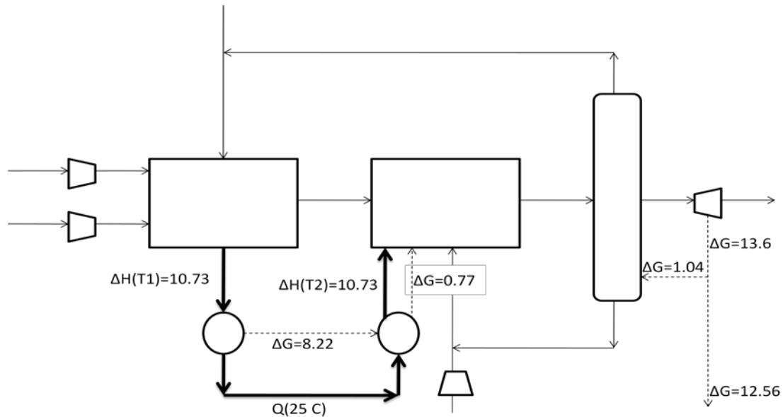
Figure 3.21: Flow of heat (thick solid lines) and work (dashed lines) for Flowsheet, Figure 3.20
