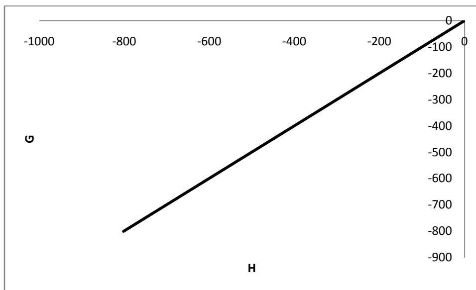
Figure 4.11: The set of all combustion extents with 0 \leq \epsilon \leq 1
