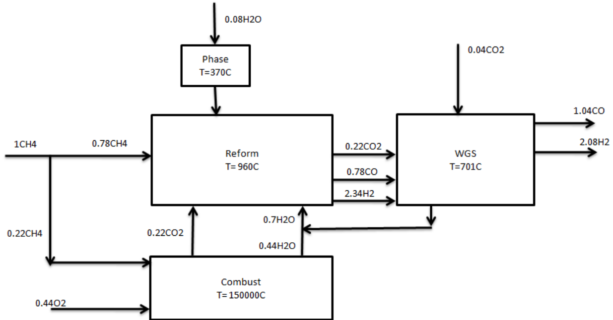
Figure 3.13: Postulate reformer flow sheet 1 using process Carnot temperatures
