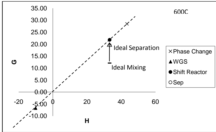
Figure 2.20: Shift reactor at 600°C with ideal mixing and ideal separation
