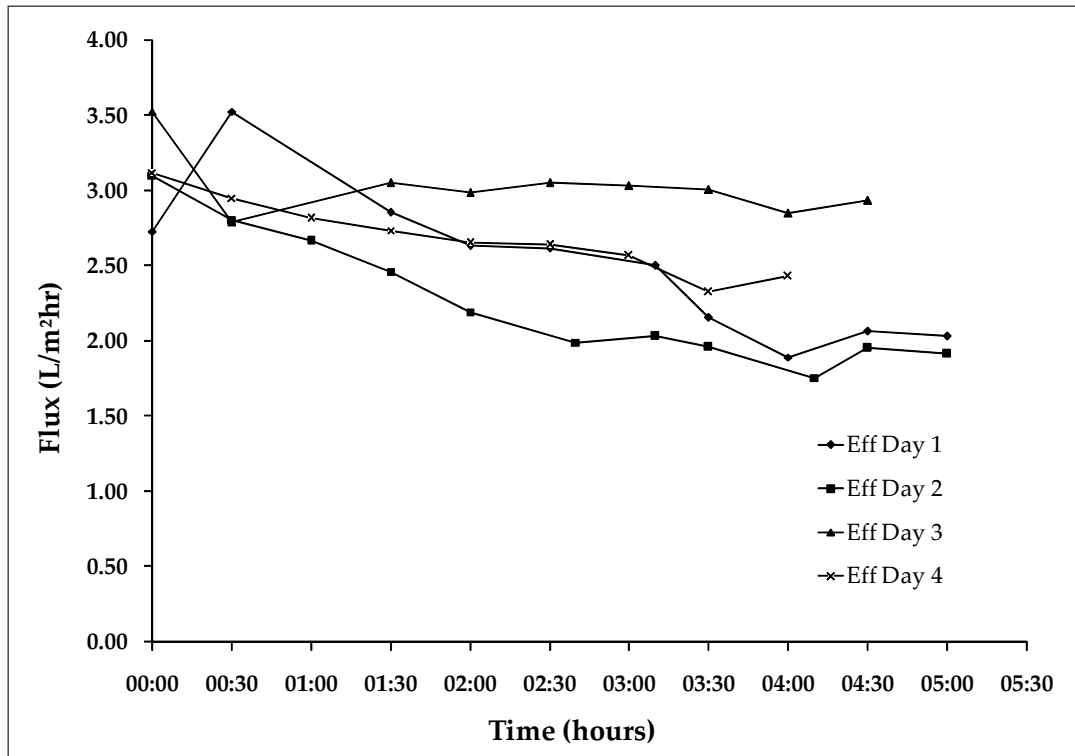
Figure A.9: Graph showing the flux from the 4 day test (of 5 hours per day) on the membrane.
