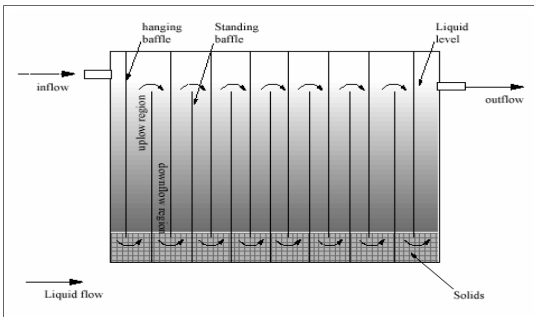
Figure 1.2: A simple plan of an ABR, showing water flow patterns (Foxon et al., 2001).
