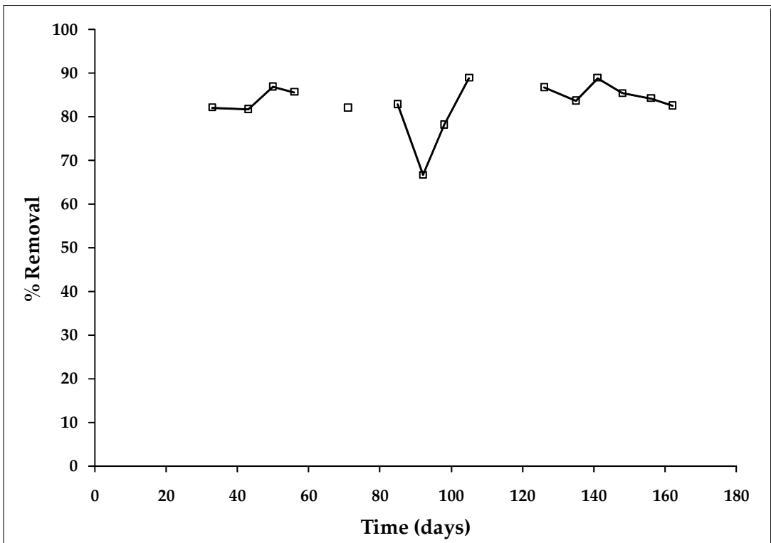
Figure 4.3: Percent removal of COD by the ABR for the duration of the study period.
