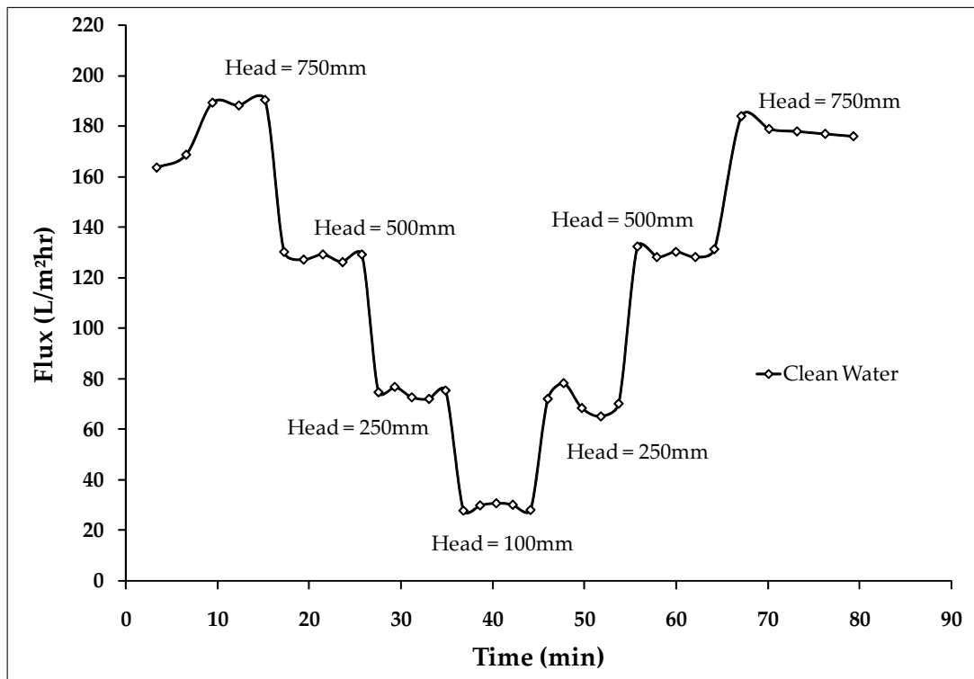
Figure A.4: Clean water flux at each head from 100 mm to 750 mm.
