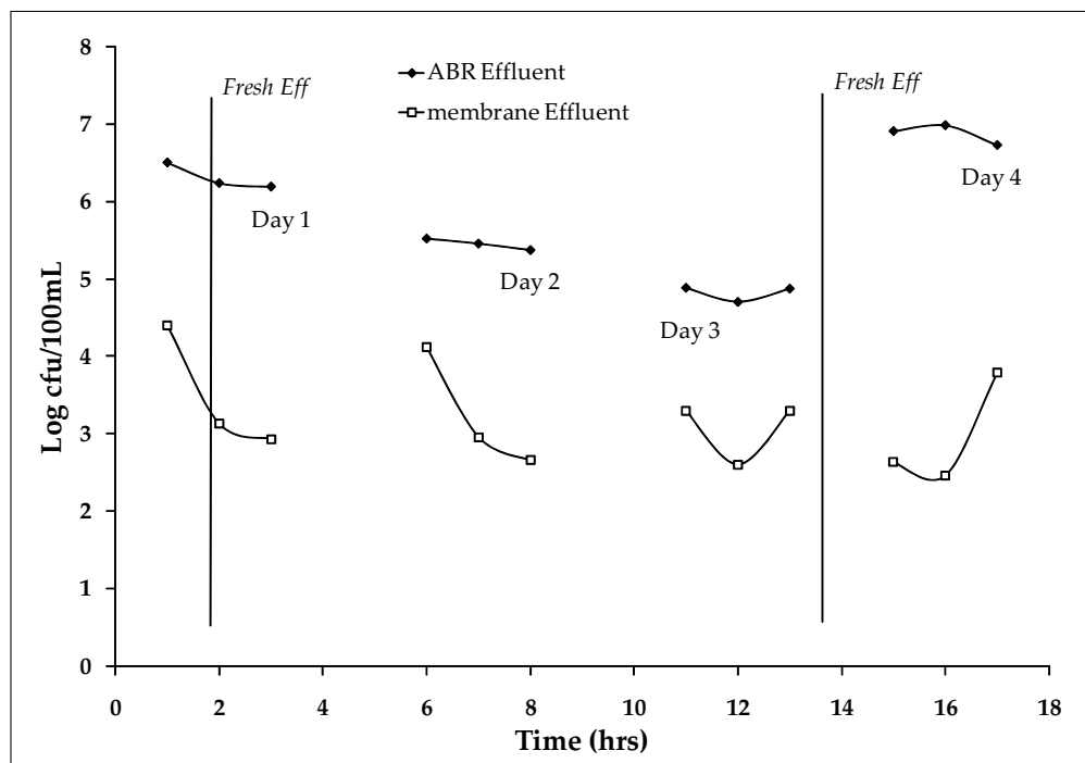
Figure A.13: Membrane removal of coliforms; showing the log values of colony-forming units pre- and post- filtering through the membrane. The vertical lines show when fresh ABR effluent was collected.
