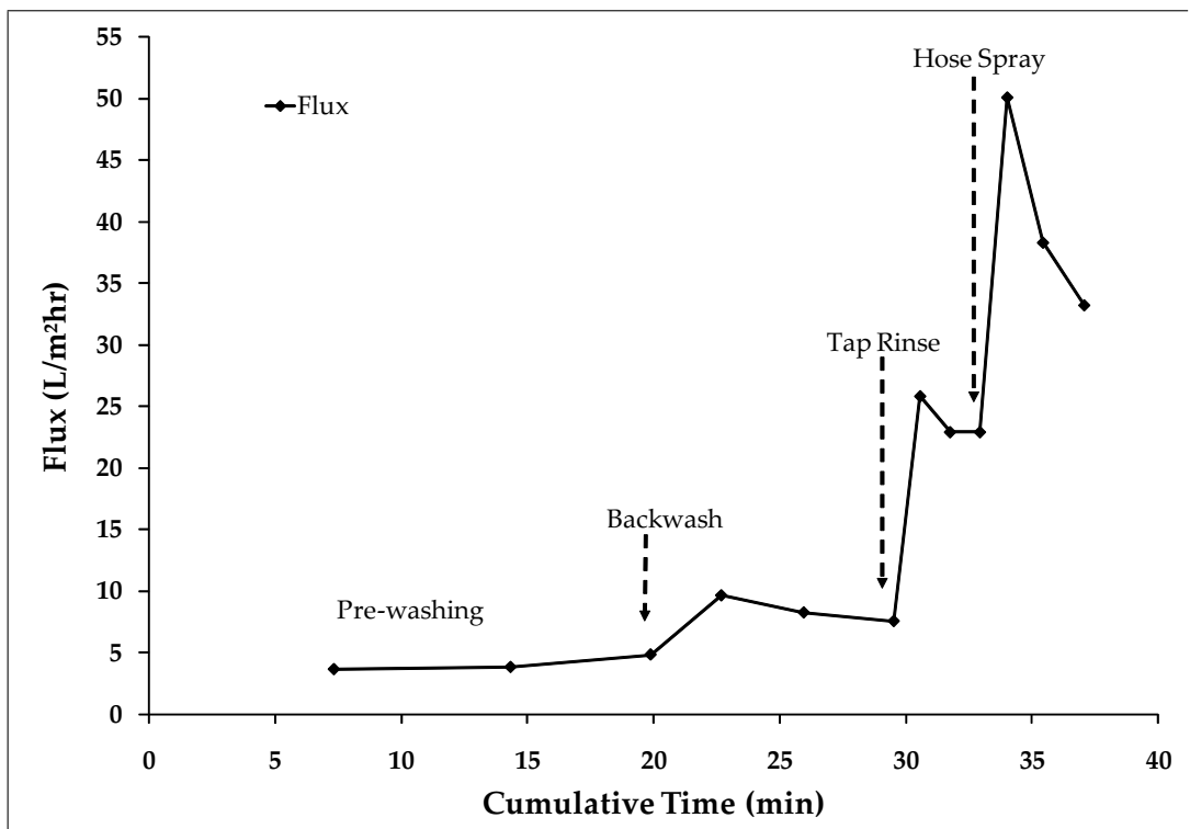
Figure A.7: Flux prior to cleaning and after backwashing, tap-rinsing and pressured spray.
