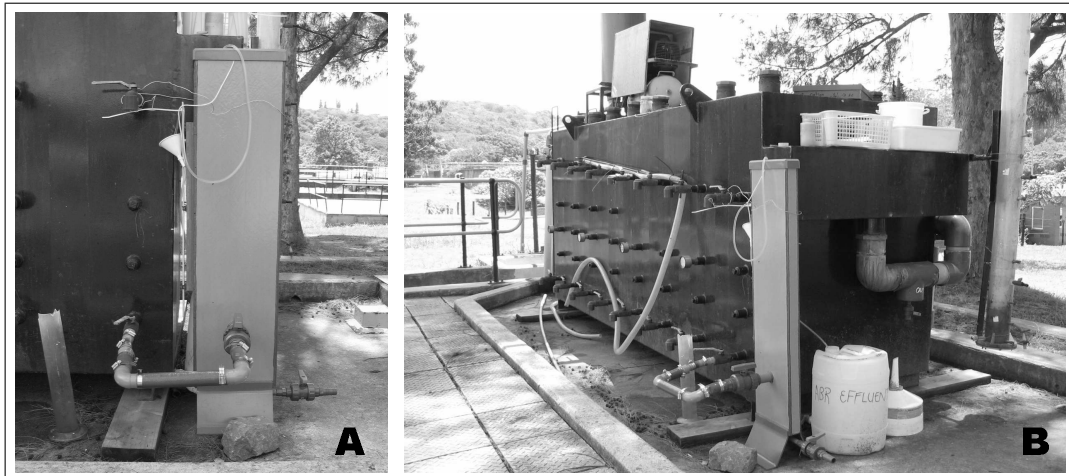
Figure A.2: (a) shows a side view of the membrane unit after it was installed and (b) shows the ABR, unit and the membrane effluent collection vessel.
