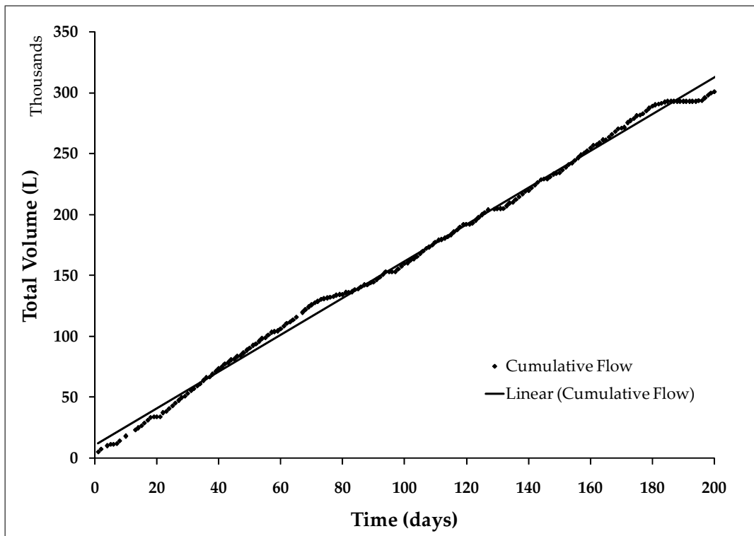
Figure 4.1: Cumulative flow for the duration of the study period.
