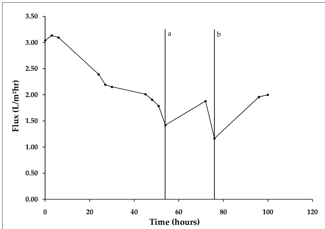
Figure A.10: Graph showing flux over time, for 5 consecutive days. The lines a and b indicate the times when the water level in the unit dropped, reducing the head and stopping flow.
