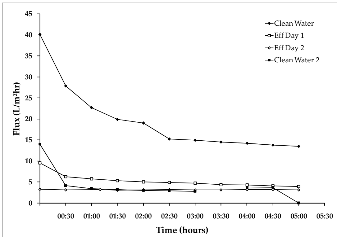
Figure A.8: Graph showing the flux from two clean water runs and the two 5 hour effluent runs on the membrane.
