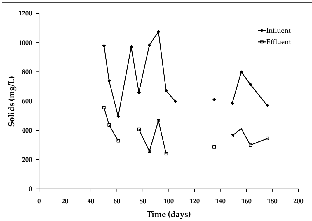
Figure 4.5: Total solids values of the influent and effluent for the period of the study.
