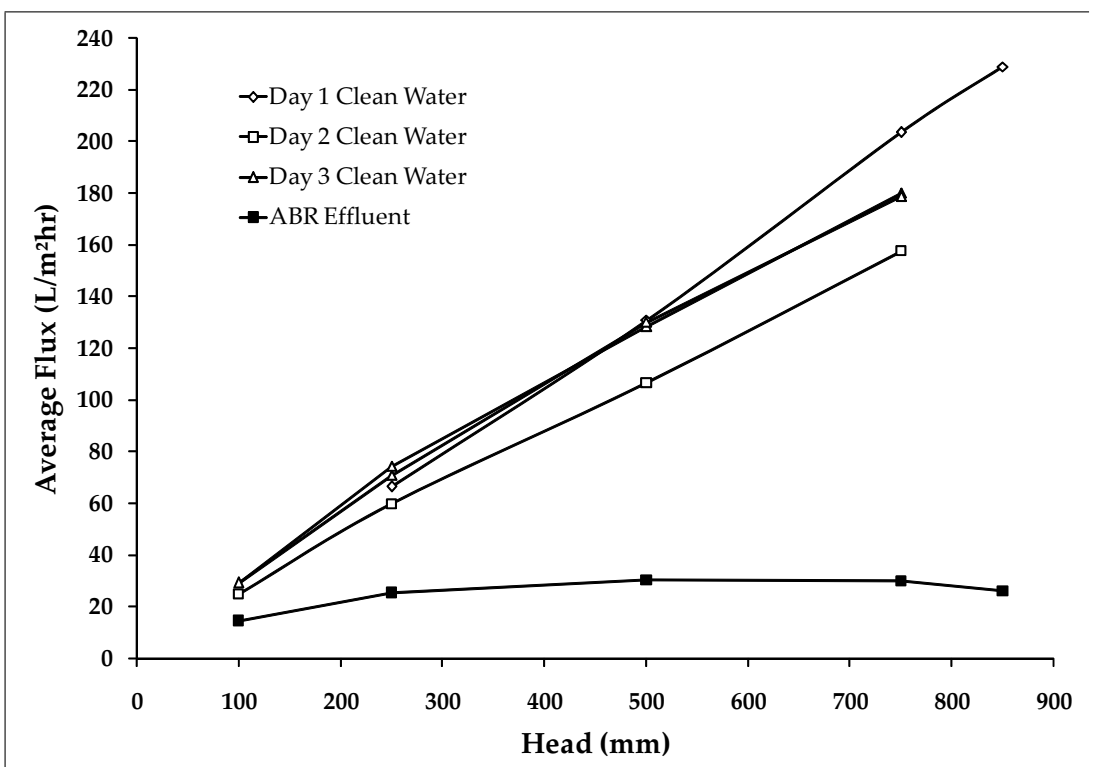
Figure A.6: Average flux from each run vs. head height.
