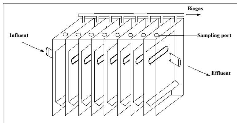
Figure 2.3: Schematic diagram of the ABR design for this project (Foxon et al., 2004).
