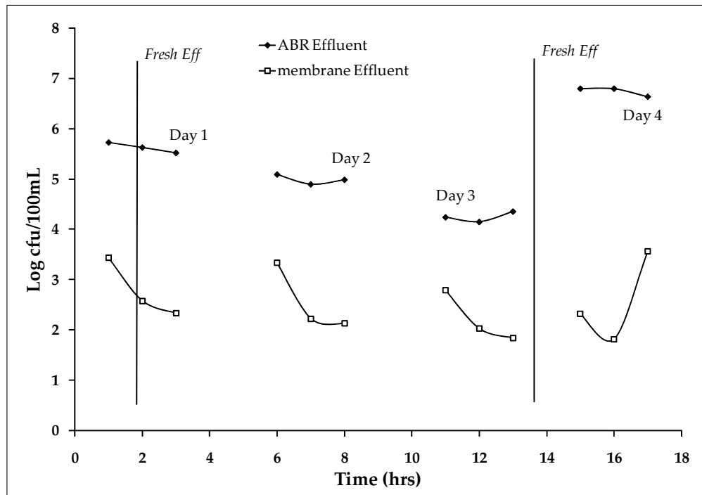
Figure A.12: Membrane removal of E. coli ; showing the log values of colony-forming units pre- and post- filtering through the membrane. The vertical lines show when fresh ABR effluent was collected.
