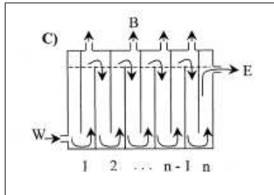
Figure 2.1: Original design for the anaerobic baffled reactor.
