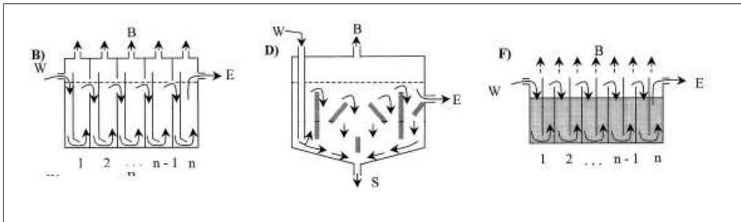
Figure 2.2: Modifications to the Anaerobic Baffled Reactor (Barber and Stuckey, 1999).
