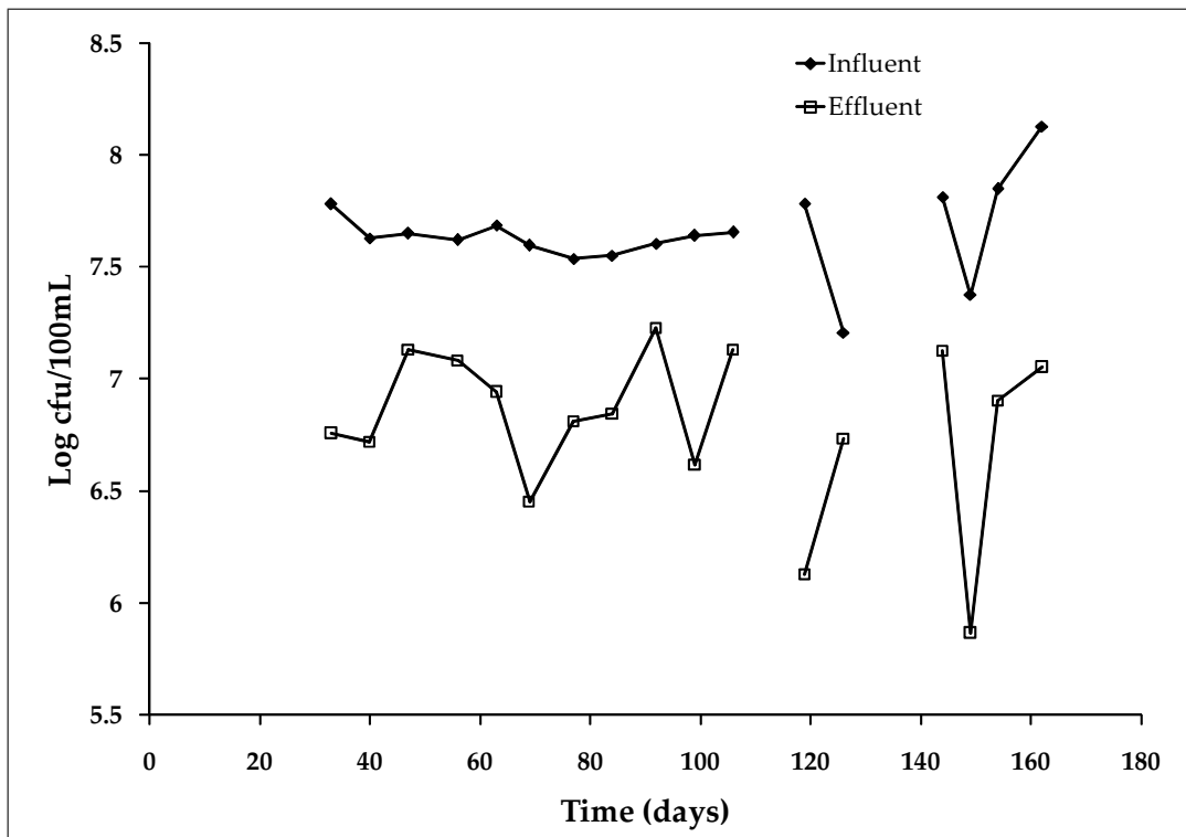
Figure 4.8: Graph showing the concentration of Faecal coliforms in the ABR influent and effluent.
