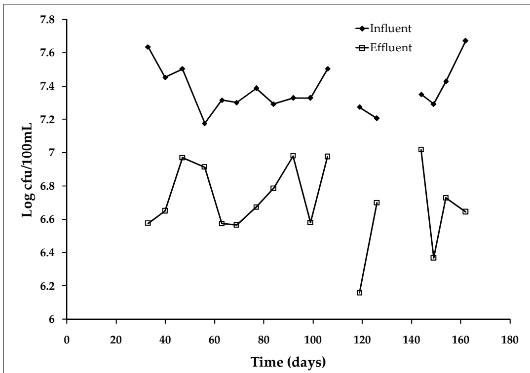
Figure 4.7: Graph showing the concentration of E.coli in the ABR influent and effluent.
