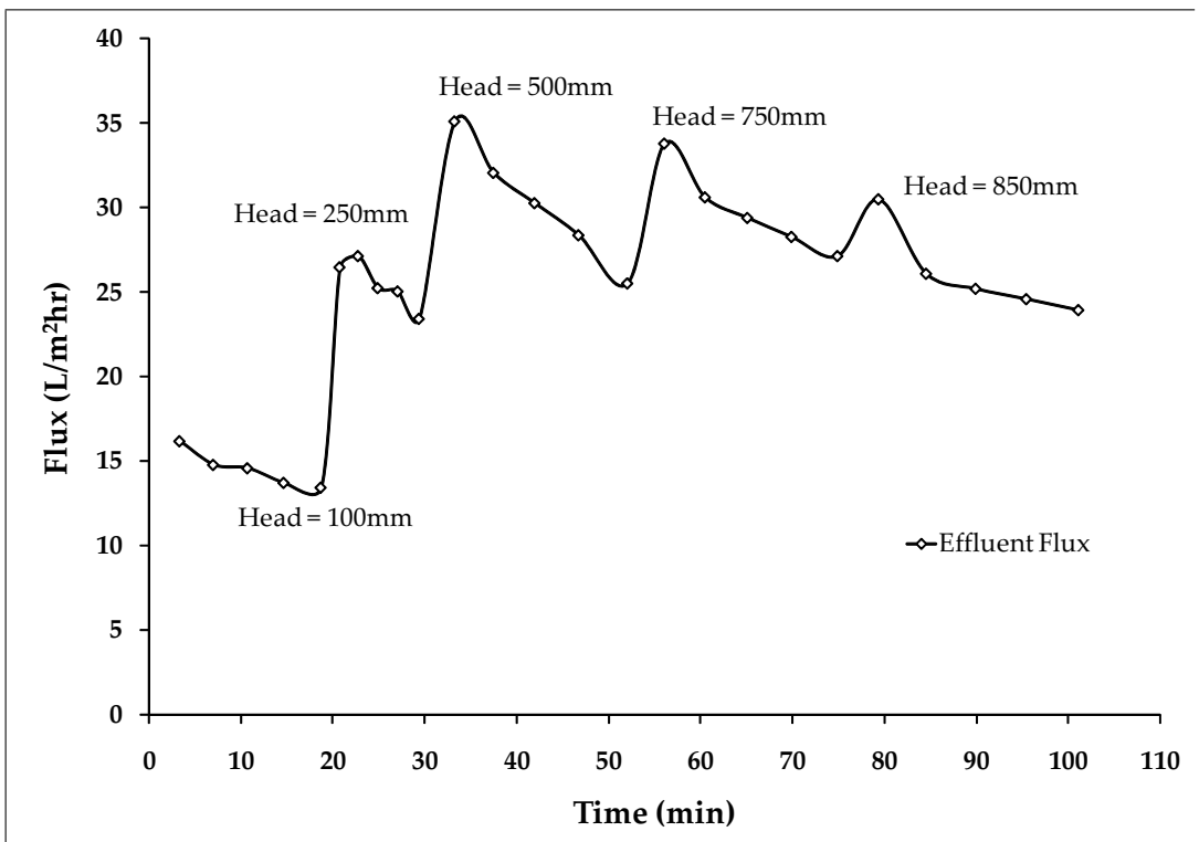
Figure A.5: Effluent flux at each head from 100 mm to 850 mm.
