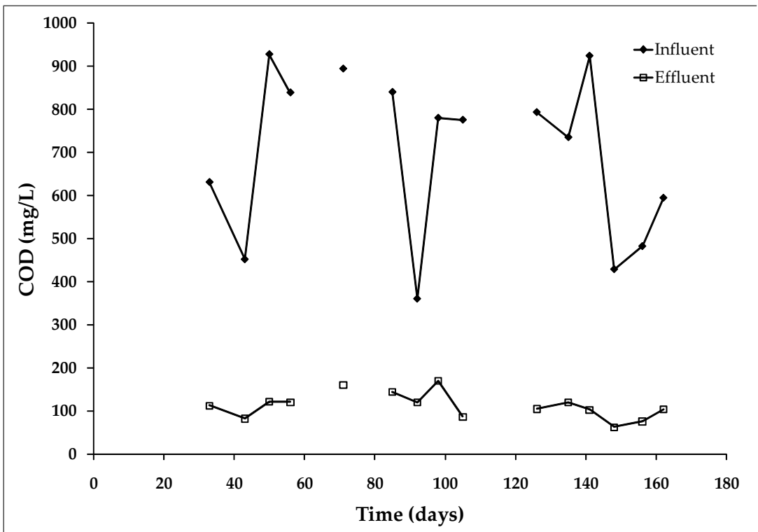
Figure 4.2: Total COD values for the period of operation.
