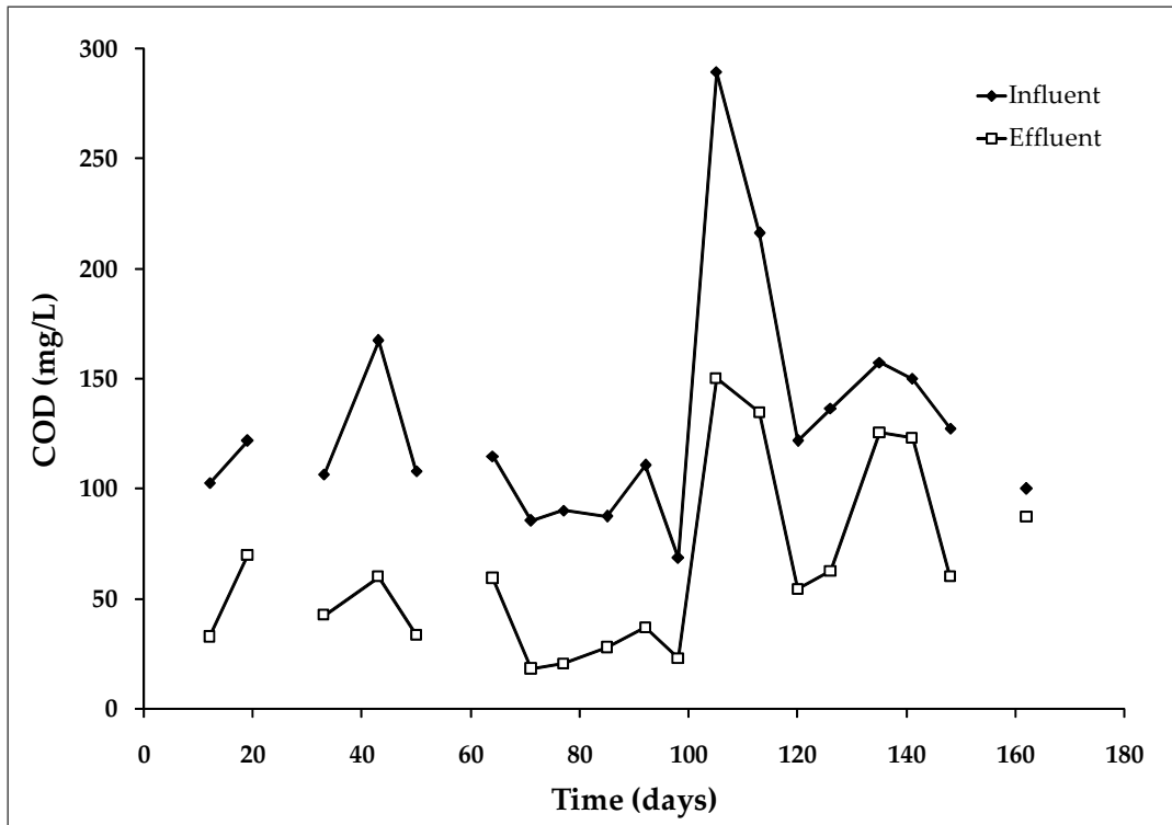
Figure 4.4: Soluble COD values of both the influent and effluent for the period of operation.
