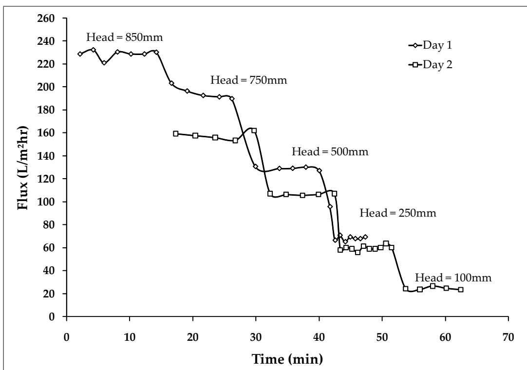
Figure A.3: Clean Water Flux tests performed in the laboratory using tap water.
