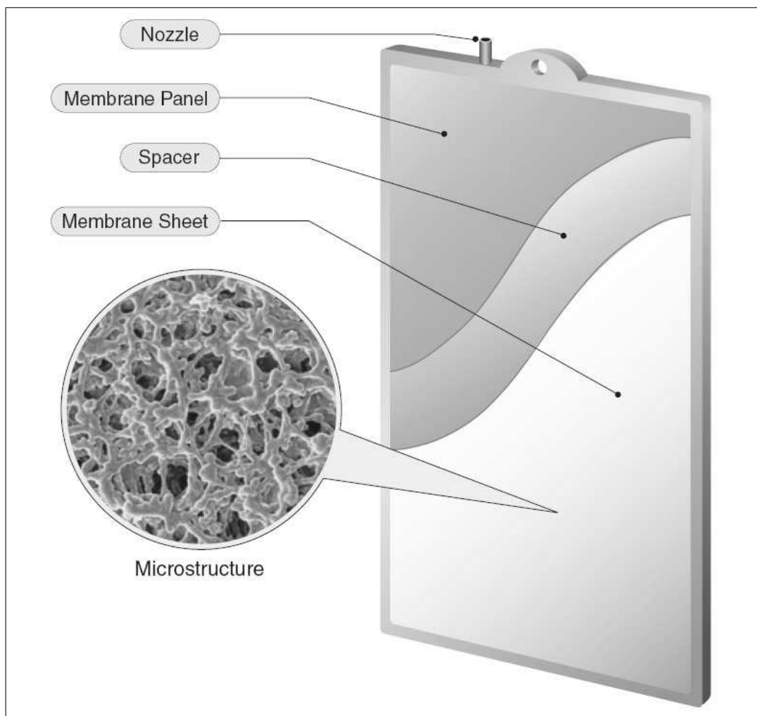
Figure A.1: The Kubota A4 membrane cartridge (Kubota Corporation, n.d.).
