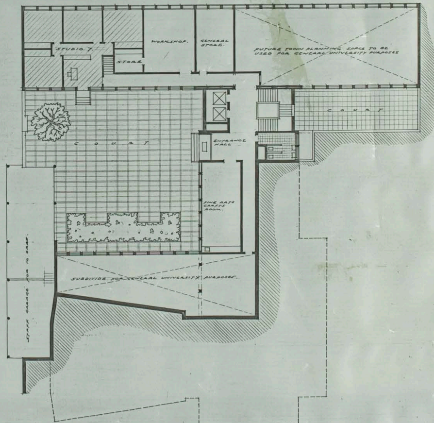
LOWER GROUND FLOOR PLAN
