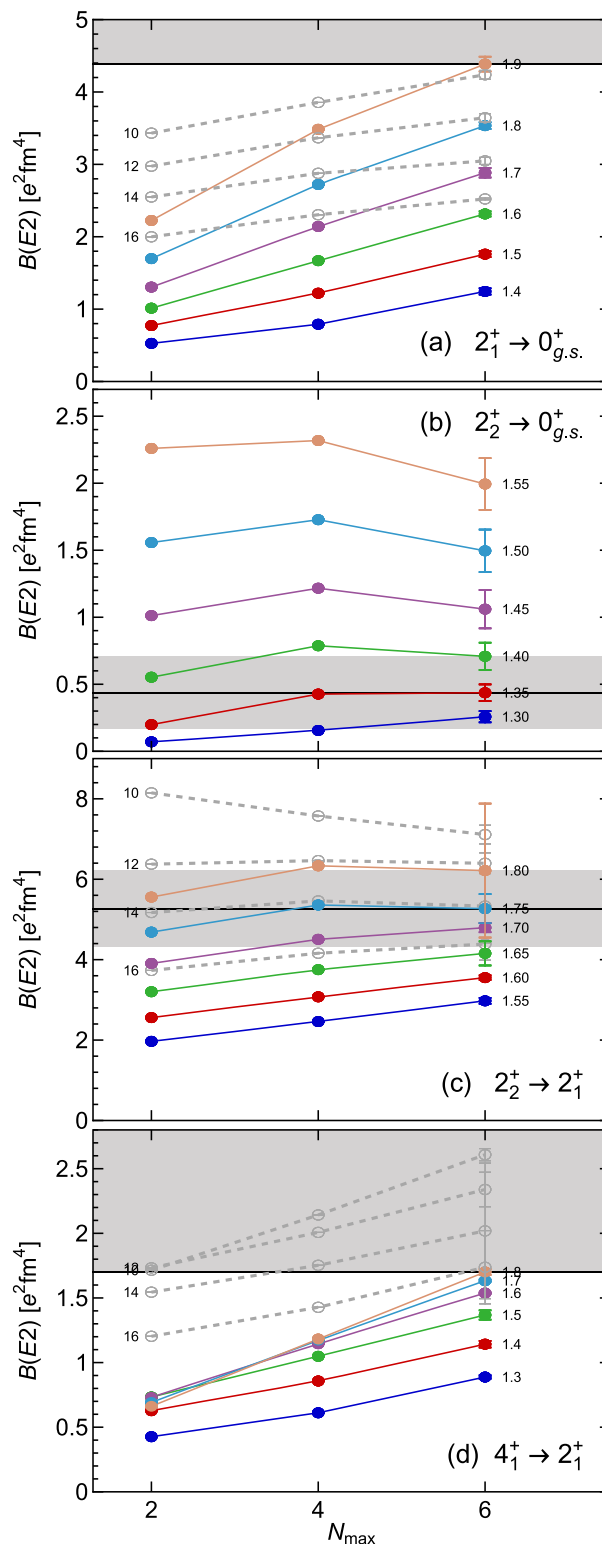
Fig. 11 Results of ab initio NCSM calculations for the B(E2) transition strengths involving the 0^+ ground state, the first two 2^+ excited states, and the first 4^+ excited state. The colored symbols show the N_{\text{max}} dependence obtained with the SNAT basis for different values of a_{\text{SNAT}} [fm] as indicated on the right-hand-side of each sequence. The grey symbols show N_{\text{max}} sequences obtained with the HO basis for different values of \hbar\Omega [MeV] as indicated on the left-hand-side of each sequence
