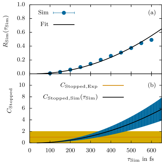
Fig. 7 a Ratio of counts between the moving and stopped peak component for the 2_2^+ \rightarrow 2_1^+ transition of ^{16}C for 110.18^\circ and results from the Geant4 simulations with Eq. 3 as a fit-function. b This fit-function scaled with C_{Moving,Exp} , which represents C_{Stopped,Sim}(\tau_{Sim}) . The blue band around the function shows its uncertainty including the uncertainty from C_{Moving,Exp} as well as the fit uncertainties. Also C_{Stopped,Exp} = 1(1) counts is plotted in orange for which the uncertainty is shown as a yellow band
