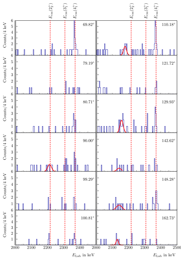
Fig. 4 Gamma-ray spectra in coincidence with the 2_1^+ \rightarrow 0_{g.s.}^+ transition for Gammasphere angles from 69.82^\circ to 162.73^\circ and a 2\sigma coincidence in Microball. The spectra for the discrete Gammasphere angles are obtained for a 2\sigma \gamma gate on the 2_1^+ \rightarrow 0_{g.s.}^+ transition with E_{cm} = 1760 keV and \sigma = 3.2 keV. The red dashed lines mark the expected center-of-mass energies for the 4_1^+ \rightarrow 2_1^+ ( E_{cm}(4_1^+) ), 3_1^+ \rightarrow 2_1^+ ( E_{cm}(3_1^+) ) and 2_2^+ \rightarrow 2_1^+ ( E_{cm}(2_2^+) ) transitions [6,8]. The red fit-functions are defined by a single Gaussian function using the binned-likelihood method recommended in case of low statistics
