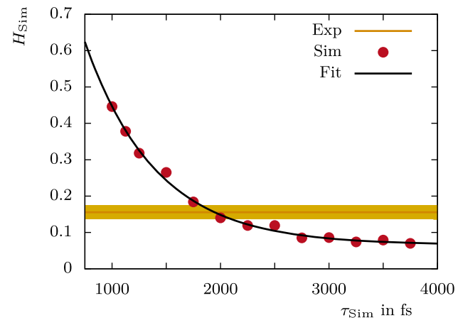
Fig. 9 Estimation of a lower lifetime limit for the 4_1^+ state of ^{16}\text{C} using the 148.28^\circ Gammasphere spectrum. Geant4 simulation results for H_{\text{Sim}}(\tau_{\text{Sim}}) have been performed using SRIM stopping powers and \bar{\beta}_{\text{TO}} = 0.04527(44) . The black fit-function is described by Eq. 7. The yellow band illustrates the experimental ratio of H_{\text{Exp}} = 0.156(19) including its uncertainty
