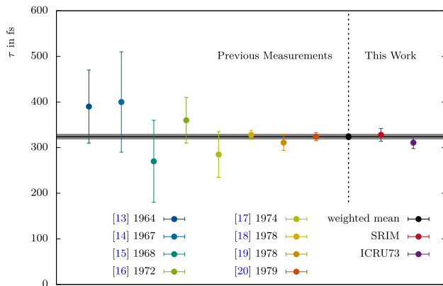
Fig. 3 Temporal development of the measured lifetimes for the 4_1^+ state in ^{22}\text{Ne} . The eight values from the previous measurements are taken from [13–20] respectively. They lead to the uncertainty weighted mean of 324(6)fs [21], which is shown as a black point and as a grey uncertainty band. The results from this work, illustrated by the red (SRIM stopping powers) and purple (ICRU73 stopping powers) data points, are in excellent agreement with the previous measurements
