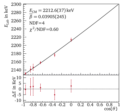
Fig. 5 E_{\text{Lab}} versus \cos(\theta) fit for the 2_2^+ \rightarrow 2_1^+ transition of ^{16}\text{C} . The E_{\text{Lab}} values are extracted from the Gaussian fits shown in Fig. 4. The black fit-function is described by Eq. 1. The lower plot shows the residuals \Delta E of the fit which is shown in the upper part
