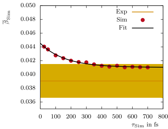
Fig. 6 Simulated mean decay beta \bar{\beta}_{Sim} versus simulated lifetime \tau_{Sim} for the 2_2^+ \rightarrow 2_1^+ transition of ^{16}C . The initial beta in the simulation was obtained with \bar{\beta}_{TO} = 0.04527(44) . The yellow band illustrates the experimental mean decay beta value of \bar{\beta}_{Exp} = 0.03905(245) including its uncertainty
