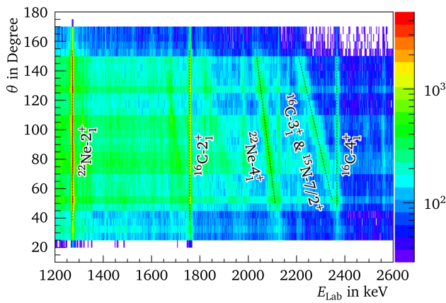
Fig. 2 Radiation-detection angle \theta versus laboratory energy E_{\text{Lab}} for 2p Microball-gated \gamma -ray events for the target/degrader setting. Dominant \gamma rays from other fusion-evaporation reactions, as well as those from the reaction channel of interest are indicated with a dotted line, the corresponding isotope and the initial state of the \gamma -ray transition is given. Other transitions visible but not marked on the plot correspond to the ^{23}\text{Ne } 7/2^+ \rightarrow 5/2^+ 1701 keV transition and to the ^{15}\text{N } 5/2_2^+ \rightarrow 5/2_1^+ 1884 keV transition
