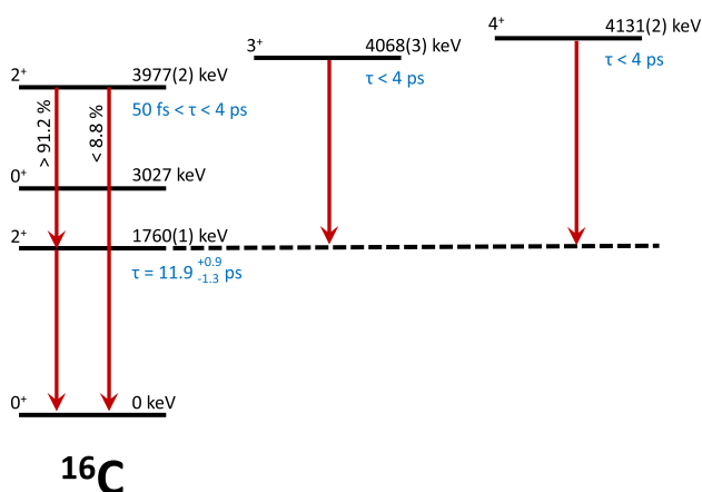
Fig. 1 Spectroscopic information on the bound excited states of ^{16}\text{C} ; lifetime information are extracted from Refs. [6–9]
