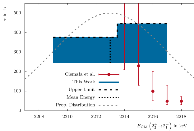
Fig. 8 Results for the lifetime range of the 2_2^+ state in ^{16}\text{C} using the count ratio method and SRIM stopping powers. The values from this work are shown as black dashed lines and blue boxes. The horizontal black dashed lines mark the upper lifetime limit while the vertical black dashed line marks the mean \gamma -ray energy for the 2_2^+ \rightarrow 2_1^+ transition as measured in this work. The blue boxes mark the most likely lifetime range. The external values shown as red dots are the most recent measurements from Ciemała et al. [7]. The grey dashed function shows the relative probability distribution as a function of the transition energy for our results. It follows a Gaussian distribution with a mean of 2213 keV and a sigma of 4 keV
