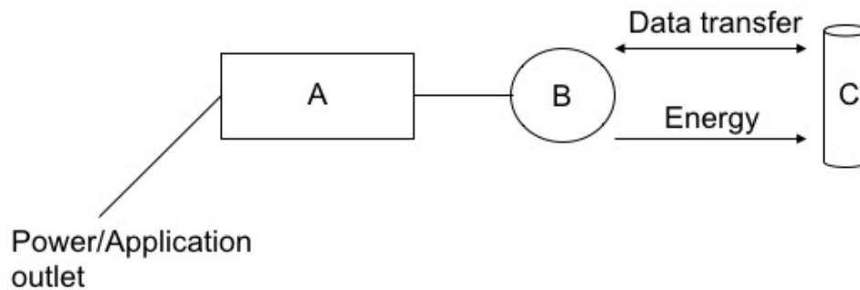
Figure 2.1: The main components of an RFID system are the reader (A), with an attached antenna (B) and the tag (C).
