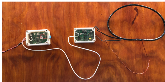
Figure 2.4: The Automated Cellular Reader System (ACRS) showing the housing of the cellphone engine (left), reader board (right) and the attached antenna.
