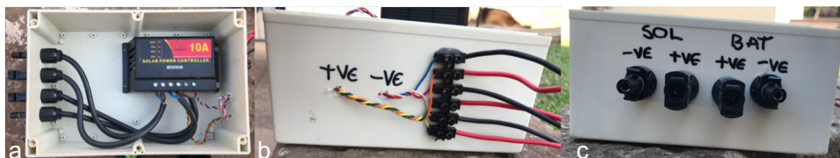
Figure 2.2: The connection box showing the solar controller (a), the connections for multiple ACRSs (b) and connections for the solar panel and battery (c).
