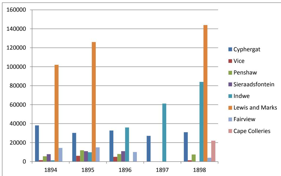
Figure 8. Coal output in tons of the various Stormberg companies, Indwe and Lewis and Marks, 1894-1898
