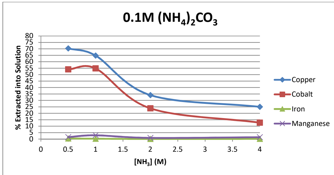
[(NH 4 ) 2 SO 3 ]: 0.4M; 80°C; 300rpm; -75+63μm; Pre-Treatment Time: 1hour; Leach Time: 1hour; Figure 4.6(a): The Effect of Changing Ammonia Solution Concentration at Fixed 0.1M Ammonium Carbonate
