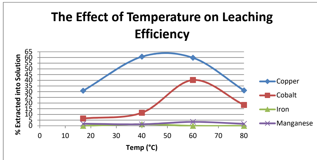
[NH 3 ]: 4.0M; [(NH 4 ) 2 CO 3 ]: 0.4M; [(NH 4 ) 2 SO 3 ]: 0.4M;; 300rpm; 90mins Fig 4.2: The Effect of Temperature on Leaching
