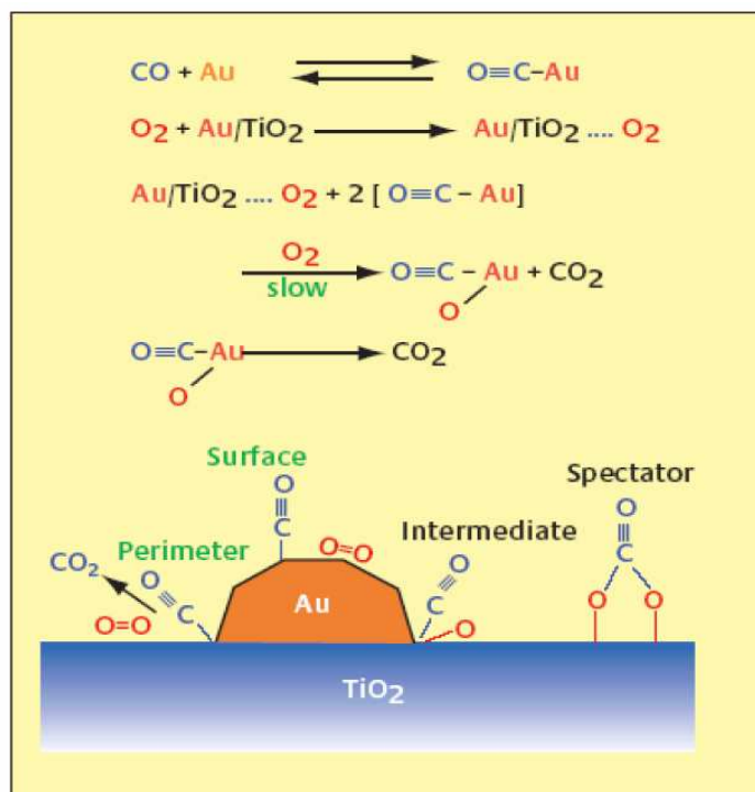
Figure 1.5 CO oxidation reaction pathways of the Au on TiO 2 catalyst suggested by Haruta et al. [2-3]
