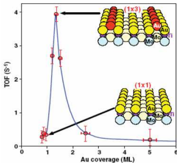
Figure 1.8 Activity for CO oxidation at room temperature as a function of Au coverage above the monolayer \text{TiO}_x on Mo(112) [43]
