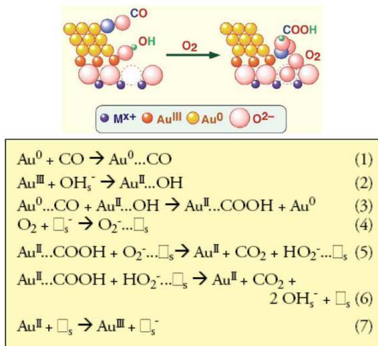
Figure 1.6 A representation of the oxidation of carbon monoxide at the periphery of an active gold particle on metal oxide support [48]
