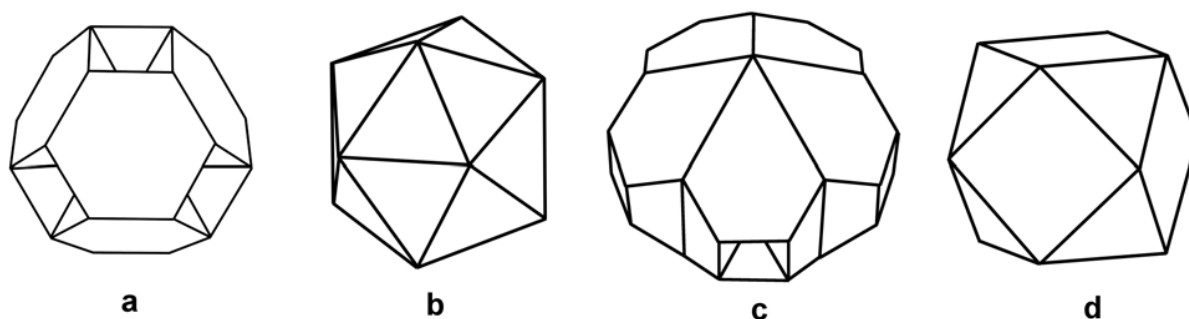
Figure 1.1. Comparison of (a) truncated octahedron, (b) icosahedron, (c) Marks decahedron and (d) cuboctahedron. Note the re-entrant facets in the truncated octahedron and the Marks decahedron. (a) and (c) redrawn from Doye [49], b and d redrawn from Mackay [16].
