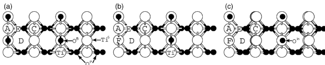
Figure 1.4. Schematic geometry (top view) of TiO 2 (110) surfaces. Five possible adsorption sites are marked from A to E for the stoichiometric surface (a) and six possible adsorption sites are marked from A to F for the Ti-rich (b) and O-rich (c) surfaces. The small filled circles and the large open circles indicate the oxygen and titanium atoms, respectively [38].
