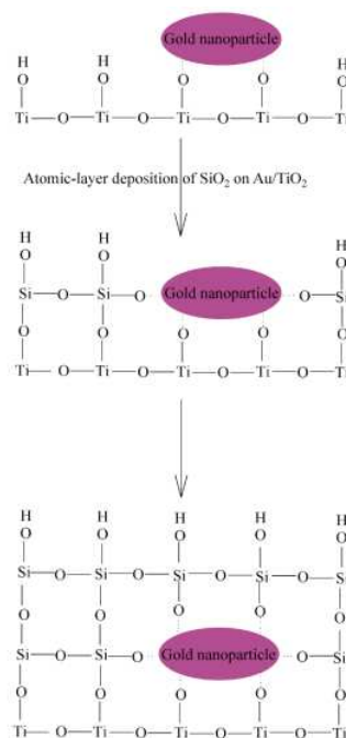
Figure 1.13 Schematic representation of the ALD of amorphous SiO 2 onto Au/TiO 2 [82]
