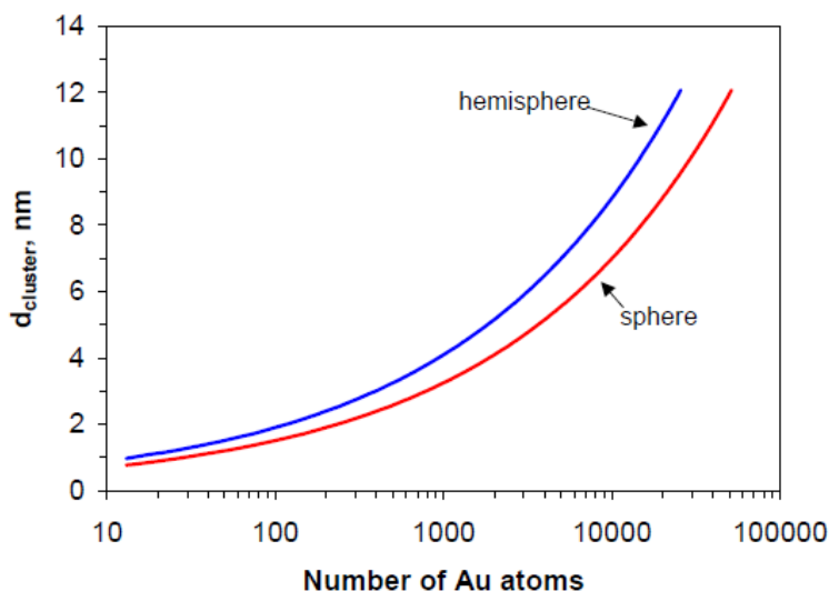
Figure 1.2. Approximate size of nominally spherical and hemispherical clusters of Au_n [25].
