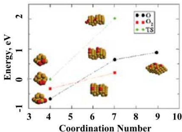
Figure 1.7 Binding energy of different oxygen species, versus gas-phase O 2 , plotted with respect to the coordination number of the Au atoms of the site. Yellow spheres (Au), red (O), and gray (C) [54]
