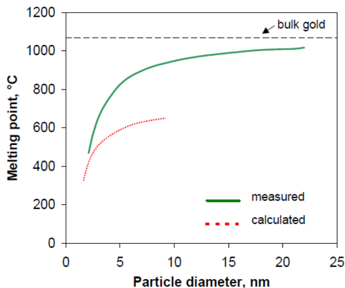
Figure 1.3. Reduction of melting point with a decrease in size of gold nano-particles, showing both theoretical data computed using molecular dynamics [10] and measured data derived from gold nanoparticles encapsulated in silica [38].
