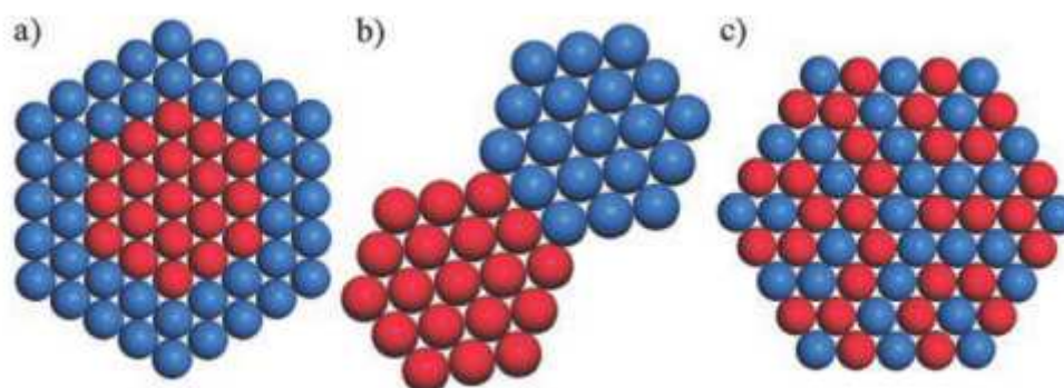
Figure 1.14. Bimetallic Nano Crystals with different structures: a) core/shell; b) heterostructure; c) intermetallic or alloyed structures [178].
