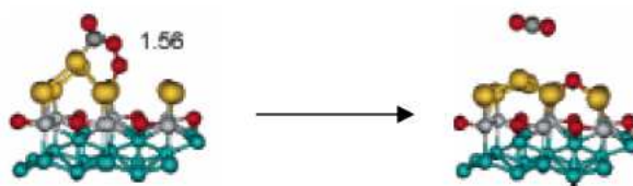
Figure 1.9 Structure of the peroxo-type CO-O 2 complex (left) and final state (right) for CO oxidation on the 4/3 layer Au/TiO-Mo(112) surface [86]
