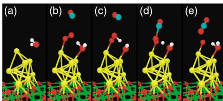
Figure 1.11 Atomic configurations displaying several stages in the simulation of the coadsorption of H 2 O and O 2 on the top facet of a Au 8 cluster supported on MgO(100), and the subsequent reaction with gaseous CO to form CO 2 . Yellow (Au), red (O), white (H), green (Mg), and aquamarine (C) [98].
