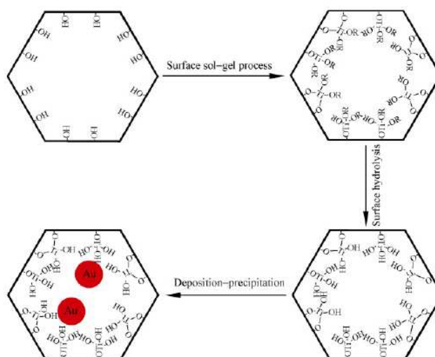
Figure 1.12 The modification of mesoporous \text{SiO}_2 by \text{TiO}_2 using a surface-sol-gel approach for loading gold nanoparticles. [116]
