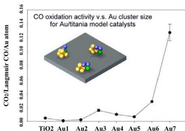
Figure 1.10 Size dependence of CO oxidation activity [90]
