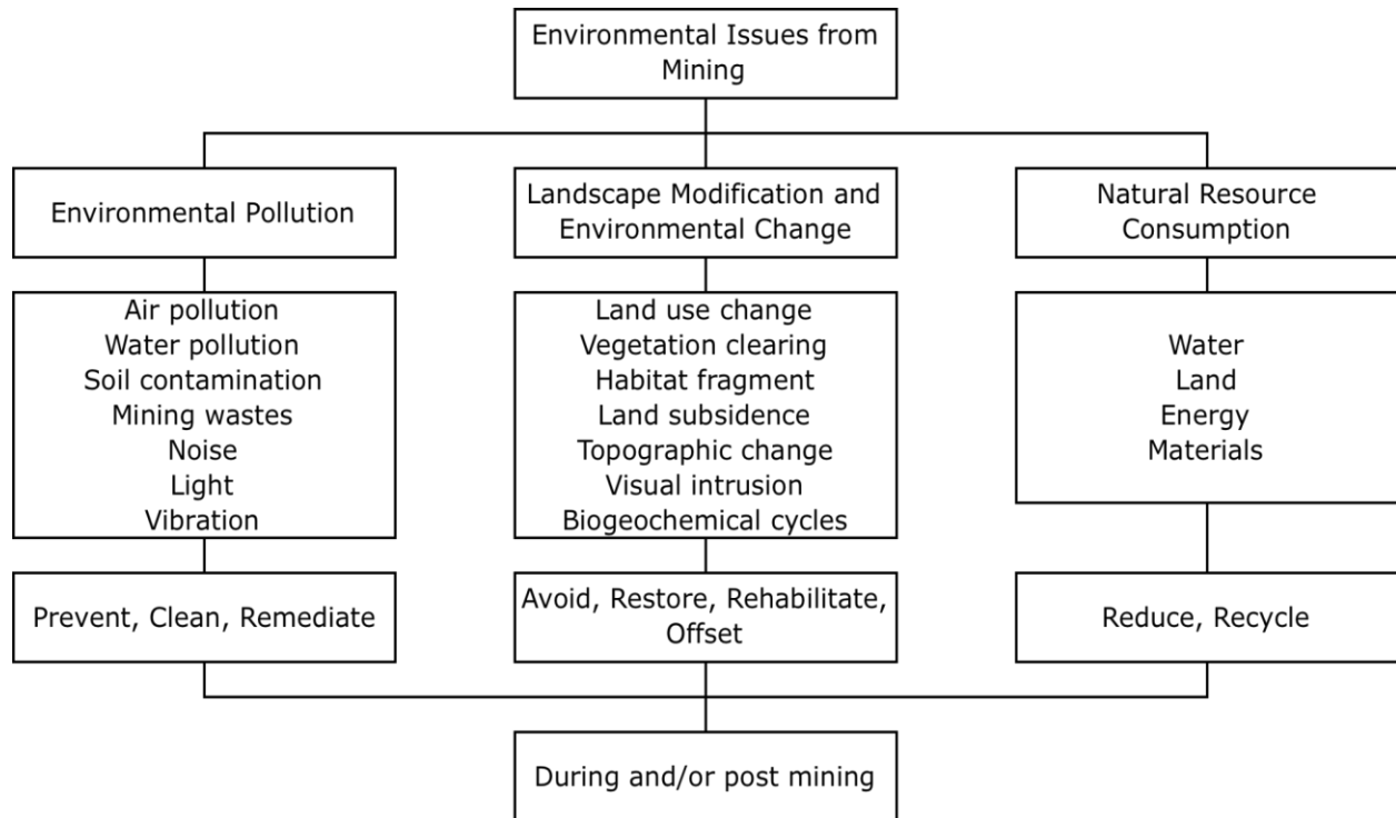
Figure 3: Environmental Issues from Mining (Adapted from Bian, Inyang, Daniels, Otto and Struthers, 2010).
