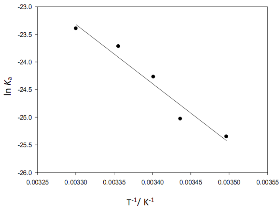
Figure 5.10 van't Hoff plot for the ionisation of coordinated H 2 O in [AC-(10-NH 2 )Cbs] + .
