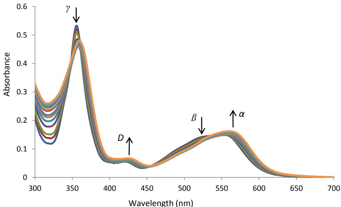
Figure 3.10 The absorbance changes observed for the binding of \text{N}_3^- to [\text{H}_2\text{O}-(10\text{-Br})\text{Cbl}]^+ .
