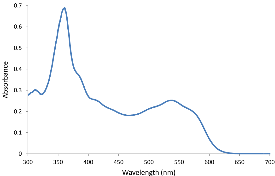
Figure 2.4 The uv-vis spectrum of [DC-(10-NO 2 )Cbs].
