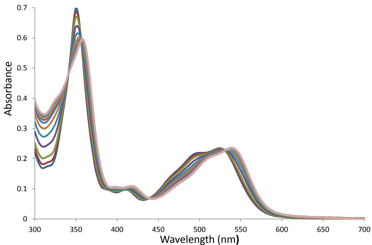
Figure 3.1.8 The absorbance changes observed for the binding of \text{N}_3^- to [\text{H}_2\text{OCbl}]^+ .
