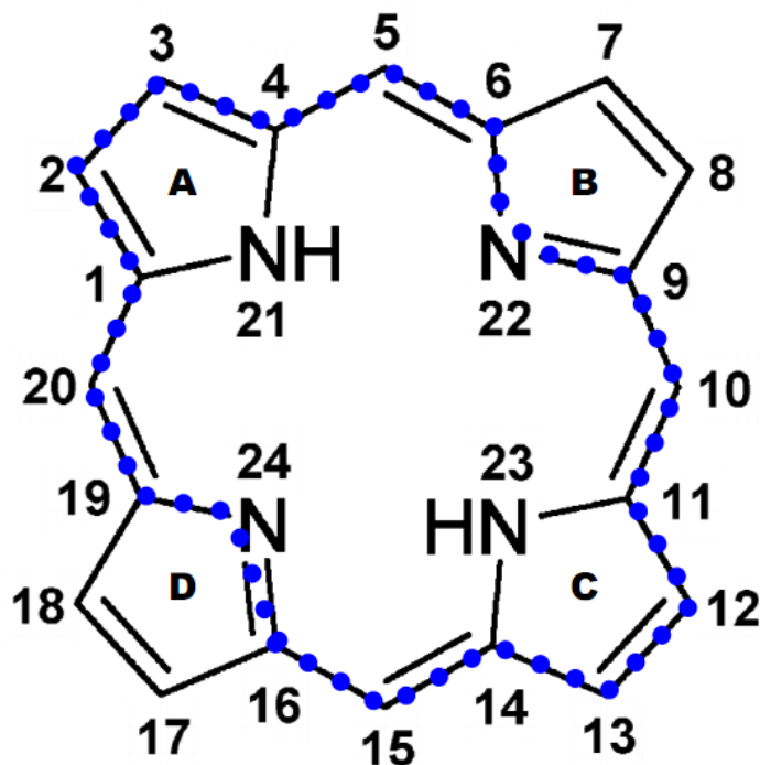
Figure 1.5 The backbone of all porphyrins. The indicated blue pathway shows the delocalised 18- \pi electron system. This structure was proposed by Küster in 1912. However, Hans Fischer is often credited with identifying this structure in 1929. 76,77
