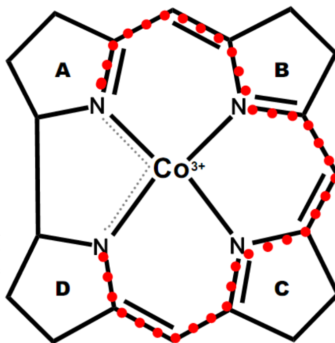
Figure 1.4 The cobalt corrin structure, red dots indicate the delocalised \pi electron system. 45
