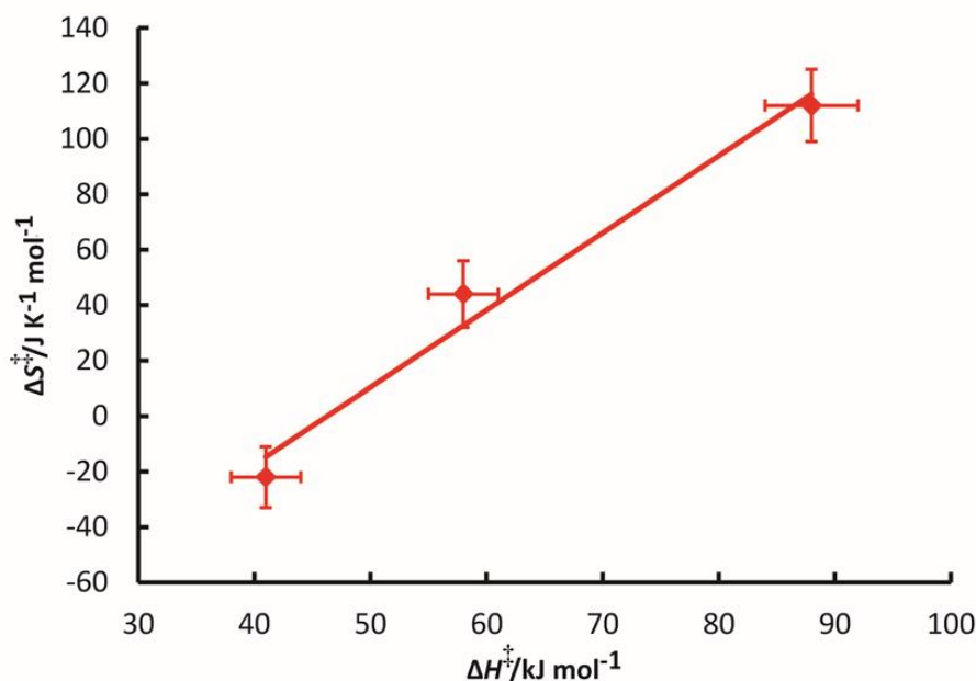
Figure 6.3 There is a compensation effect between values of \Delta H^\ddagger and \Delta S^\ddagger for the ligand substitution of coordinated \text{H}_2\text{O} in [\text{AC}-(10\text{-Z})\text{Cbs}]^+ ( \text{Z} = \text{H}, \text{NH}_2, \text{NO}_2 ).
