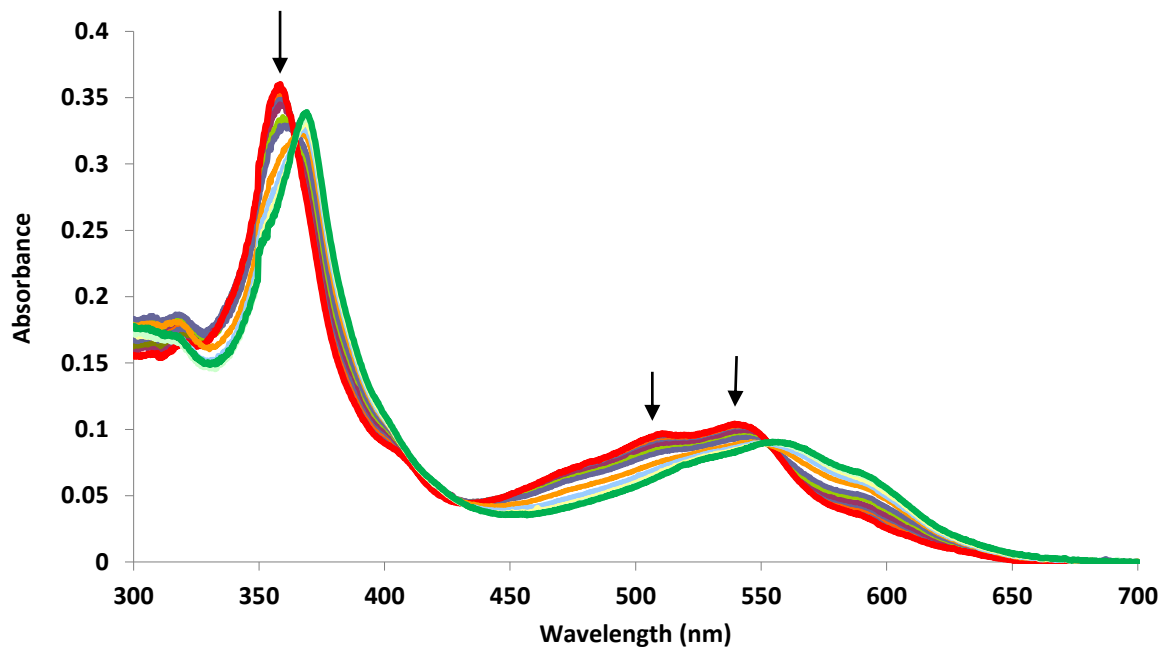
Figure 5.8 The effect of pH on the uv-vis spectrum of [AC-(10-NH_2)Cbs]^+ , varying pH from 6.2 (red) to 12.6 (green).
