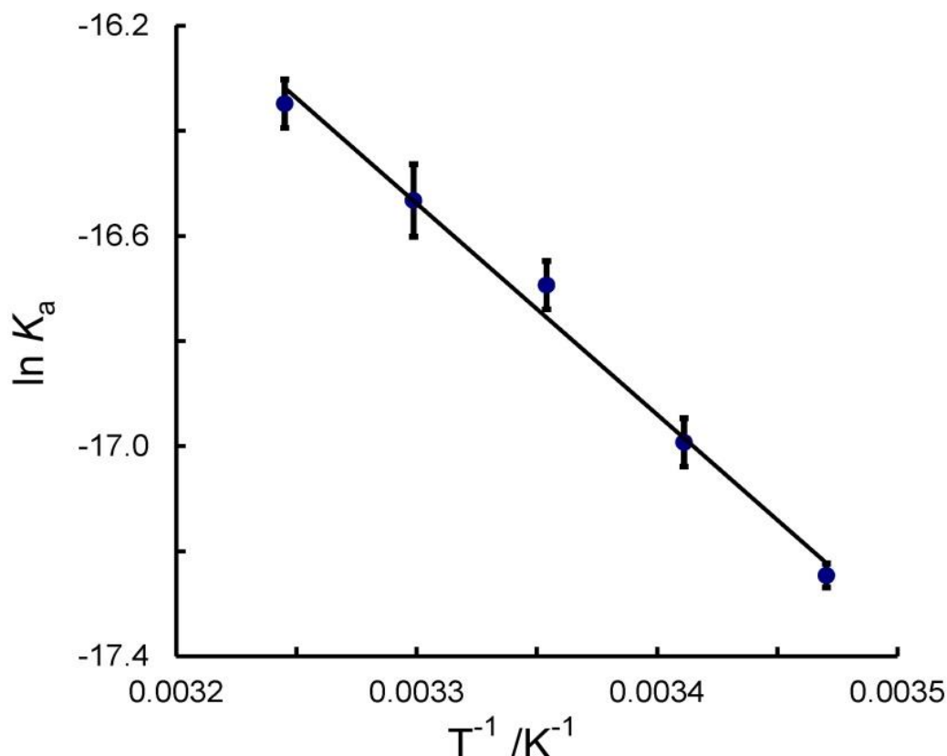
Figure 3.7 van't Hoff plot for the ionisation of coordinated H_2O in [H_2O-(10-Br)Cbl]^+ . From the slope and intercept \Delta H = 34 \pm 2 \text{ kJ mol}^{-1} and \Delta S = -26 \pm 6 \text{ J K}^{-1} \text{ mol}^{-1} were determined, respectively.
