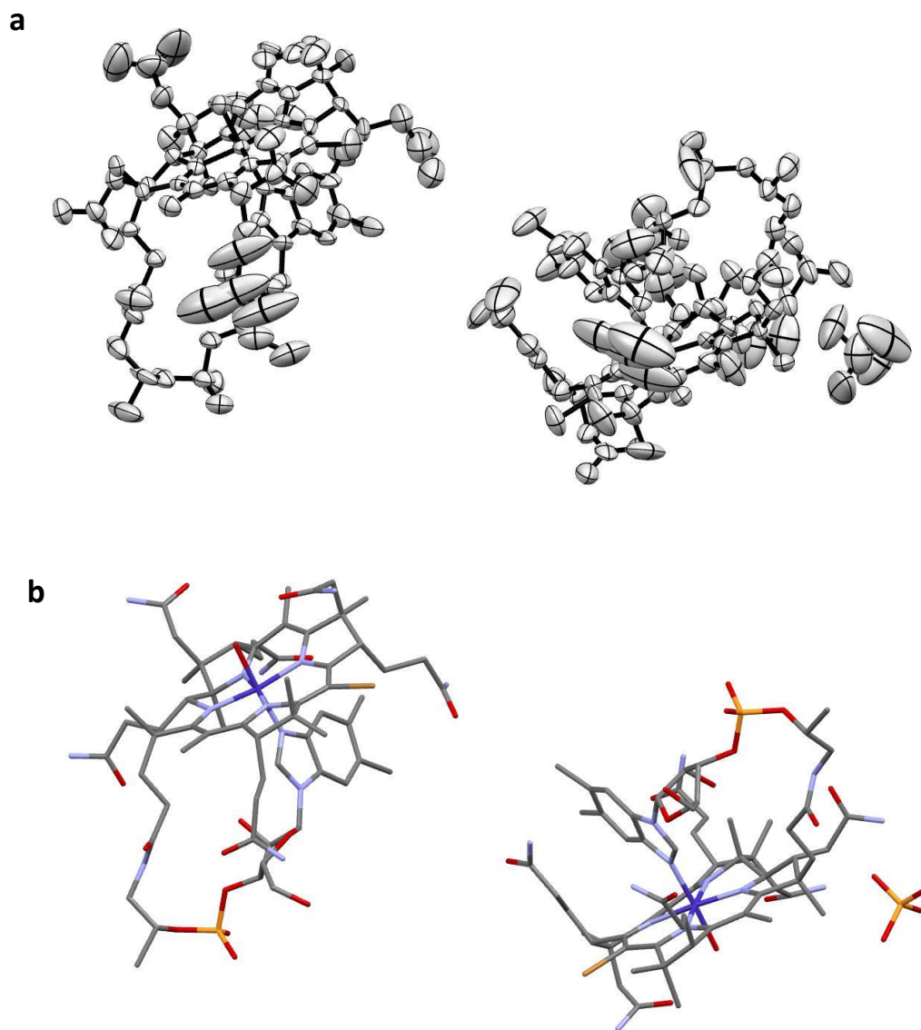
Figure 2.10 Crystal structure of [\text{H}_2\text{O}-(10\text{-Br})\text{Cbl}]^+ , (a) ORTEP diagrams with the ellipsoids drawn at the 50% contour level, (b) capped sticks diagram.
