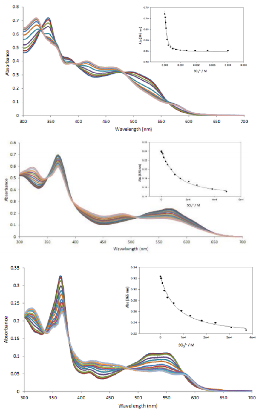
Figure 5.15 Changes in the uv-vis spectrum on substituting coordinated \text{N}_3^- in (top) [\text{N}_3\text{CN}-(10\text{-NO}_2)\text{Cbs}] , (middle) [\text{N}_3\text{CN}-(10\text{-NH}_2)\text{Cbs}] and (bottom) [\text{N}_3\text{CNCbs}] by \text{SO}_3^{2-} at 25 °C, pH 8.9. The insert shows a fit of the absorbance change at 346, 570 and 365 nm, (from top to bottom) to the binding isotherm given by Equation 2.4 .
