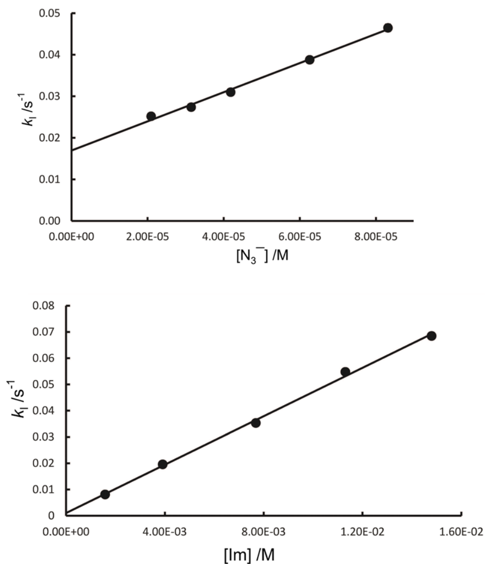
Figure 4.2 Plots of k_I against (top) [\text{N}_3^-] (25.0 °C) and (bottom) imidazole (20.0 °C). The intercept in the first case is significant statistically different from zero, but not in the second case. The gradients give the second order-rate constant, k_{II} .
