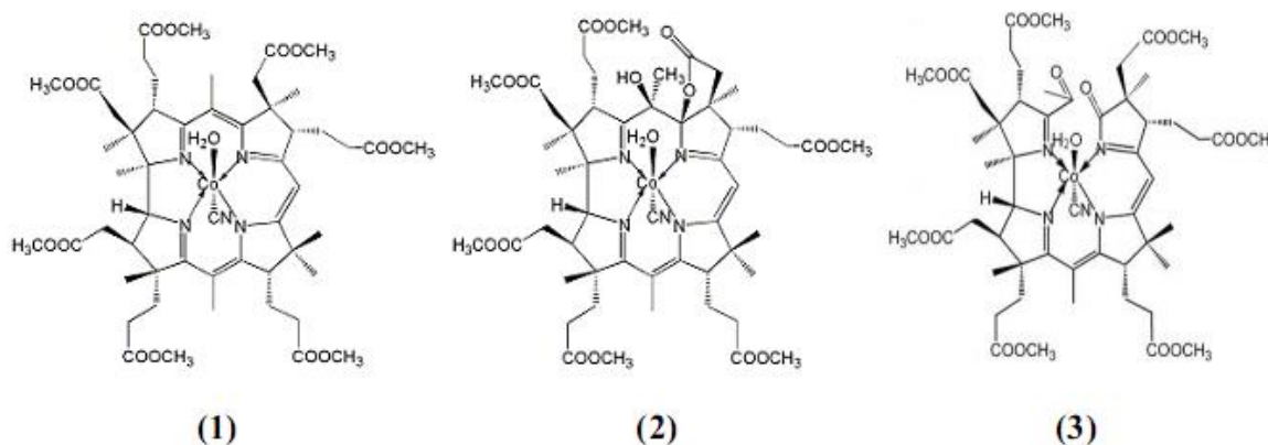
Figure 5.1 The structures of [\text{ACCbs}]^+ (1), [\text{ACSYCbs}]^+ (2) and [\text{5-seco-ACCbs}] (3). 8
