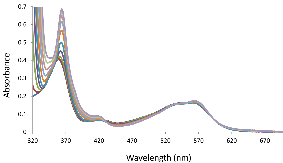
Figure 3.1.7 The absorbance changes observed for the binding of DMAP to [\text{H}_2\text{O}-(10\text{-Cl})\text{Cbl}]^+ .
