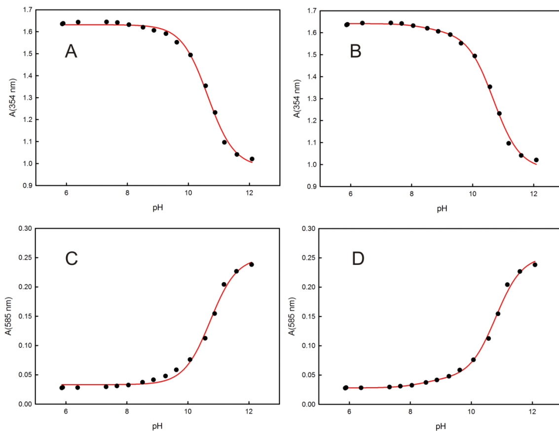
Figure 5.3 Plots of the change in absorbance of [ACCBs] + in 50% isopropanol/buffer solutions at 25 °C, (A) at 354 nm fitted to a single pK a model, (B) at 354 nm fitted to a two pK a model (C) at 585 nm fitted to a single pK a model, (D) at 585 nm fitted to a two pK a model.
