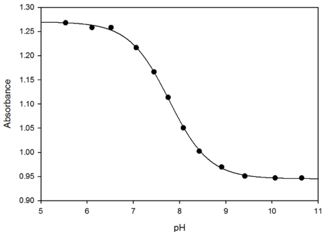
Figure 3.2 A plot of the change in absorbance of [\text{H}_2\text{OCbl}]^+ at 352 nm to which Equation 2.1 has been fitted.
