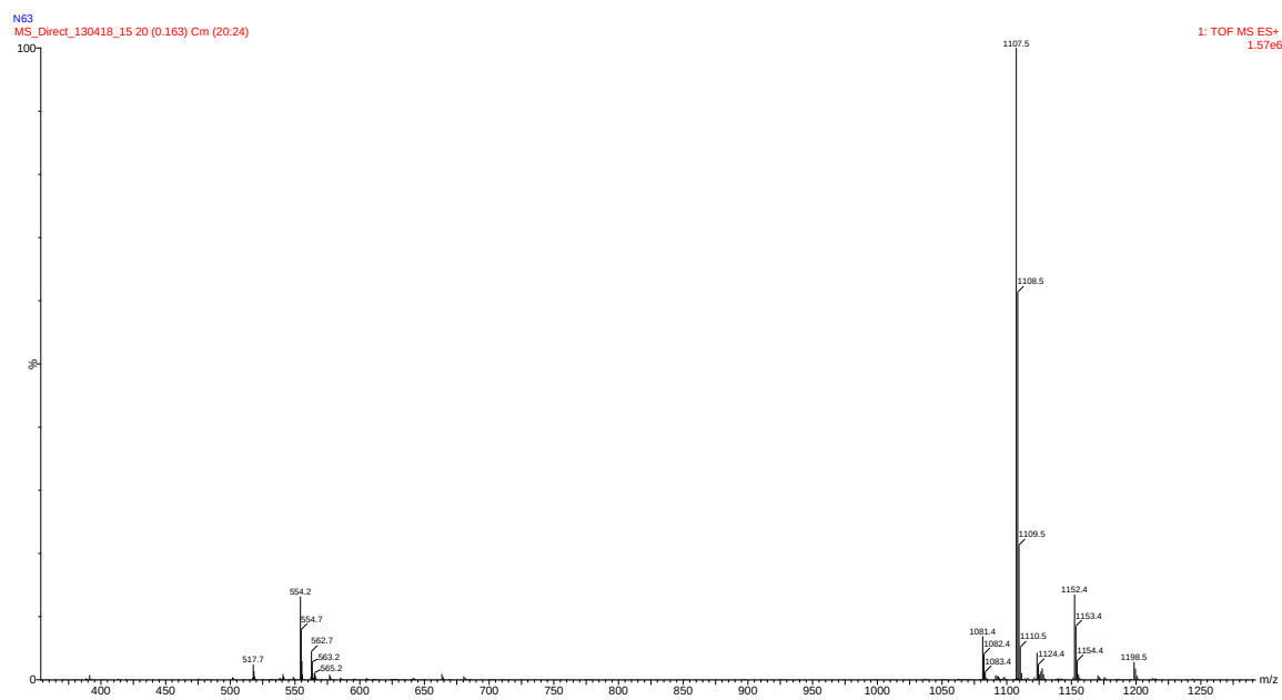
Figure 2.3.3 The positive ESI-MS of [DC-(10-NO 2 )Cbs] indicating the loss of the water axial ligand (1107).
