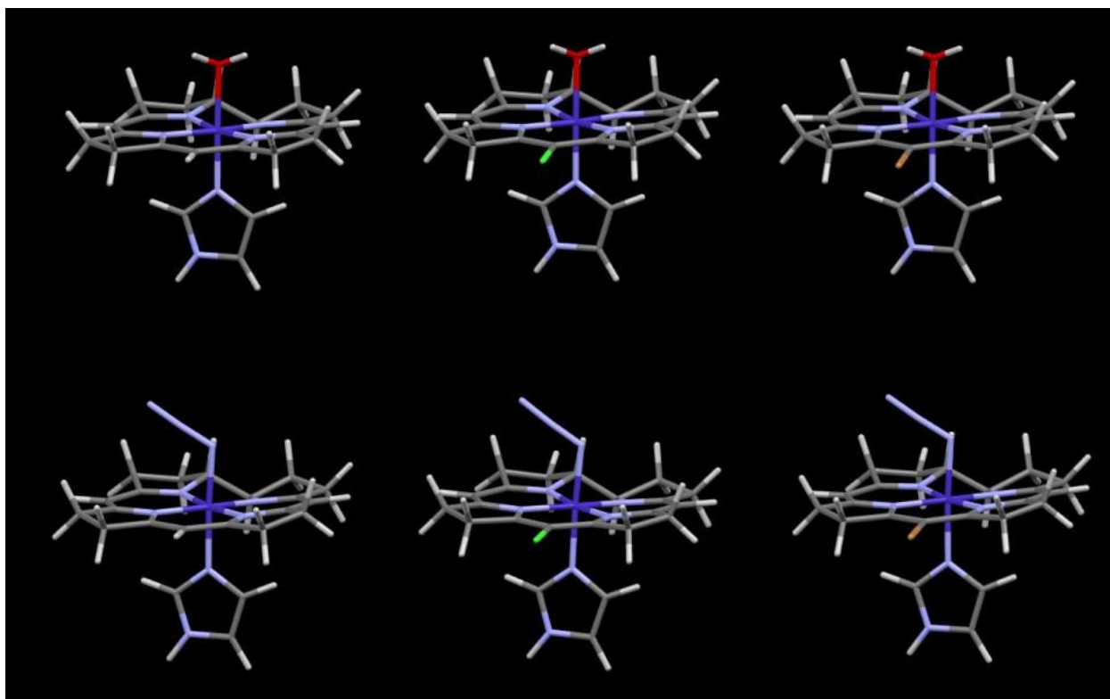
Figure 3.18 Energy-minimised DFT models of (top) [\text{H}_2\text{O}-(10\text{-Z})\text{Cbl}]^+ with (left to right) \text{Z} = \text{H} , \text{Cl} , \text{Br} ; and (bottom) [\text{N}_3-(10\text{-Z})\text{Cbl}] with (left to right) \text{Z} = \text{H} , \text{Cl} , \text{Br} .
