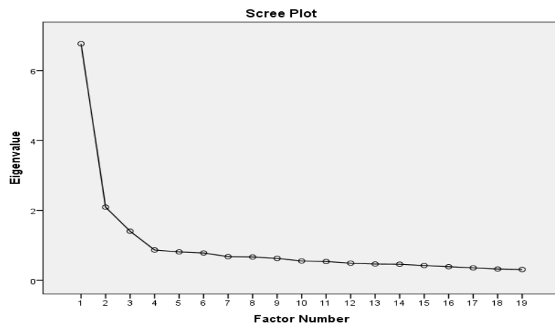
Figure 4.8: Scree Plot
