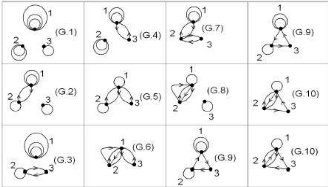
Figure 8.2: The open string configurations consistent with the Gauss Law for a three giant system with \Delta weight \Delta = (3, 2, 1) . The figure labels match the corresponding equation.
