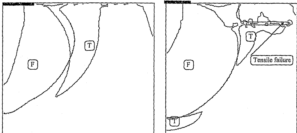
a) Contours of plastic failure (F) and tensile minor principal stresses (T) at an initial stage of loading
