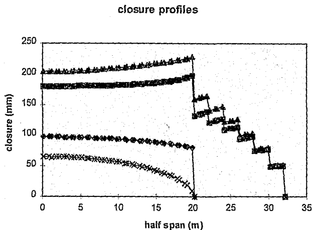
Figure 6.21 Vertical deformations at the skin of a stope for different scenarios: -elastic, after 1 mining step (half span of 20m) -vertical discontinuity introduced, after 1 mining step -vertical discontinuities introduced, after 6 additional mining steps -same plus simulation of additional tensile fractures
