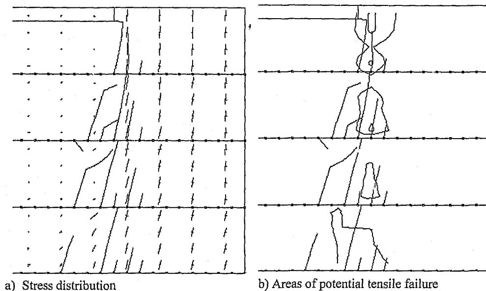
Figure 6.12 Effect of induced fracture coalescence. The narrow zone between those fractures, which completely split individual layers, is allowed to “crush”
