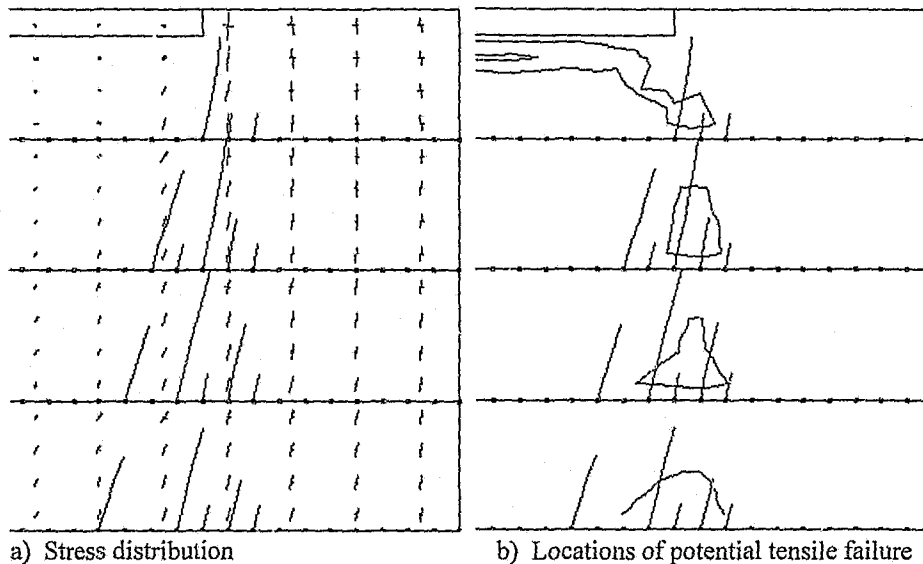
Figure 6.11 (tensile) Fracture formation due to the stress field induced by a stope in a layered medium as in the previous example
