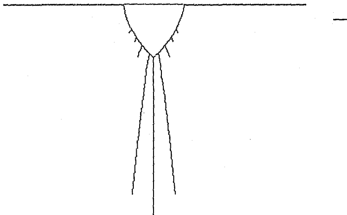
Figure 6.15 DIGS simulation of punch failure in an elastic material
