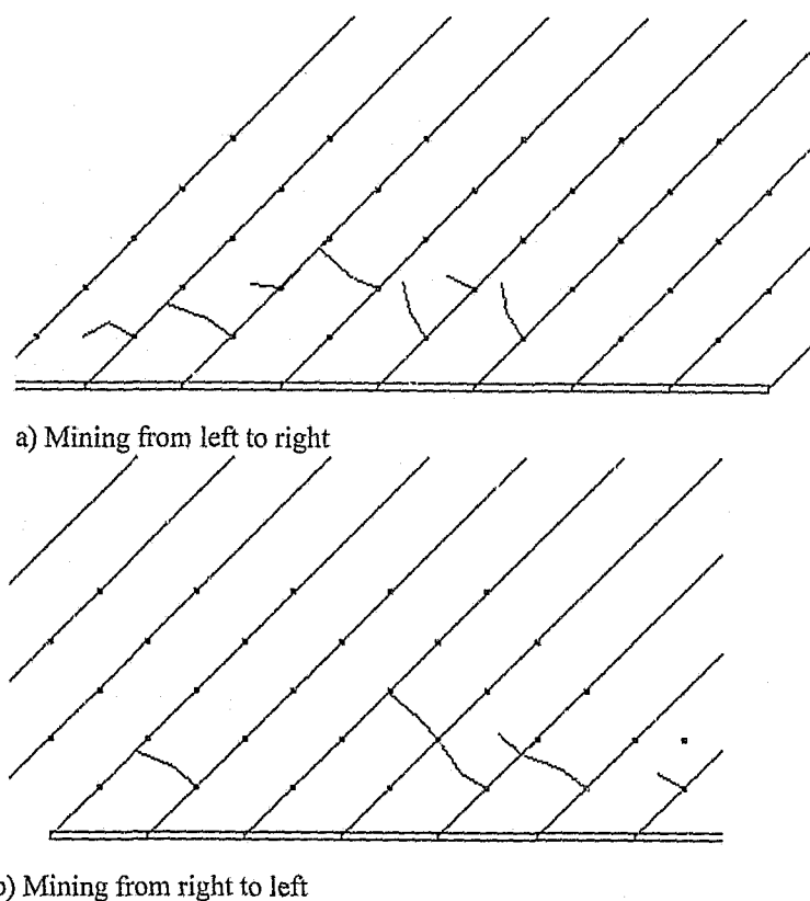
Figure 6.13 Effect of a joint set on mining induced (extension) fracturing
