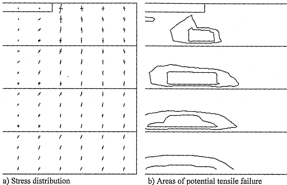
Figure 6.10 Results of a DIGS simulation near a stope abutment. Quarter symmetry, friction angle across bedding planes is 30 degrees
