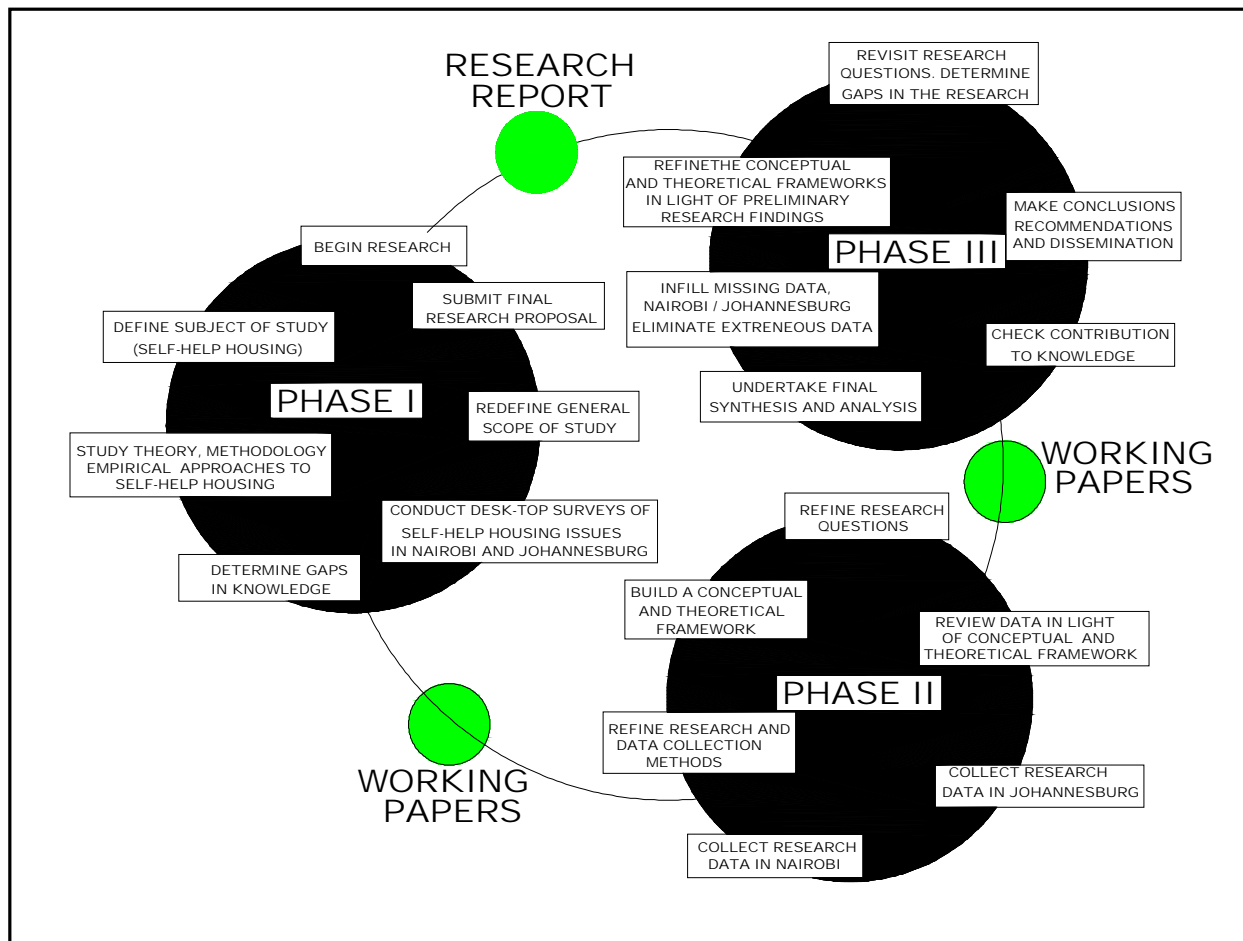
Figure 1.9. Research Strategy
