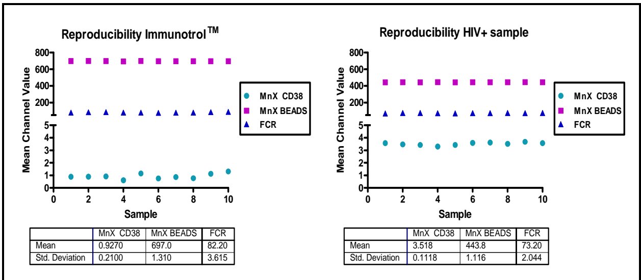
Figure 19: Reproducibility testing with ImmunoTrol™ (left) and an HIV+ patient sample (right), prepared as 10 replicates and analysed on the flow cytometer. FCR was also calculated as an internal quality control measure to establish instrument fluidic stability.
