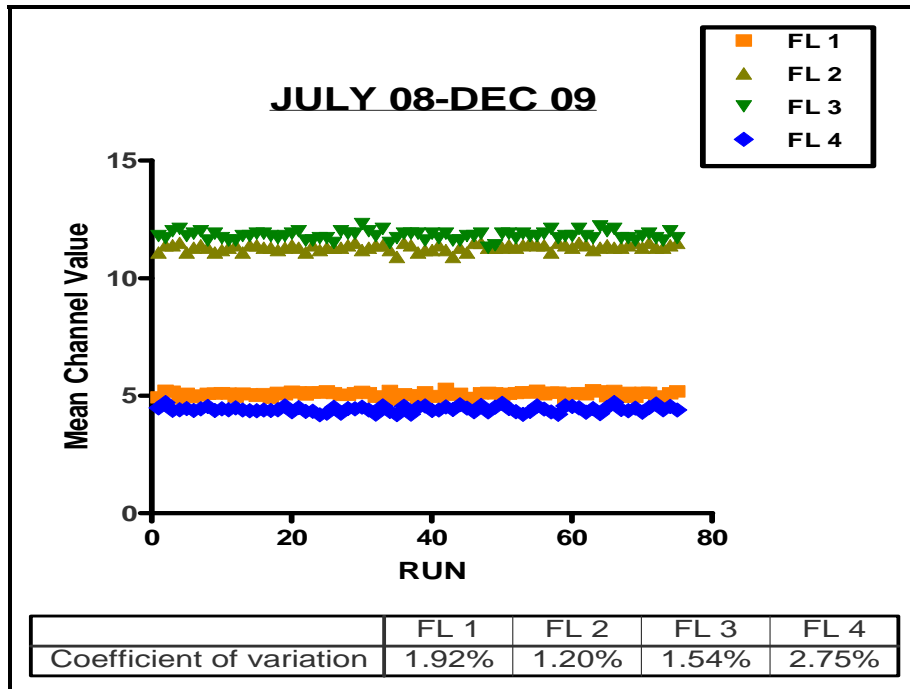
Figure 15: Weekly FlowSet™ results in a Levy Jennings style plot for the period July 2008 to December 2009. Mean channel values for the different fluorescent channels (FL1, FL2, FL3 and FL4) are shown.
