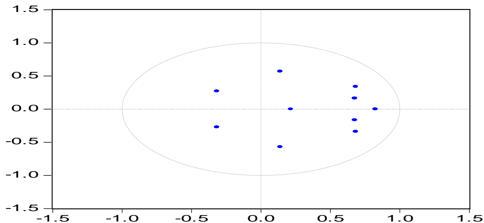
Figure 13 AR Roots
