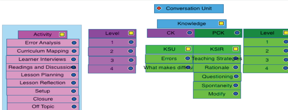
Figure 3.1: Code window
