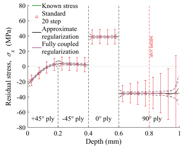
Fig. 7 Comparison of regularized integral solutions of \sigma_x for significant stress variation in the first ply in a [+45/-45/0/90]_s laminate
