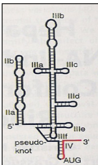
Fig.3. The IRES structure in the 5'untranslated region, with stem-loop domains IIa, IIb, IIIa-f, IV and pseudo-knot, red in figure (adapted from Wang et al.,2005)
