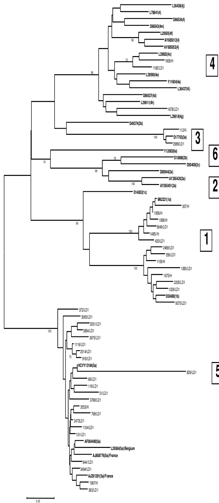
Fig.18. Unrooted neighbour-joining tree of 41 HCV isolates of the haemophilia, liver disease 1 and 2 groups. The region sequenced is 202bp in the NS5B region and clusters are shown of different genotypes and subtypes. Significant bootstrap values are indicated. GenBank accession numbers are in bold print with subtypes in parentheses. Genotypes are labelled according to the nomenclature of Simmonds et al., 1993a. The scale bar represents 0.05 substitutions/nucleotide site.
