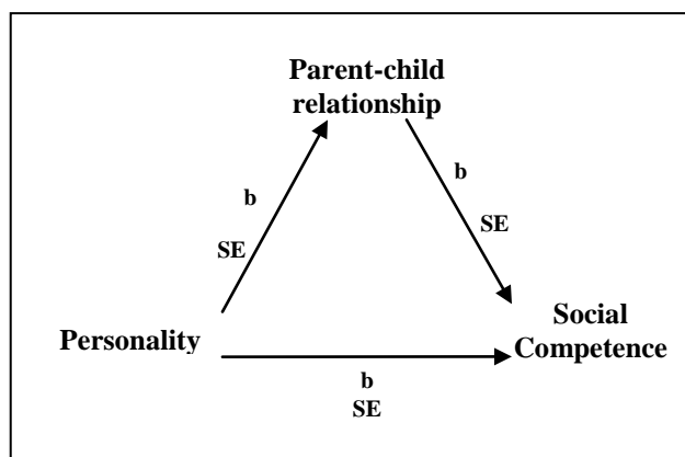
Figure 1. Proposed mediation model.
