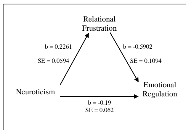
Figure 3. Mediation between Relational Frustration, Neuroticism and Emotional Regulation.
