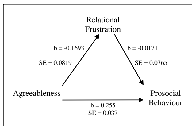
Figure 5. Mediation between Relational Frustration, Agreeableness and Prosocial Behaviour.
