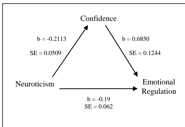
Figure 2. Mediation between Parenting Confidence, Neuroticism and Emotional Regulation.
