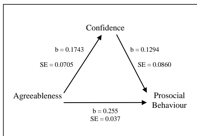
Figure 4. Mediation between Parenting Confidence, Agreeableness and Prosocial Behaviour.
