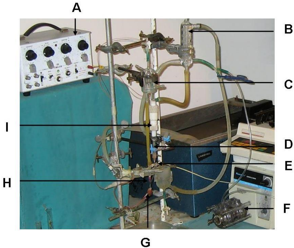
Figure 2.2. Isolated, perfused heart apparatus used in ex vivo experiments to assess cardiac structure and function. A, pacing device; B, heated water jacket; C, bubble trap; D, three way tap open to E, H and I; E, pressure transducer; F, peristaltic pump; G, platinum electrodes attached to the isolated heart; H, fluid filled catheter attached to latex balloon which is inserted into the left ventricular lumen; I, micromanipulator.
