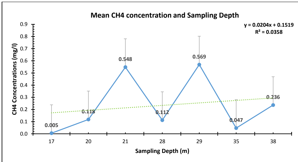
Figure 12: Mean CH 4 concentrations and sampling depth
