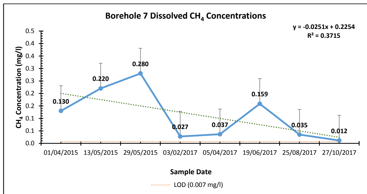
Figure 7: Borehole 7 dissolved CH 4 concentrations over time
