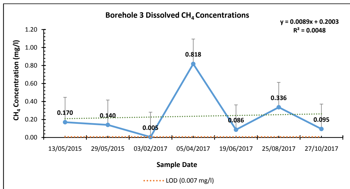
Figure 4: Borehole 3 dissolved CH 4 concentrations over time
