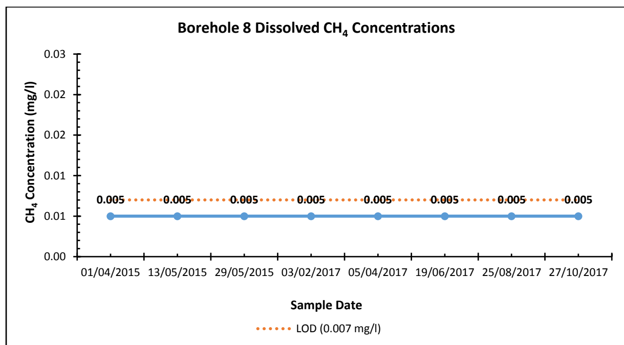
Figure 8: Borehole 8 dissolved CH 4 concentrations over time
