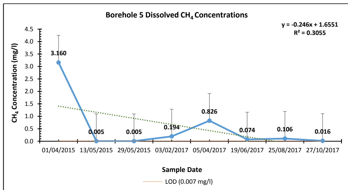
Figure 6: Borehole 5 dissolved CH 4 concentrations over time
