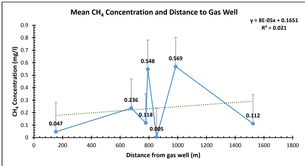
Figure 10: Mean CH 4 concentrations and distance to gas well
