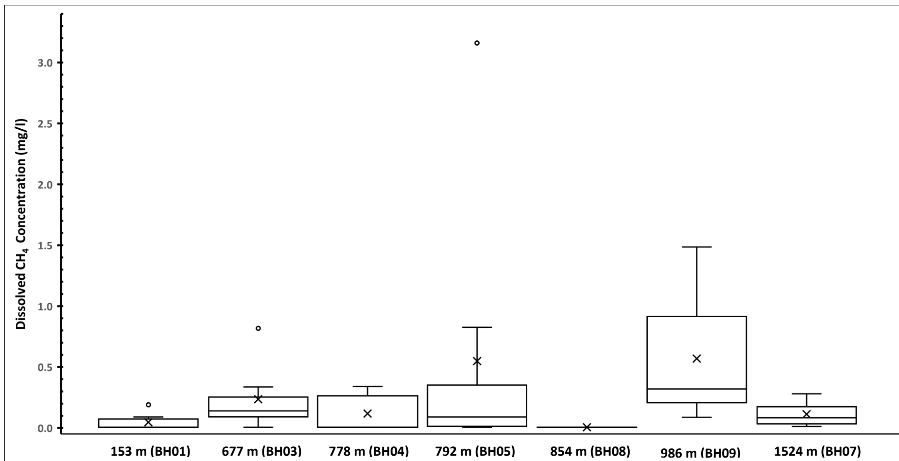
Figure 2: Boxplots of dissolved CH 4 concentrations by proximity to production well. All boxplots show the mean as an x, the median as the line within the box which represents the 1st and 3rd quartiles and whiskers indicating 1.5 times the interquartile range with points representing outliers.
