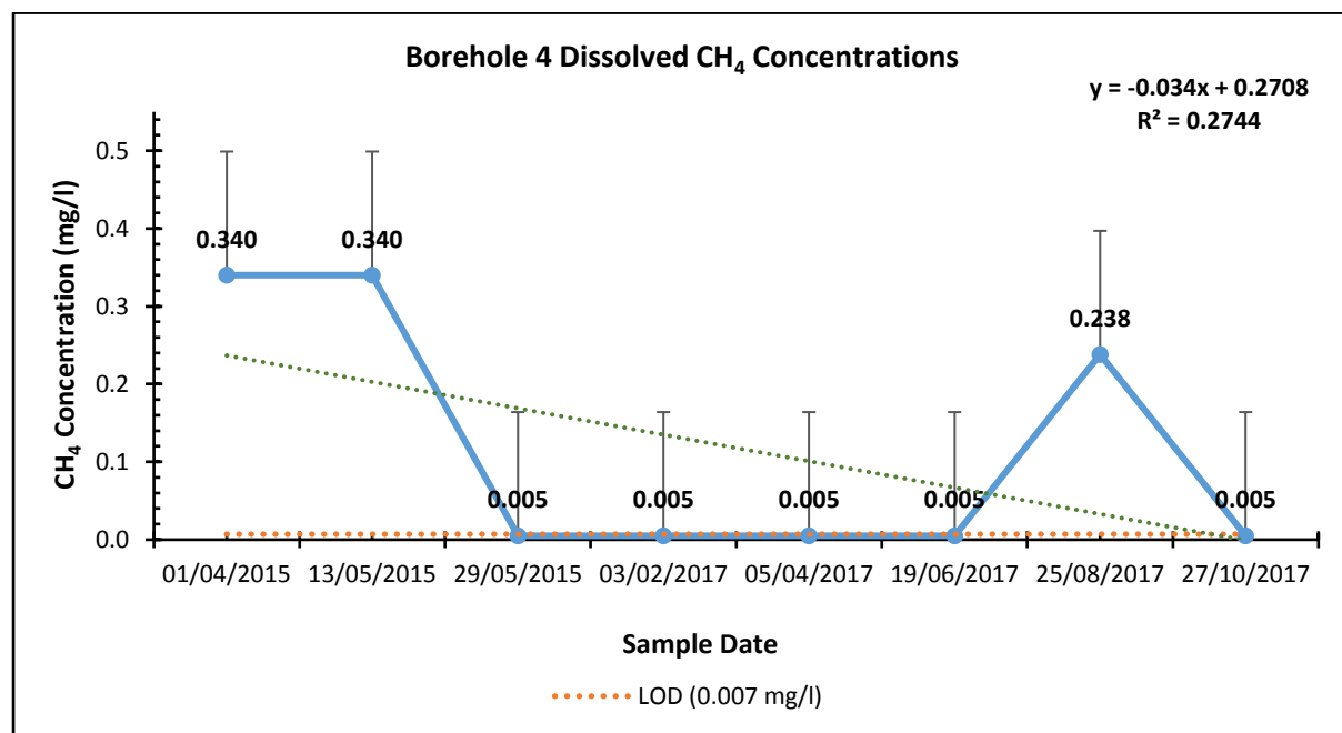
Figure 5: Borehole 4 dissolved CH 4 concentrations over time
