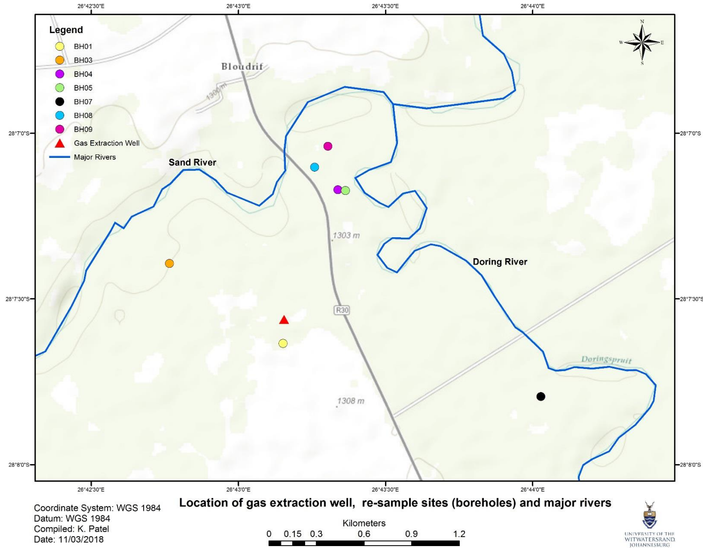
Figure 1: Location of gas extraction well, re-sample sites and major rivers
