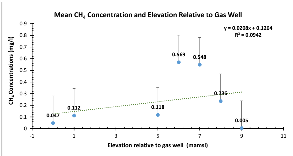
Figure 11: Mean CH 4 concentrations and elevation relative to production well.
