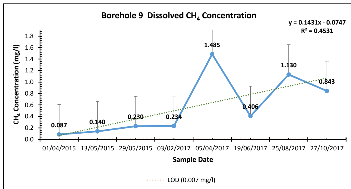
Figure 9: Borehole 9 dissolved CH 4 concentrations over time
