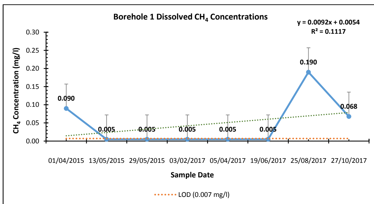
Figure 3: Borehole 1 dissolved CH 4 concentrations over time
