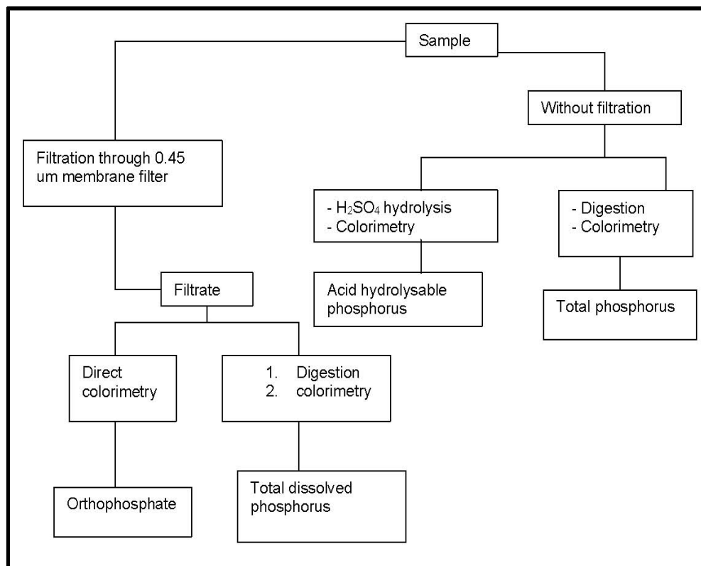
Figure 4.10: Flow chart of the procedure for phosphorous species measurements (STD Methods, 1994).
