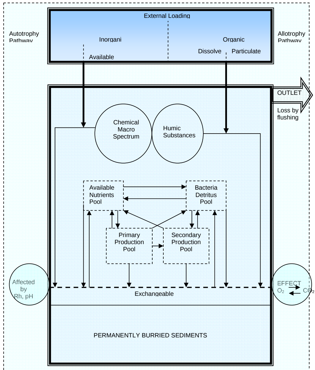
Figure 2.1: The main internal dynamics of a lake and relationships between internal and external loading (OECD, 1996).
