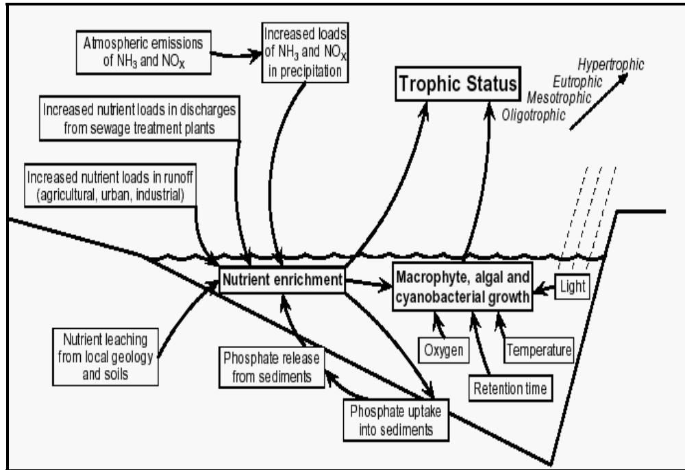
Figure 2.3: The main causes of eutrophication and other trophic states (DWAF, 2003).
