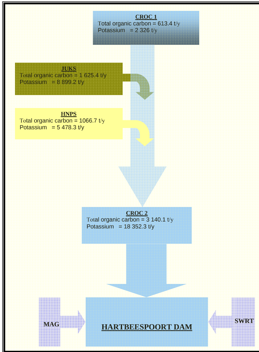
Figure 5.16: The total organic carbon and potassium mass loading into the Dam.
