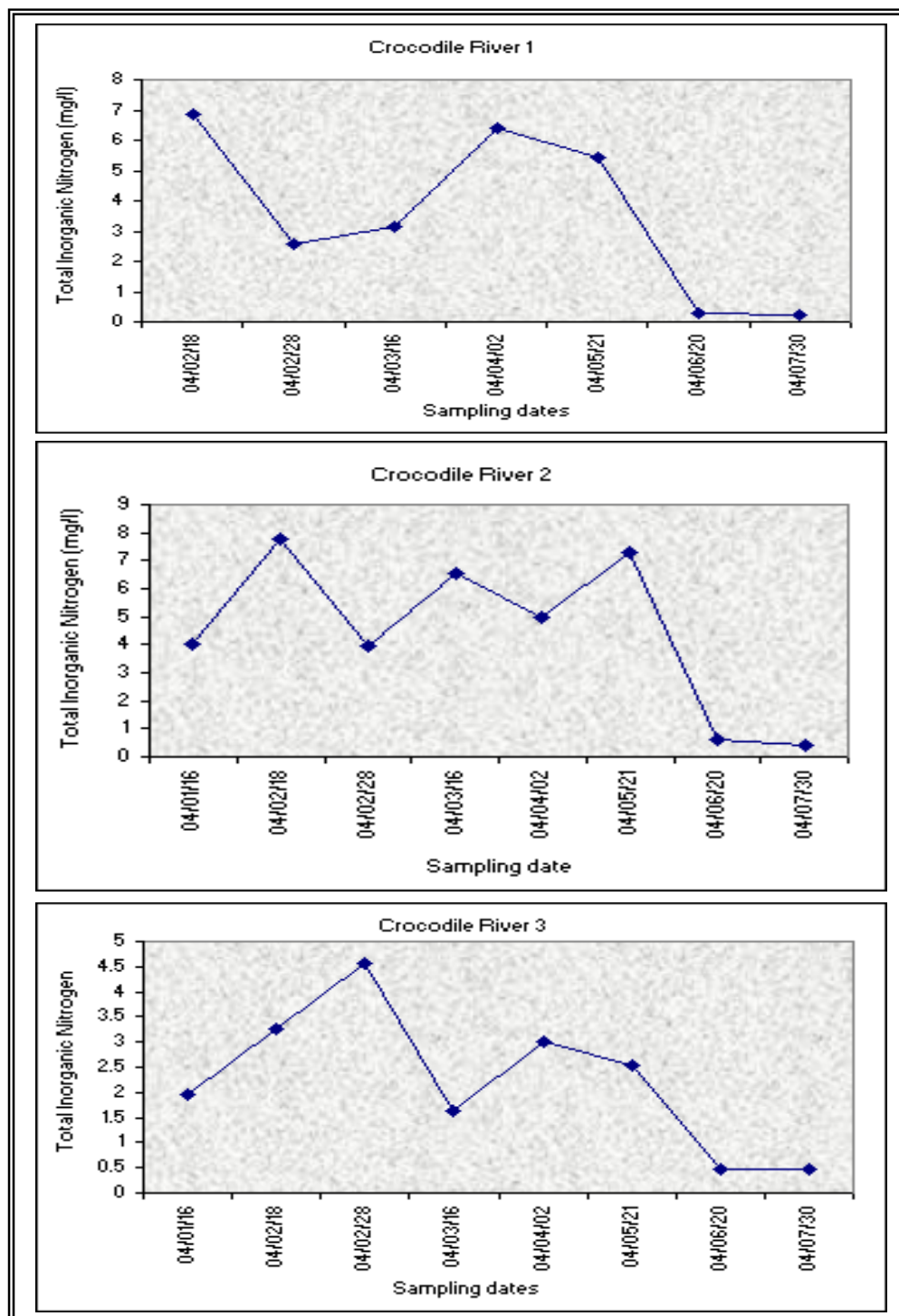
Figure 5.5 (b): The total inorganic nitrogen measured at CROC 1, CROC 2 and CROC 3.
