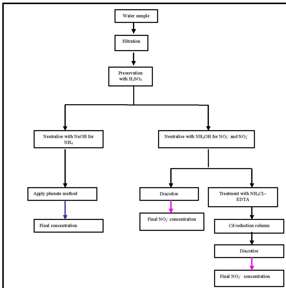
Figure 4.8: Flow chart of the procedure for nitrogen compounds measurements (Author).
