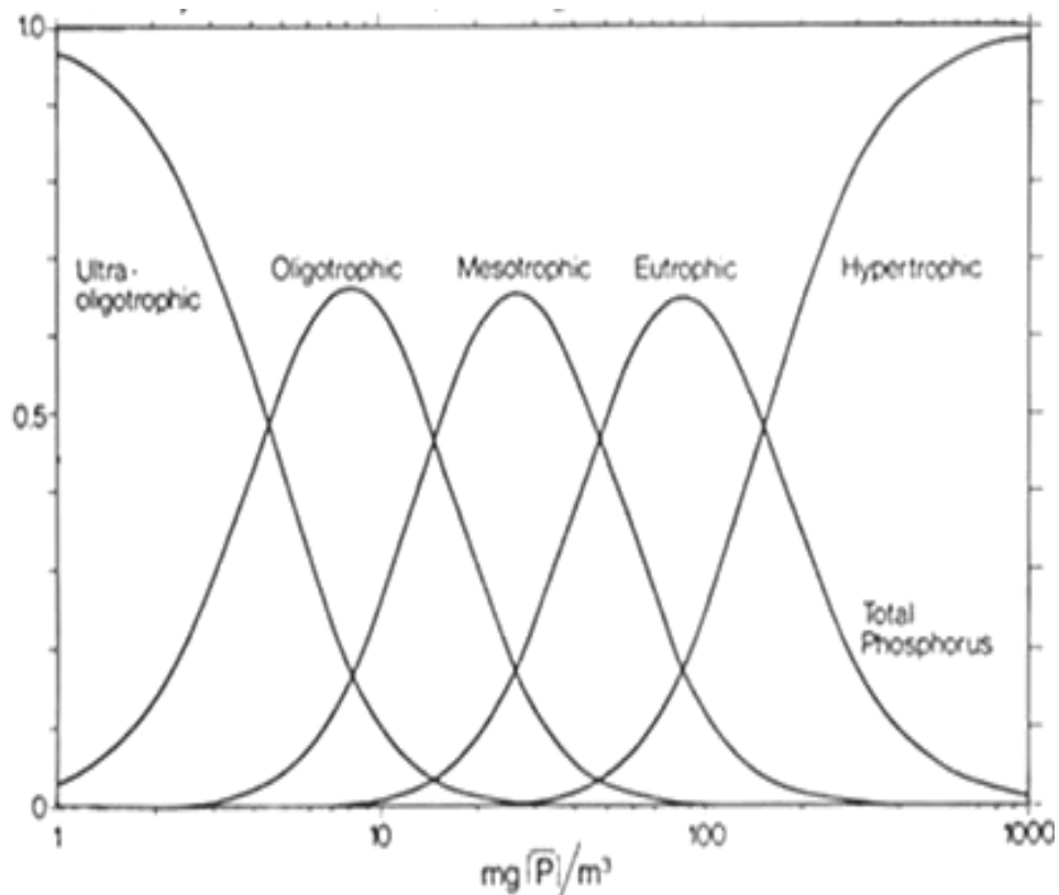
Figure 2.8: Relationship between the phosphorous concentration in a dam and probability of the occurrence of given trophic state (OECD, 1982)
