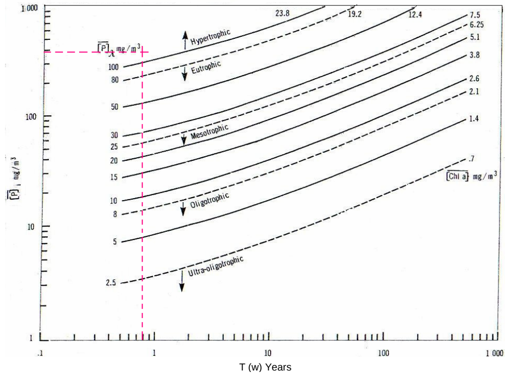
Figure 2.9: Relationships among retention time, P concentration, trophic state and chlorophyll-a concentration (OECD, 1982).
