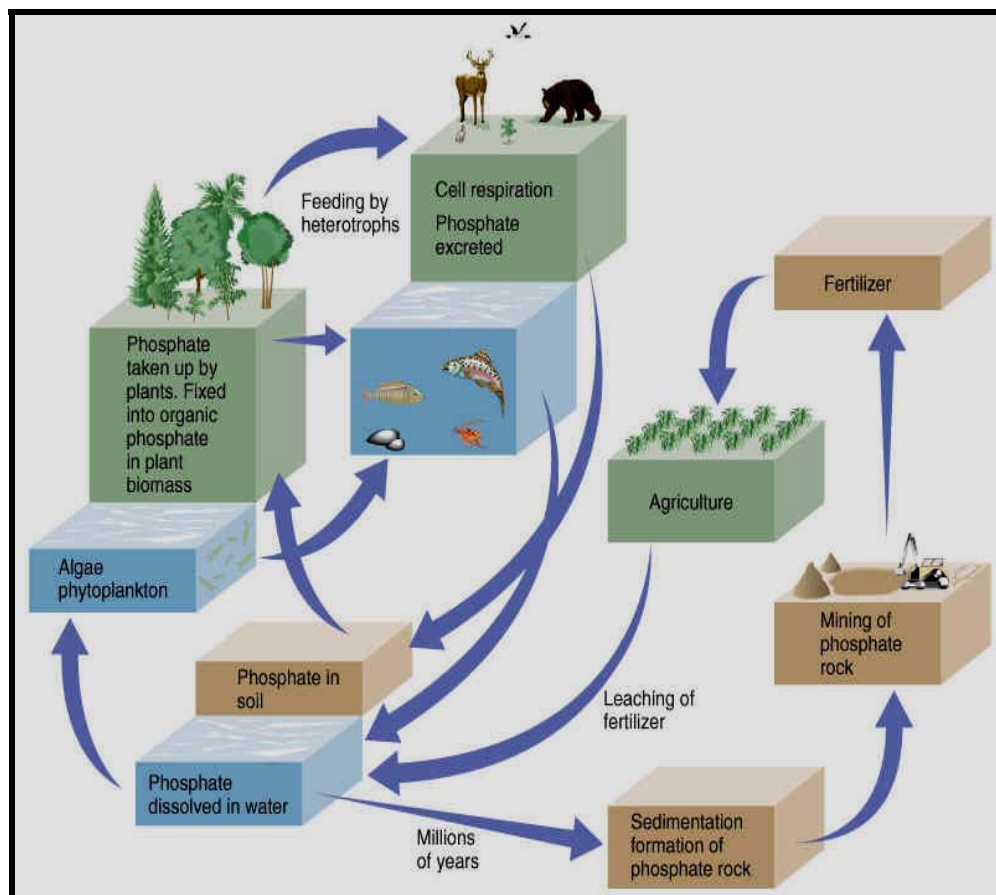
Figure 2.4: The Phosphorous cycle (TCL's courses 2005).
