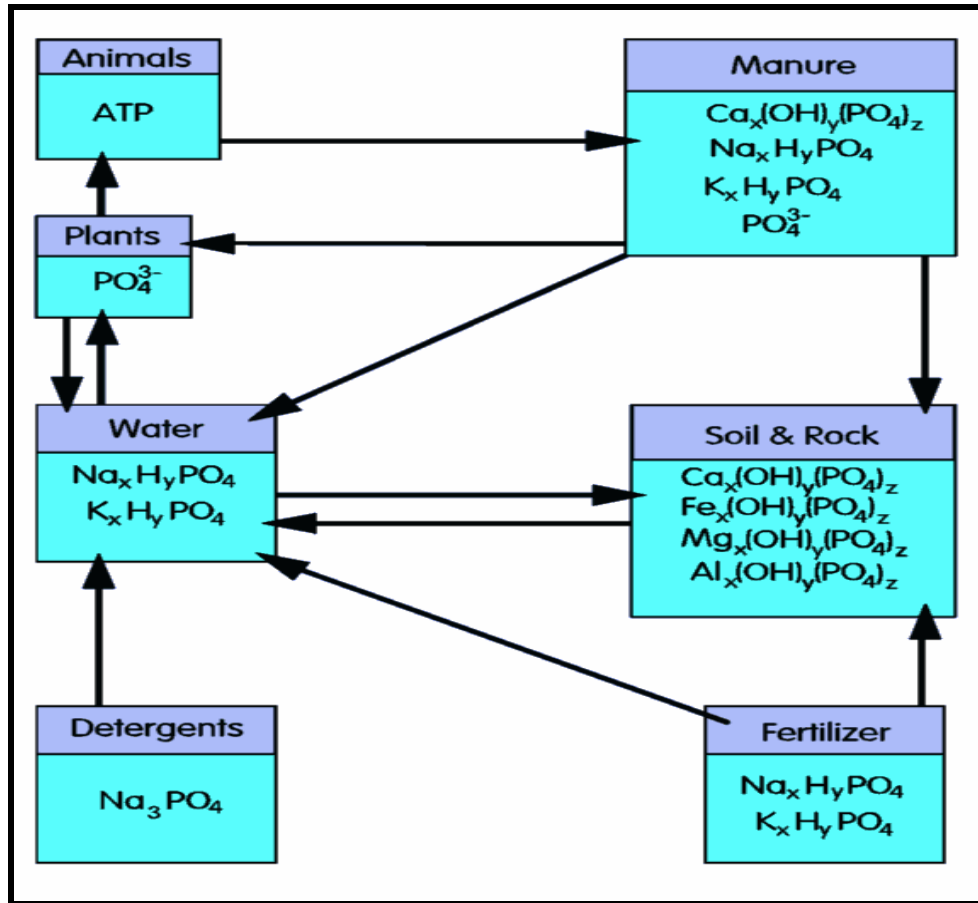
Figure 2.5: The association of phosphates with other chemicals in water (Edward, 2005).
