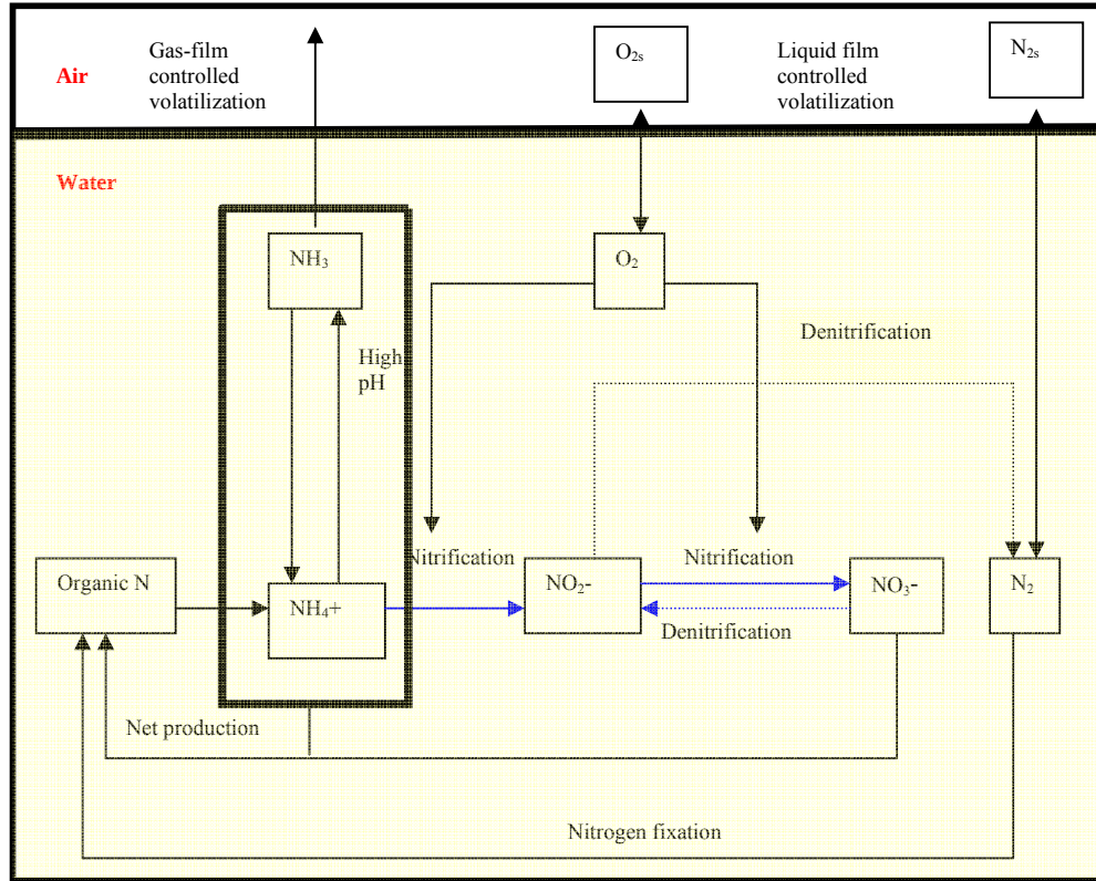
Figure 2.6: Nitrogen cycle in natural waters (Chapra, 1997).
