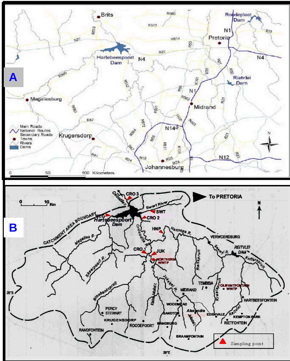
Figure 3.1: The regional setup (A) and the river networks (B) at the HBS Dam Catchment.
