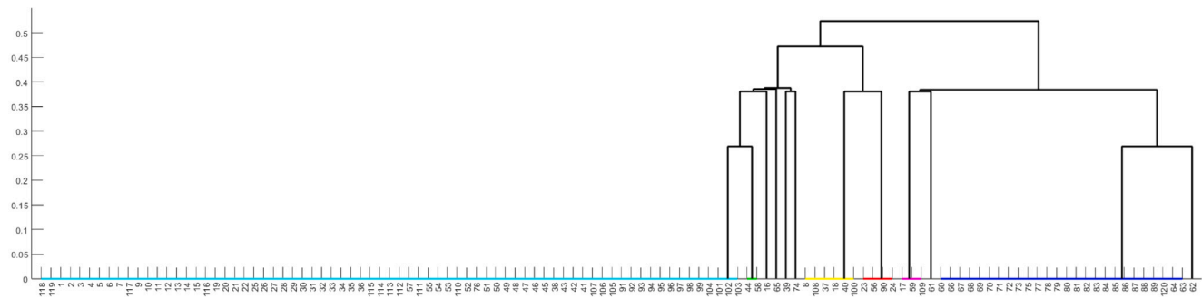
Fig. 8. Phylogenetic relationship among the co-mutated NSP14 sequences based on the relative frequency of BA, NA, AA, BB, NB, AB, BN, NN, and AN changes.
