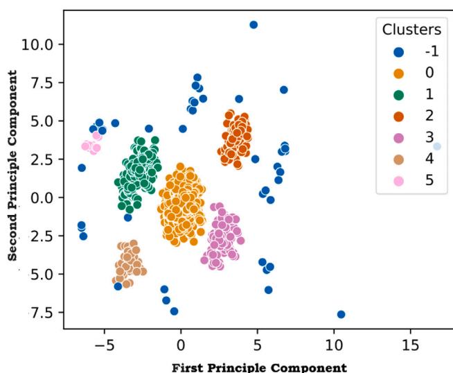
Fig. 13. Clustering of NSP14 variants based on the amino acid frequency distribution of 3953 SARS-CoV-2 NSP14 sequences.
