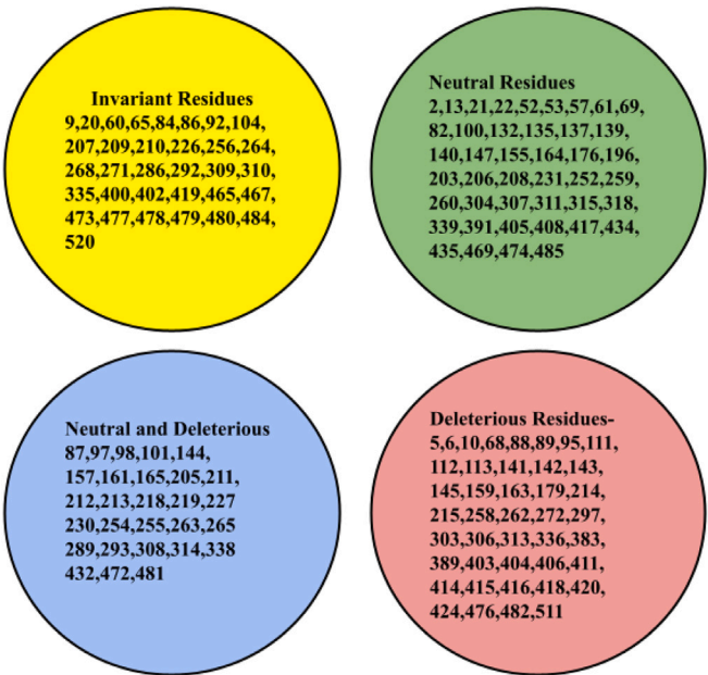
Fig. 10. Three disjoint classes of interacting residues based on pathogenicity of mutations were detected. Invariant interacting residues set is marked in yellow.
