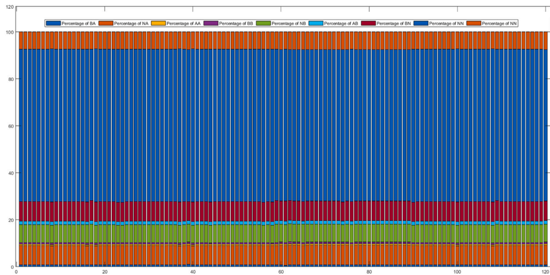
Fig. 7. Bar graph of the relative frequency of BA, NA, AA, BB, NB, AB, BN, NN, and AN changes among 120 co-mutated NSP14 sequences.
