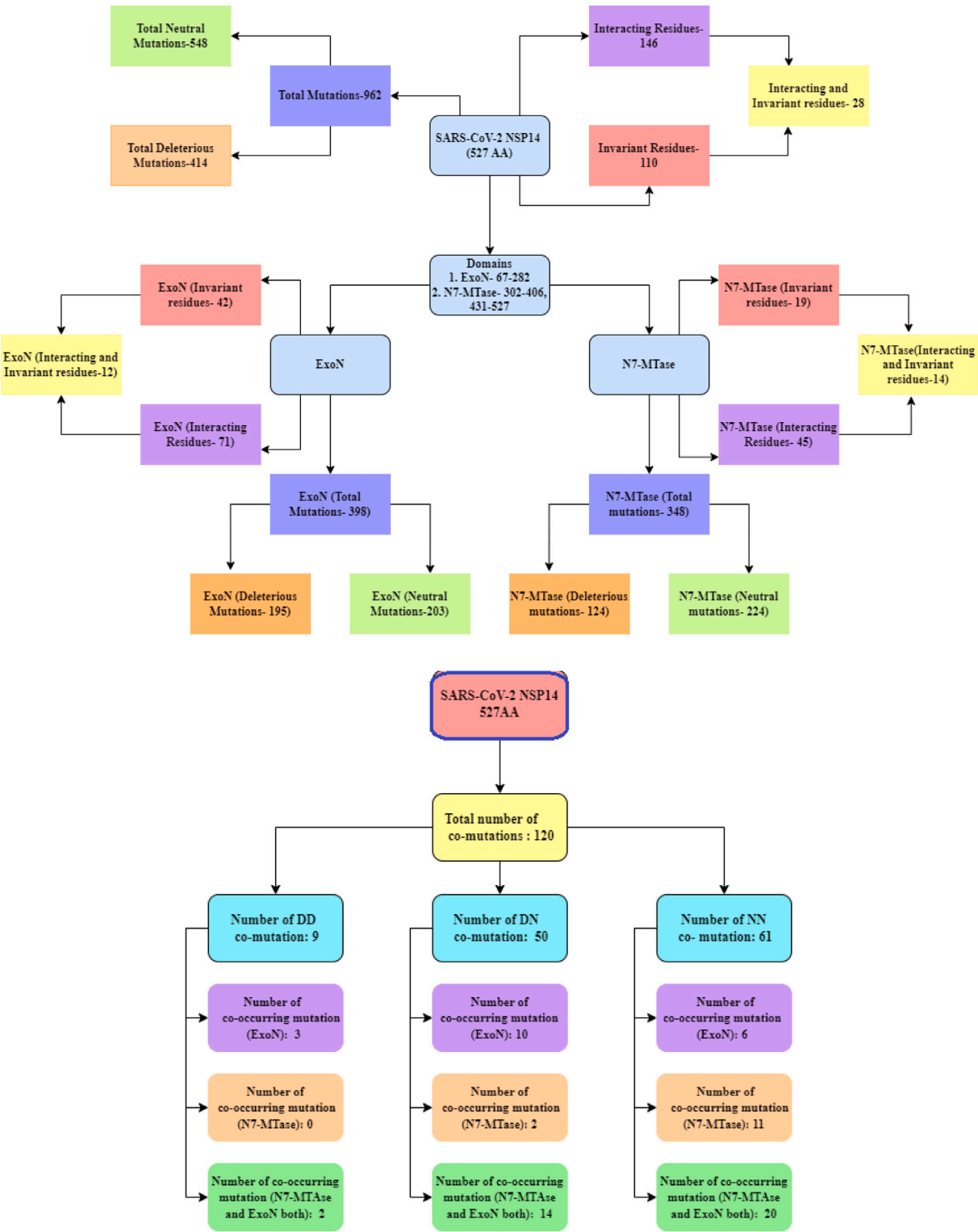
Fig. 16. Schematic snapshot of frequency of mutations and co-occurring mutations, invariant residues, and interacting residues in ExoN and N7-MTase domains in SARS-CoV-2 NSP14.
