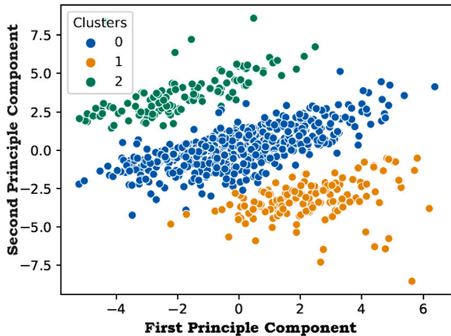
Fig. 15. Clusters 0, 1, and 2 contain 3201, 297, and 455 respectively.
