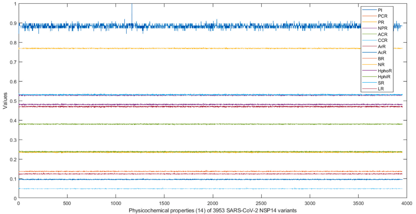
Fig. 14. Physicochemical features of 3953 SARS-CoV-2 NSP14 variants.
