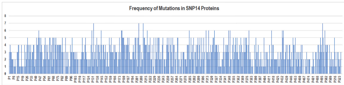
Fig. 1. Total frequency of mutations per mutant residues of NSP14 reference sequence (YP_009725309).
