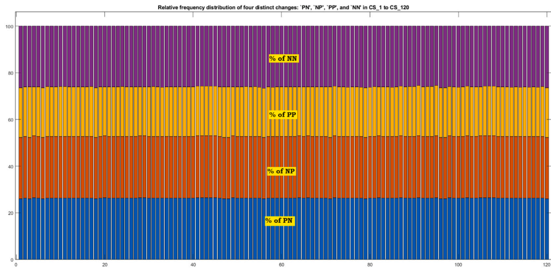
Fig. 5. Bar graph of the relative frequency of PN, NP, PP, and NN changes among 120 co-mutated NSP14 sequences.
