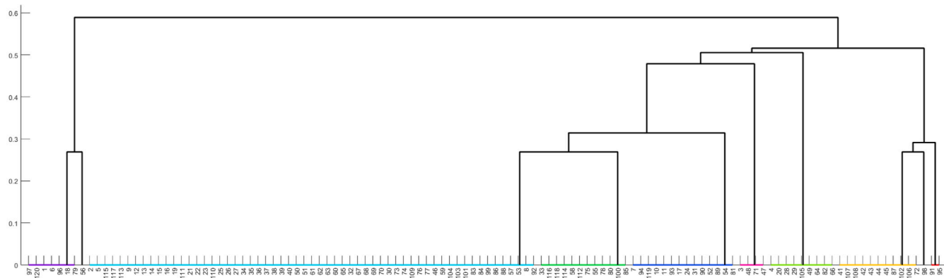
Fig. 6. Phylogenetic relationship among the co-mutated NSP14 sequences based on the relative frequency of PN, NP, PP, and NN changes.
