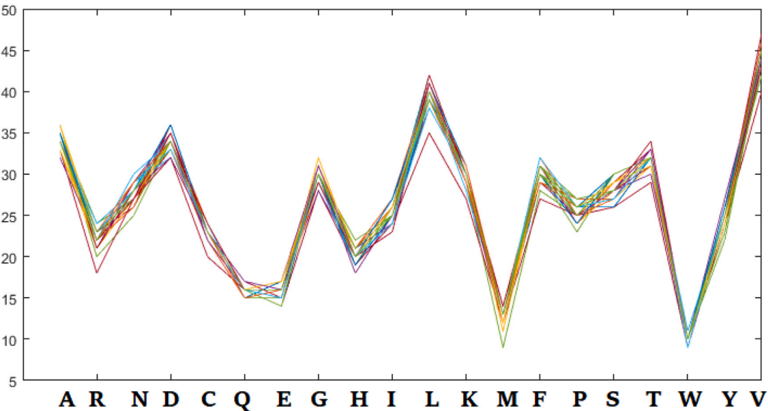
Fig. 11. Frequency distribution of each amino acids in 393 SARS-CoV-2 NSP14 sequences.
