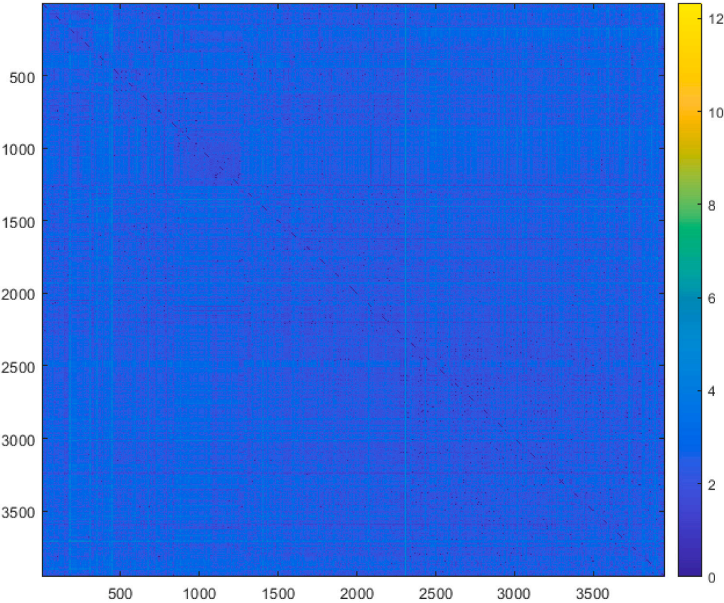
Fig. 12. Pairwise distances among 3953 SARS-CoV-2 NSP14 sequences.
