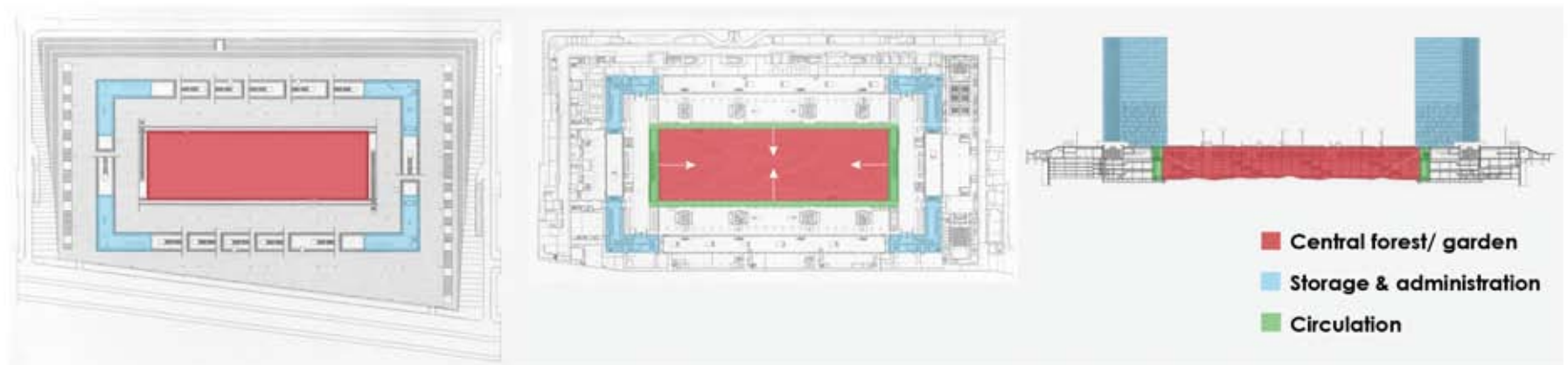
Overall building plan; Upper garden level plan; Longitudinal section (after Brawne 1997: 158 & 159)
