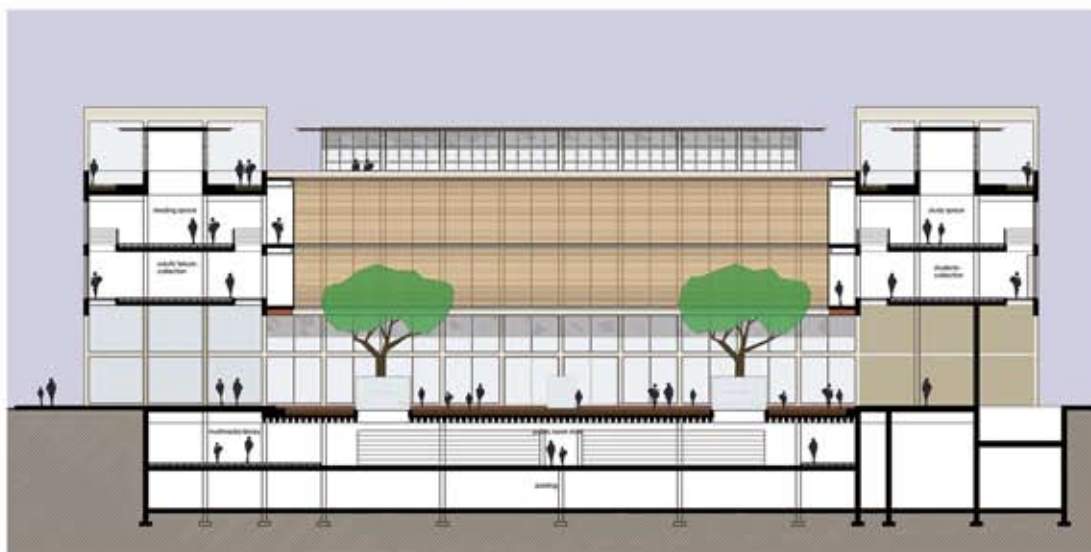
0 1 2 4 8 16 SECTION B-B: 1/500
