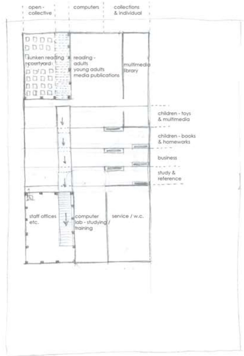
BASEMENT (-1) PLAN
