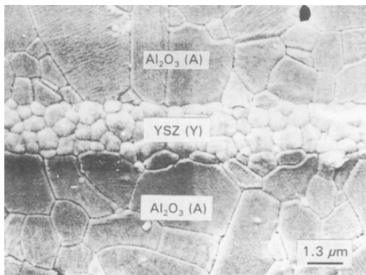
Figure 2.11: Boundaries between the sintered alumina/zirconia laminates by Sarkar and Nicholson [40].
