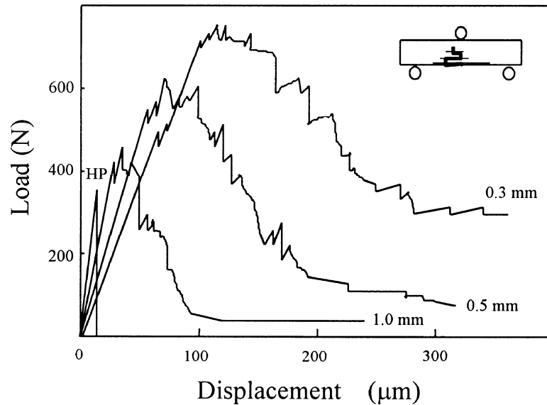
Figure 2.2: Typical load-displacement curve of fibrous monolithic Si 3 N 4 /BN showing the plots for extruded fibres of diameter 1mm, 0.5mm and 0.3mm. [2]
