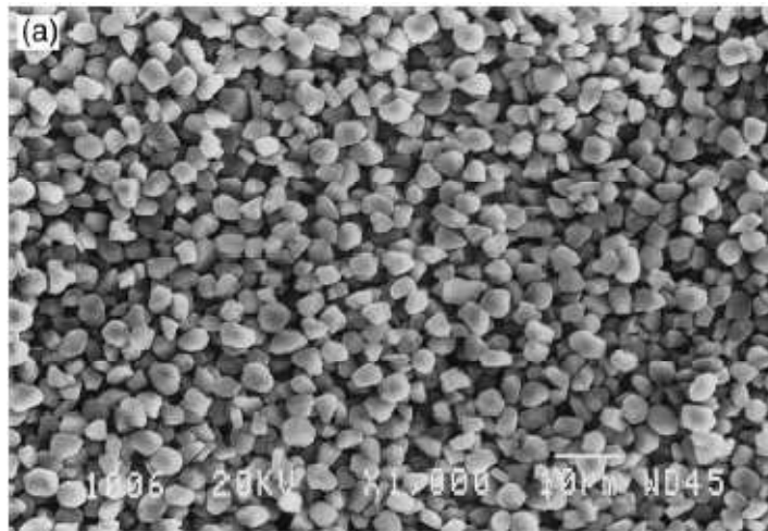
Figure 2.10: SEM picture of the diamond deposit obtained using an isopropanol suspension with acetone, iodine and water as additives [36].
