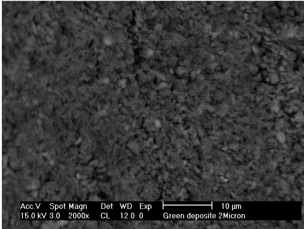
Figure 4.15: SEM image of the green deposit of a sample 53 made using a 2µm diamond suspension.
