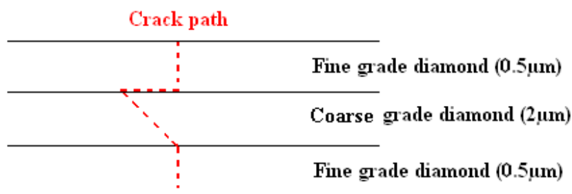
Figure 2.18: Illustration of the expected crack path through the sintered layered material.
