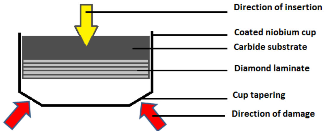
Figure 5.7: Illustration showing the effect of the cup tapering on the edges of the diamond laminate.
