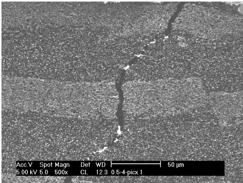
Figure 4.35: SEM micrograph of a pre-existing crack showing crack deflection in the laminate material.
