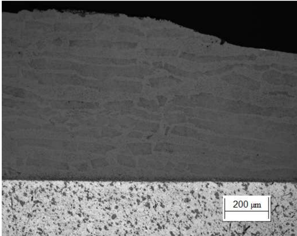
Figure 4.31: Optical microscope picture showing damage sustained at the edge of the sample.
