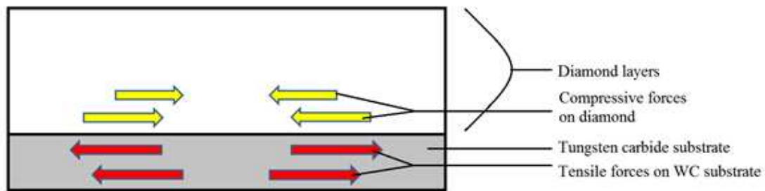
Figure 5.8: Schematic illustration of the compressive forces generated due to the mismatch in thermal expansion between the diamond and the substrate.
