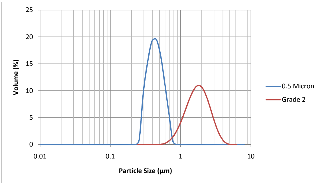
Figure 3.2: Particle size distribution of diamond powders used.
