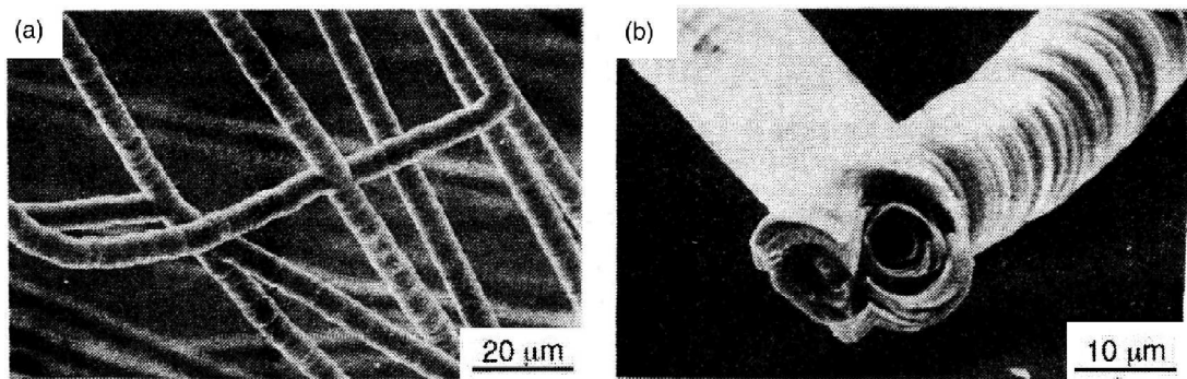
Figure 2.4: a) Microstructure of vapor-grown carbon fibers resembling tree roots b) structure of a branching point [19]
