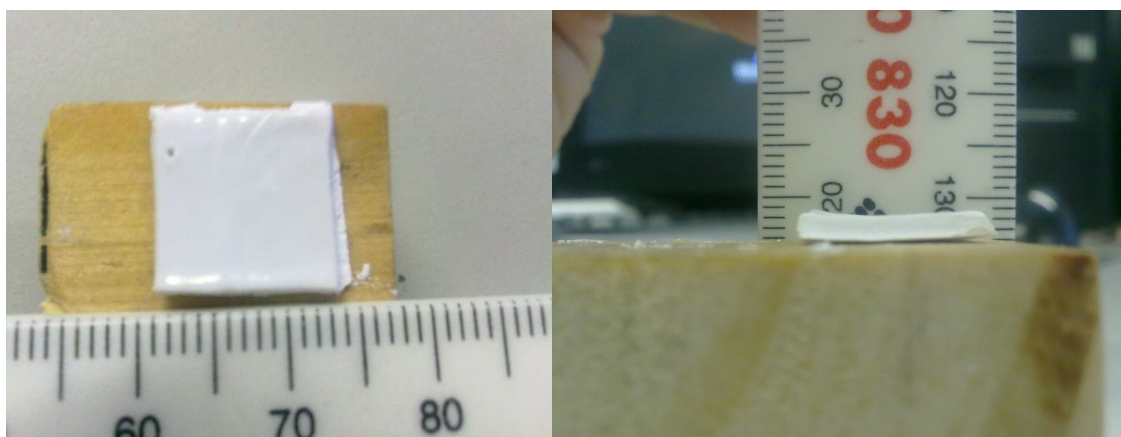
Figure 4.7: Photograph showing Sample 41 prepared using a 10% (w/v) alumina suspended in isopropanol at pH 3.7, 50V/cm for 1 hour.
