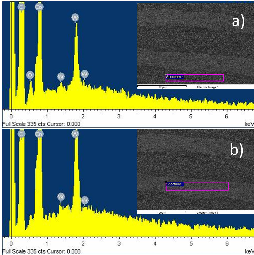
Figure 4.27: EDS scans for the first 2 \mu\text{m} layer (a) and the first 0.5 \mu\text{m} layer (b) of the diamond laminate sample.
