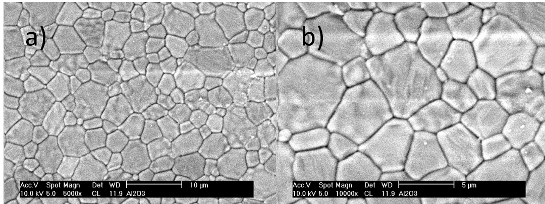
Figure 4.9: SEM micrographs of sample 42 at a) 5000x b) 10000x magnification.
