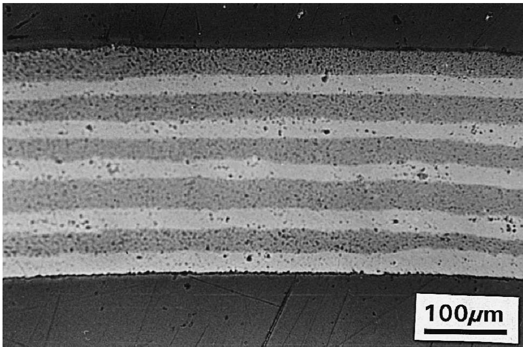
Figure 2.13: Alumina/zirconia laminates prepared by EPD using a suspension of each of the materials with 0.6% deflocculant [42]
