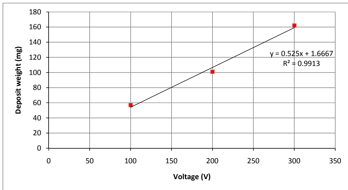
Figure 4.5: Deposit weight versus applied voltage for a suspension of pH 5.0, 10% (w/v) for 15 minutes.
