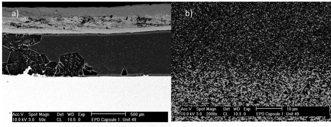
Figure 4.17: SEM of the cross section of sample 49 which was made by depositing 0.5μm diamond.
