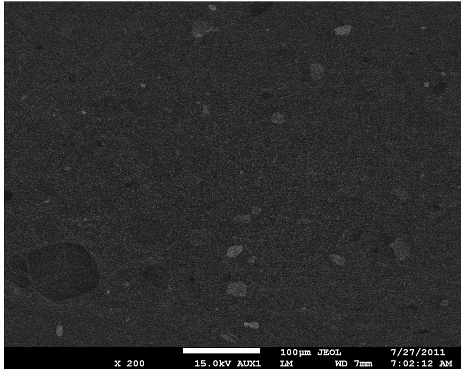
Figure 4.21: SEM showing light and dark spots in the diamond table of the 0.5µm powder pressed standard.
