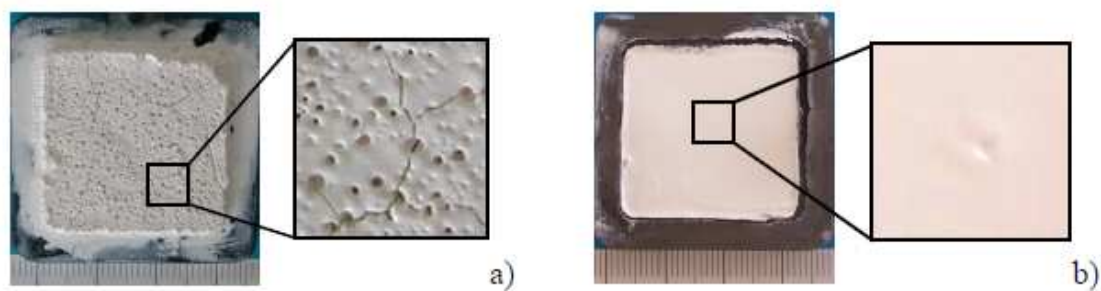
Figure 2.9: Alpha-Al 2 O 3 deposits formed using (a) 100 V DC for 1200 s and (b) a 50 Hz asymmetric AC field with an amplitude of 500 V p-p [37].
