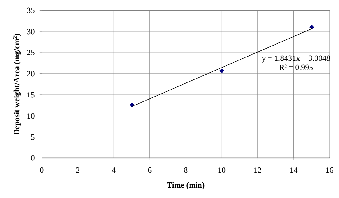
Figure 4.6: Deposit weight versus time for a suspension of pH 5.0, 10% (w/v) at 100V/cm.
