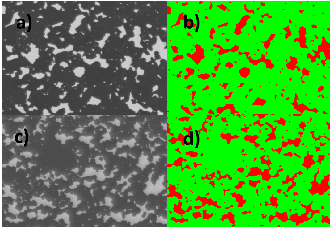
Figure 4.29: SEM Image analysis showing the phase thresh-holding for the 2 \mu m layer in a) and b) and the 0.5 \mu m layer in c) and d).
