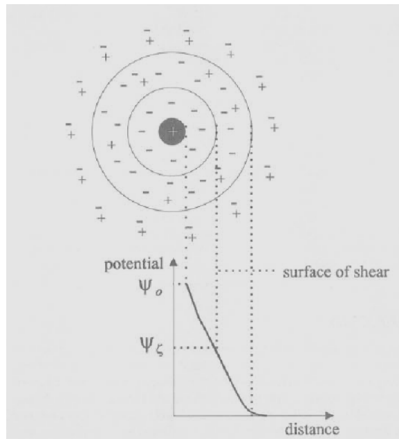
Figure 2.7: Diagram of the double layer surrounding a charged particle. The potential at the surface of shear is termed the zeta potential. It is the main parameter determining electro-kinetic behaviour [27].
