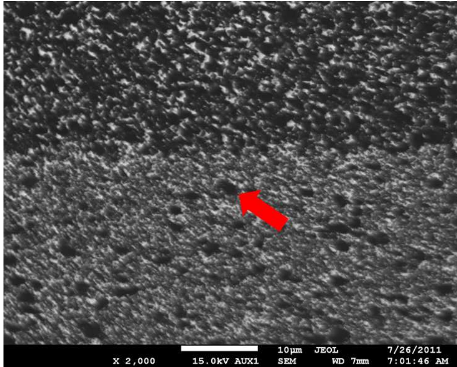
Figure 4.32: SEM showing the inclusion of larger grains in the fine grade layer.
