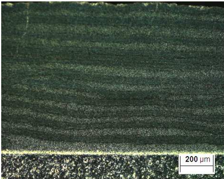
Figure 4.25: Optical microscope picture of the diamond laminate sample showing the overall structure.
