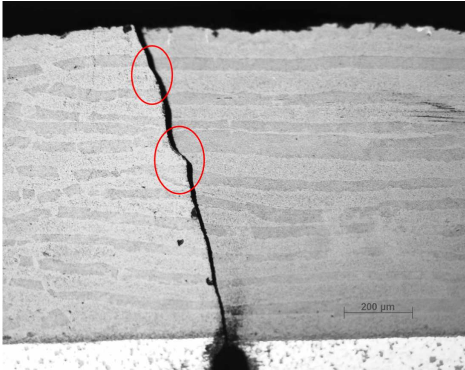
Figure 4.33: An optical microscope picture showing the direction of a forced crack path.
