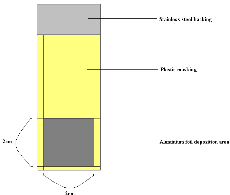
Figure 3.3: Schematic of the working electrode used for alumina deposition.
