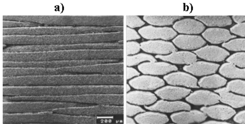
Figure 2.1: a) Longitudinal and b) cross-section microstructure of the fibrous monolithic \text{Si}_3\text{N}_4/\text{BN} resembling the structure of bamboo [2]
