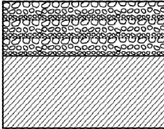
Figure 2.17: Another schematic of a functionally graded material achievable by the agitation of multimodal powders [55].
