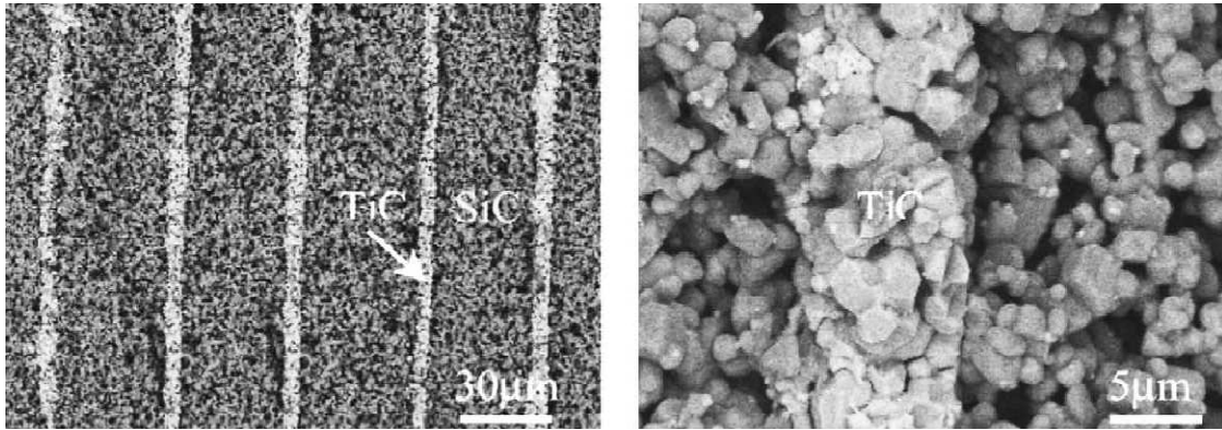
Figure 2.12: SEM image showing the pressureless sintered SiC/TiC laminates achieved by You et al. [41]
