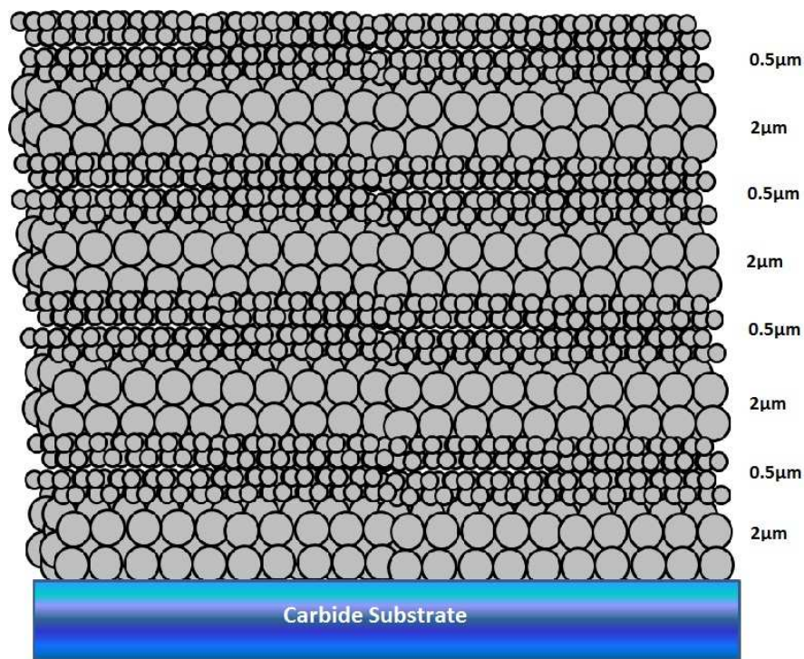
Figure 1.1: Schematic diagram showing the alternating layers of 0.5μm and 2μm grade diamond on a carbide substrate.
