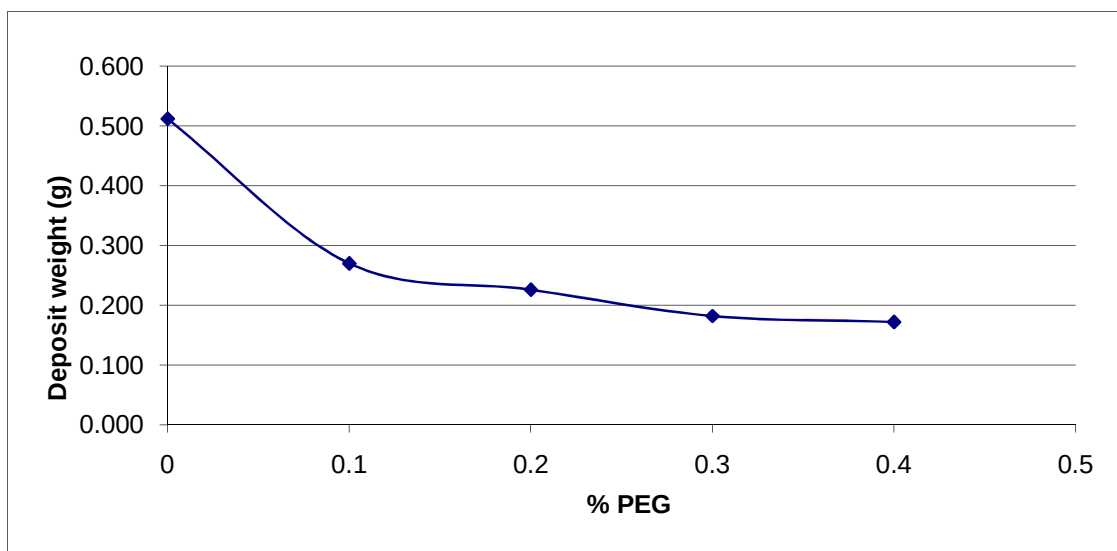
Figure 4.3: A graph showing the weight of the deposit versus % PEG-400 addition. Deposits were made using 175V/cm, 10% (w/v) for 1 hour.
