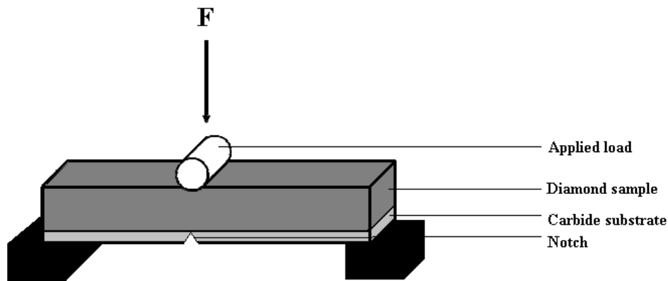
Figure 3.8: Schematic of the 3-point bend jig apparatus used to produce a controlled crack.
