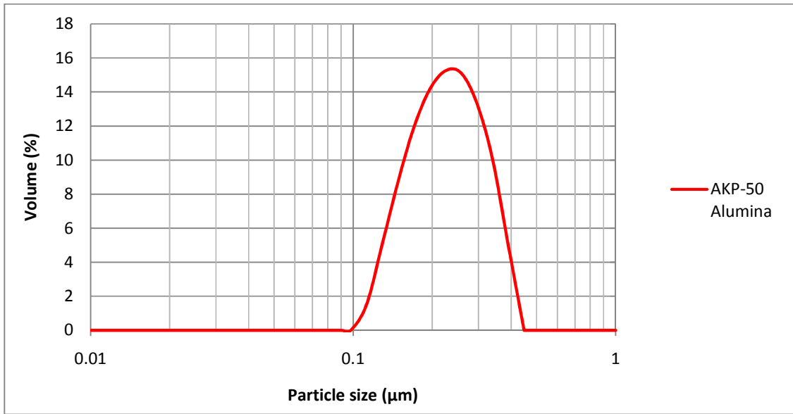
Figure 3.1: Particle size distribution of AKP-50 alumina.
