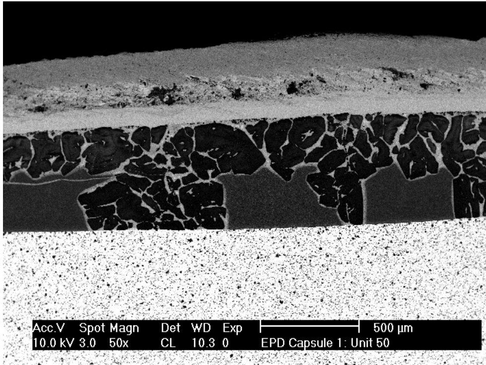
Figure 4.18: SEM of the cross section of sample 50.
