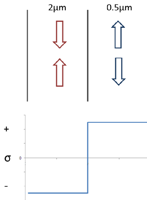
Figure 5.9: A schematic diagram showing the stress distribution in the layers.
