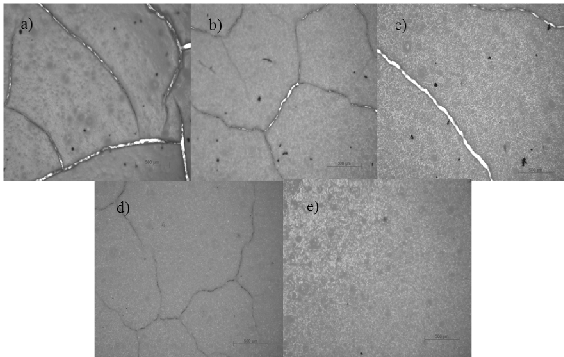
Figure 4.2: Effect of PEG-400 addition on the formation of cracks in the deposit. Weight per cent PEG-400 addition to suspension: a) 0% b) 0.1% c) 0.2% d) 0.3% e) 0.4%.
