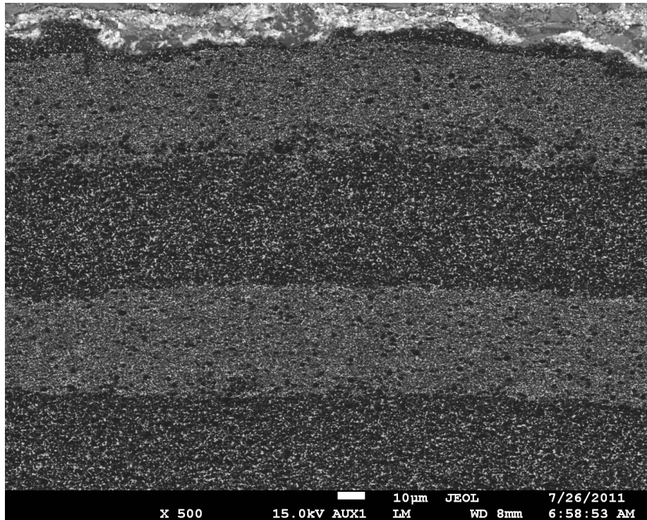
Figure 4.26: SEM micrograph of a uniform section showing the morphology of the layers.
