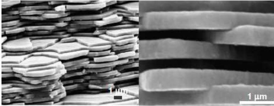
Figure 2.5: An SEM image of the micro-structure of nacre [12].
