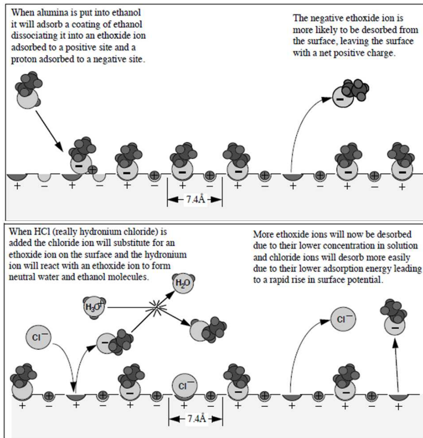
Figure 5.1: (Top) Mechanism of surface charging for alumina in ethanol. (Bottom) Effect of charged surface after the addition of HCl. [68]
