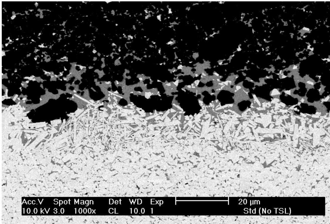
Figure 2.14: SEM micrograph of a typical PCD sintered at 8.5GPa and 1400°C [48].
