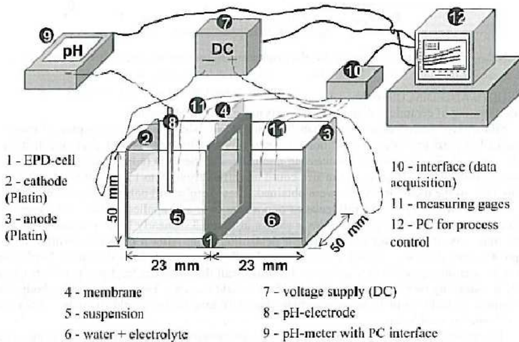
Figure 2.8: Diagram of the typical EPD setup for aqueous deposition with a membrane between the two electrodes [33].
