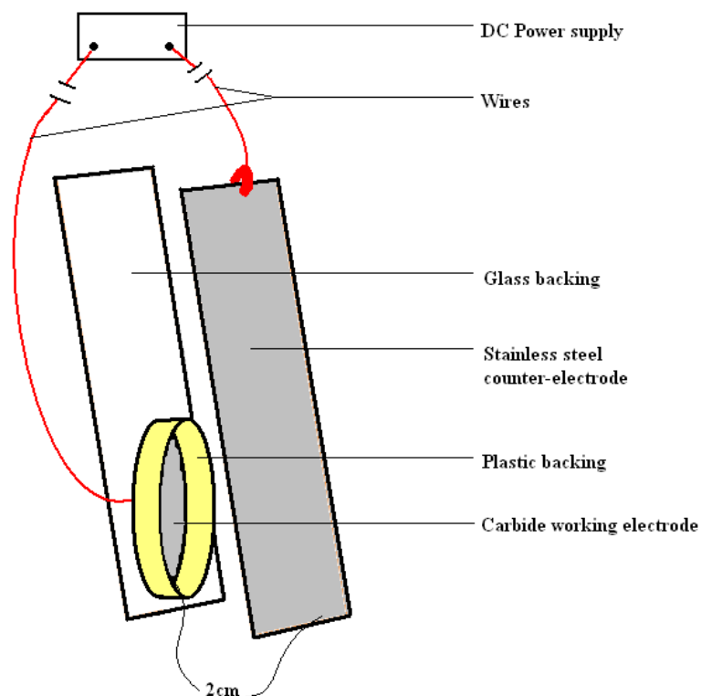
Figure 3.4: Schematic showing the experimental setup of both the working electrode and the counter-electrode.
