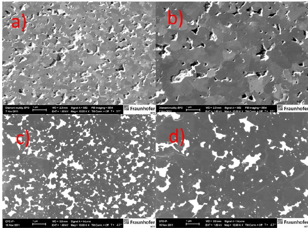
Figure 4.28: Comparison of polishing techniques: a) 0.5μm layer standard polish, b) 2μm layer standard polish, c) 0.5μm ion polish, 2μm ion polish.
