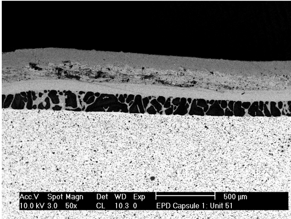
Figure 4.19: SEM of the cross section of sample 51.
