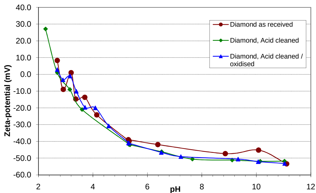
Figure 4.12: Graph of zeta-potential versus pH for the various powders in aqueous media.
