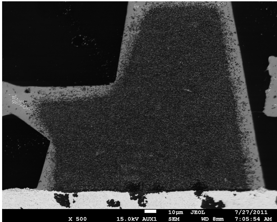
Figure 4.20: SEM of 0.5µm powder pressed standard.
