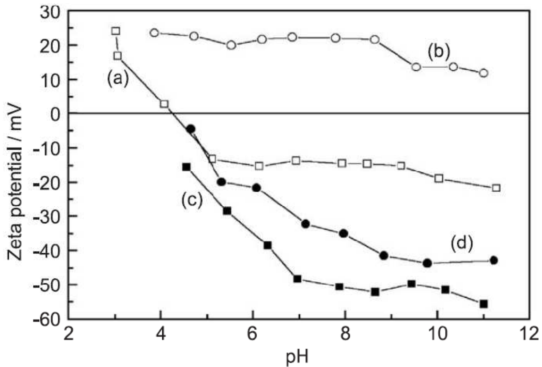
Figure 5.5: Zeta-potential vs. pH plot for detonated nano-diamond treated with: a) perchloric acid; b) sulphuric acid and potassium permanganate; c) perchloric acid and 10^{-3} \text{ mol.dm}^{-3} sodium oleate; d) sulphuric acid, potassium permanganate and 10^{-3} \text{ mol.dm}^{-3} sodium oleate [75].
