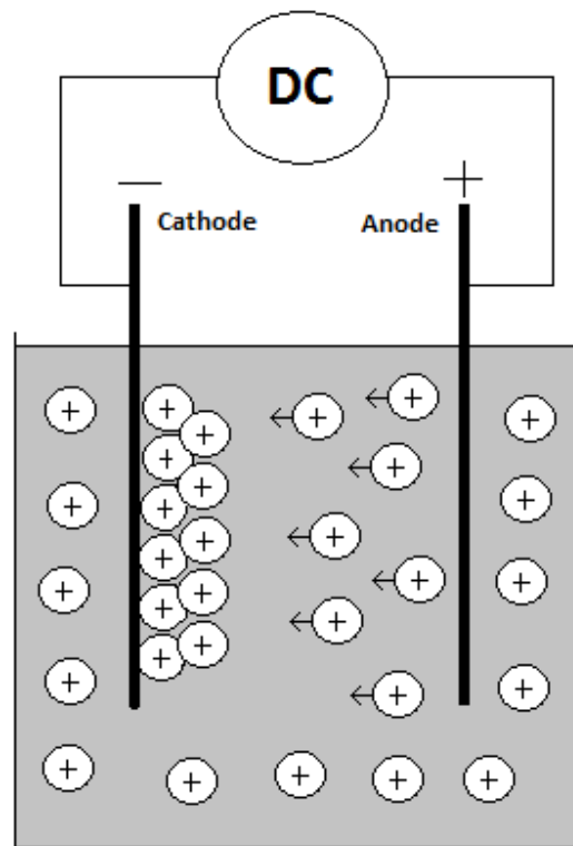
Figure 2.6: Typical EPD setup.
