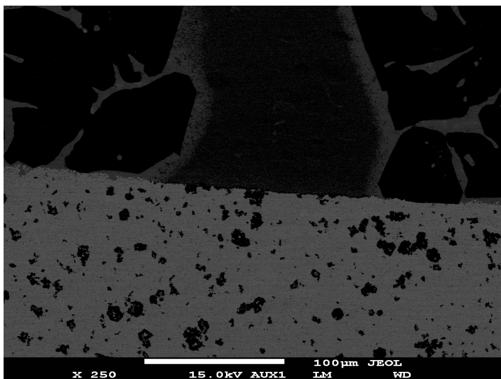
Figure 4.22: SEM of the 2µm powder pressed standard.
