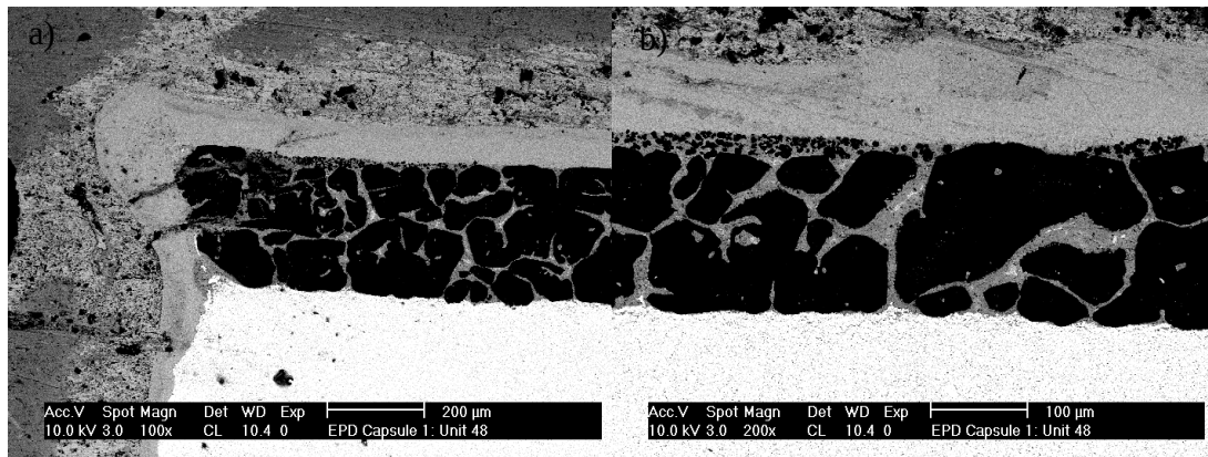
Figure 4.16: SEM of the cross section of sample 48 which was made by depositing 0.5μm diamond.
