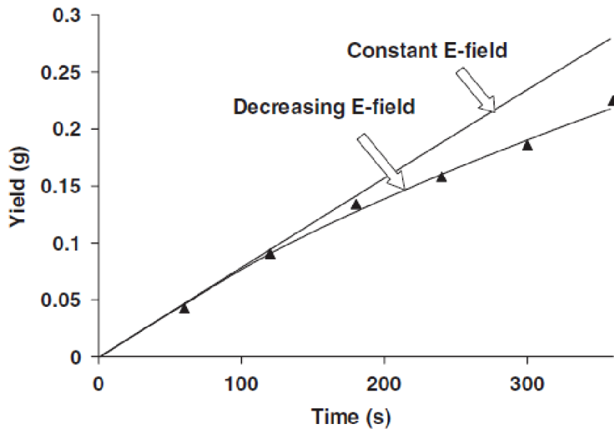
Figure 5.2: Graph showing the difference between predicted and experimental yield of deposited \text{Al}_2\text{O}_3 from ethanol- \text{HNO}_3 suspensions using a constant voltage of 42.7V/cm [69].
