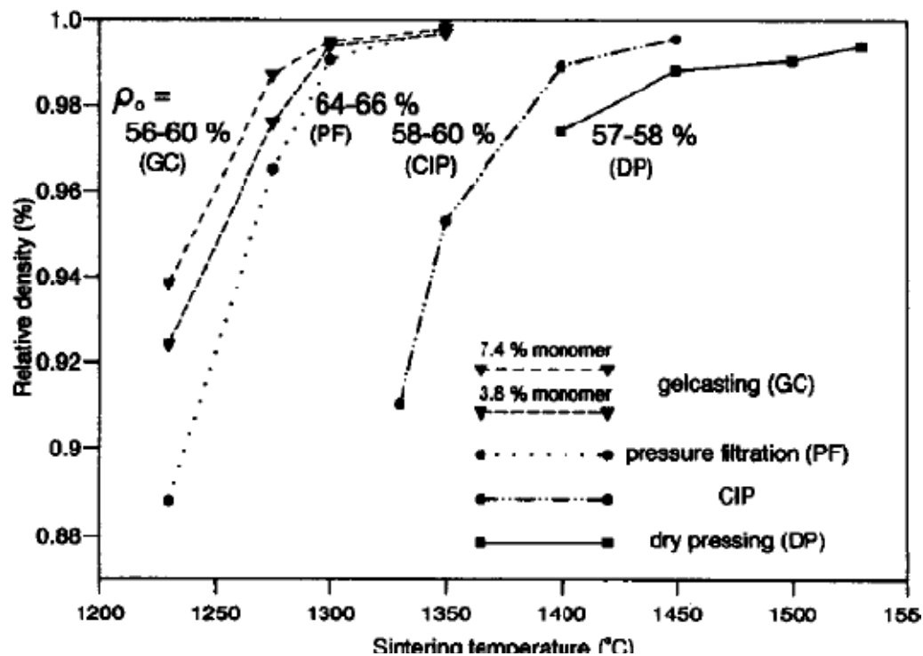
Figure 5.3: Effect of the shaping method and green density on the temperature effect on isothermal sintering for the same alumina powder [73].
