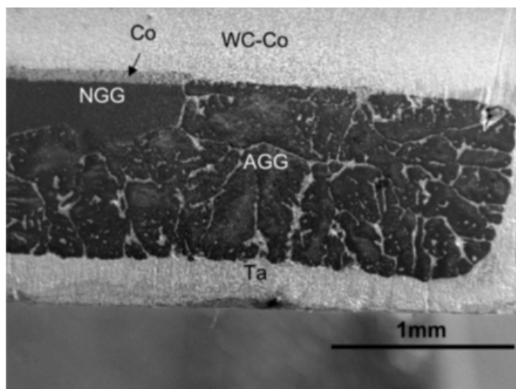
Figure 2.15: SEM of the micro-structure of the cross section of a PCD sintered compact made using 2\mu\text{m} diamond powder exhibiting AGG. [51].
