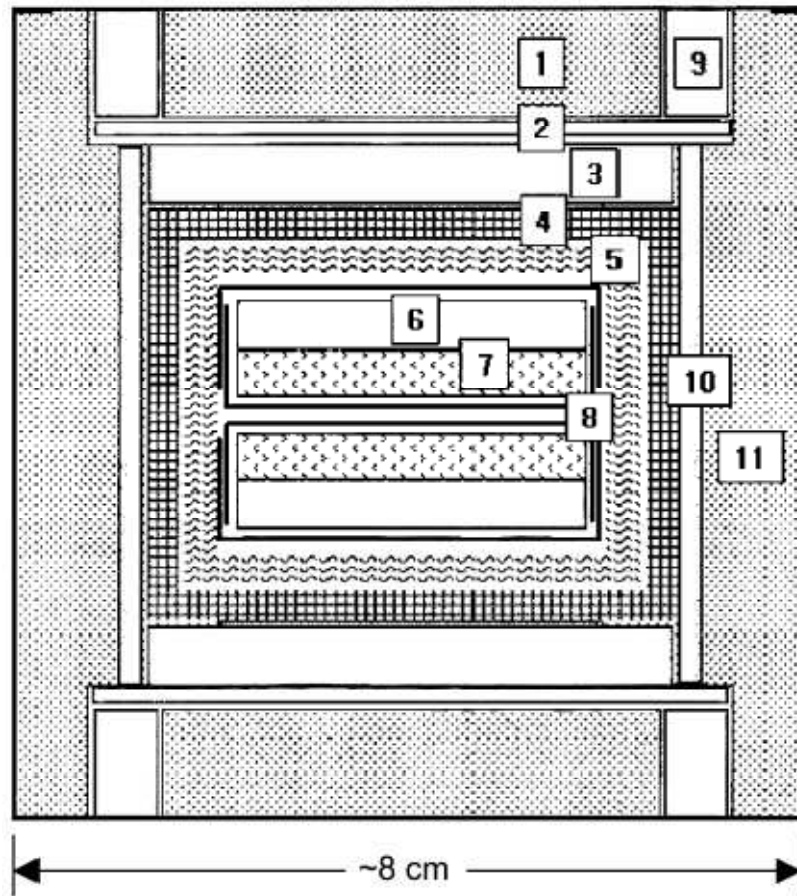
Figure 3.6: A typical HPHT assembly used for the sintering of PCD. 1) Pyrophyllite disc, 2) Mo end disc, 3) alumina disc, 4) Crucible, 5) salt nest, 6) WC-Co substrate, 7) diamond powder, 8) Nb cup and Ta double-cup, 9) current ring, 10) graphite heater, 11) pyrophyllite case. Adapted from [51].
