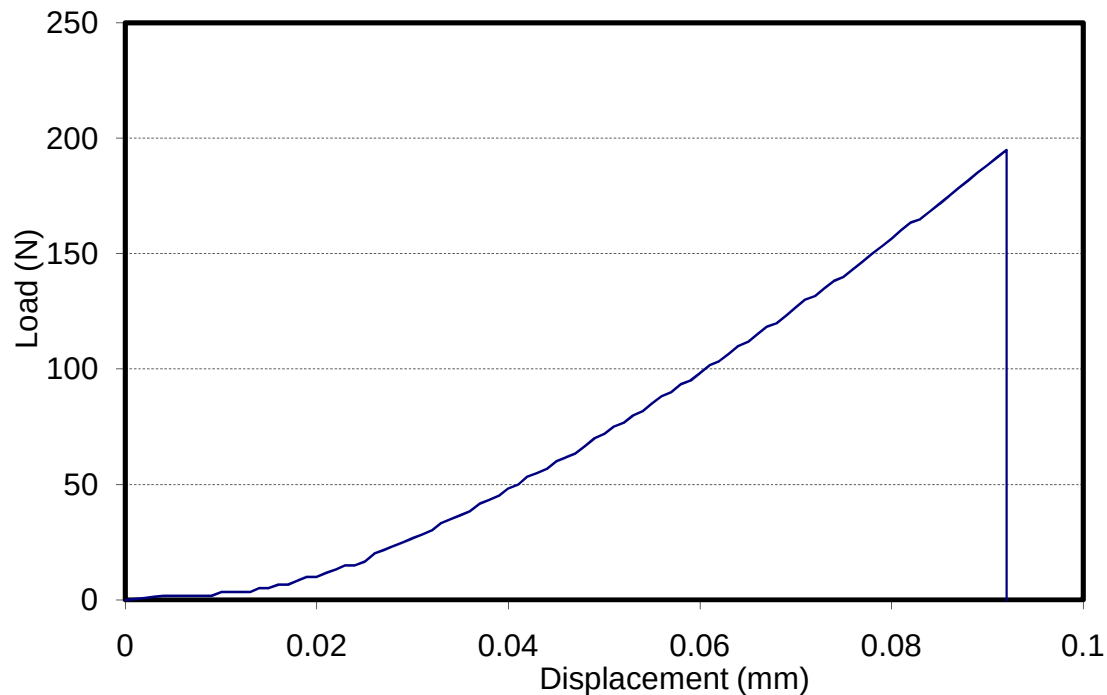
Figure 4.34: Load vs. displacement graph of the sintered diamond laminate as recorded during 3-point bend testing.
