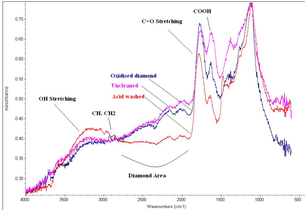
Figure 4.10: FTIR spectra of as received (uncleaned), oxidized and acid washed 0.5µm powder superimposed for comparison of surface groups.
