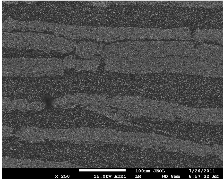
Figure 4.30: SEM micrograph of layer defects present in the diamond laminate.
