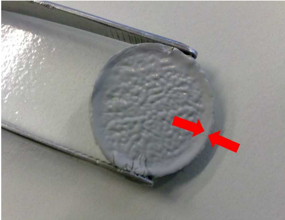
Figure 4.13: First diamond deposit obtained (Sample 47). The deposit was made using 3% (w/v), pH 8.5, 1.88 V/cm, 60 minutes.
