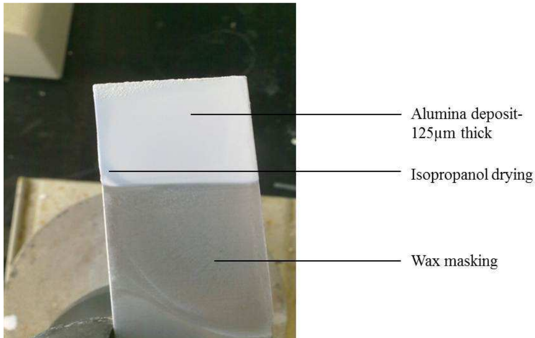
Figure 4.1: A typical electrode after deposition. This deposit was made at pH 5.7, 10% (w/v) alumina in isopropanol, 10 min at 100V/cm.
