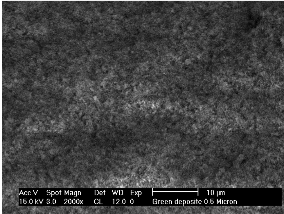
Figure 4.14: SEM image of the fracture surface of a green deposit made using a 0.5μm diamond suspension with the same conditions as sample 50.
