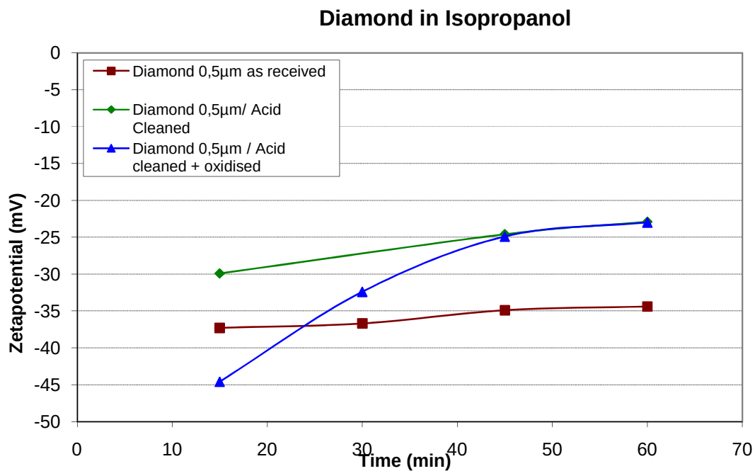
Figure 4.11: Zeta-potential measurements of as-received, acid cleaned as well as oxidized/acid cleaned powders plotted against time in isopropanol media.
