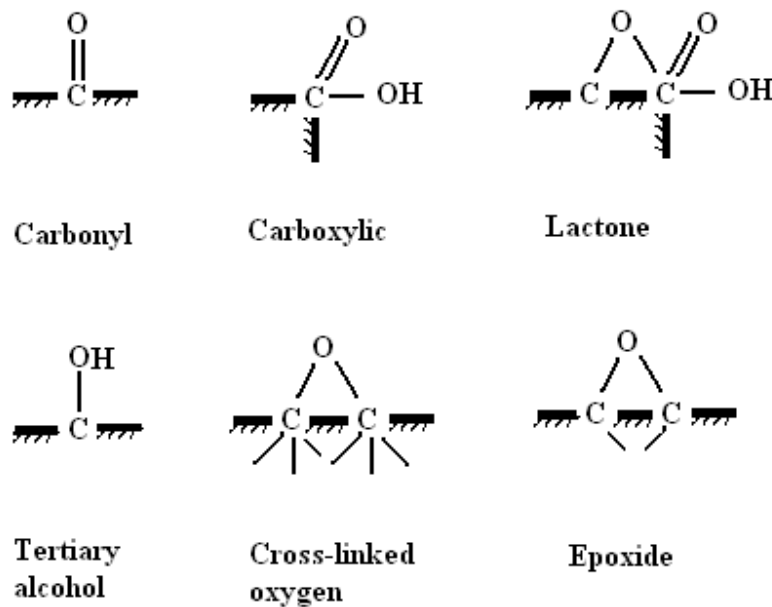
Figure 5.4: Some of the possible surface groups on diamond [66].
