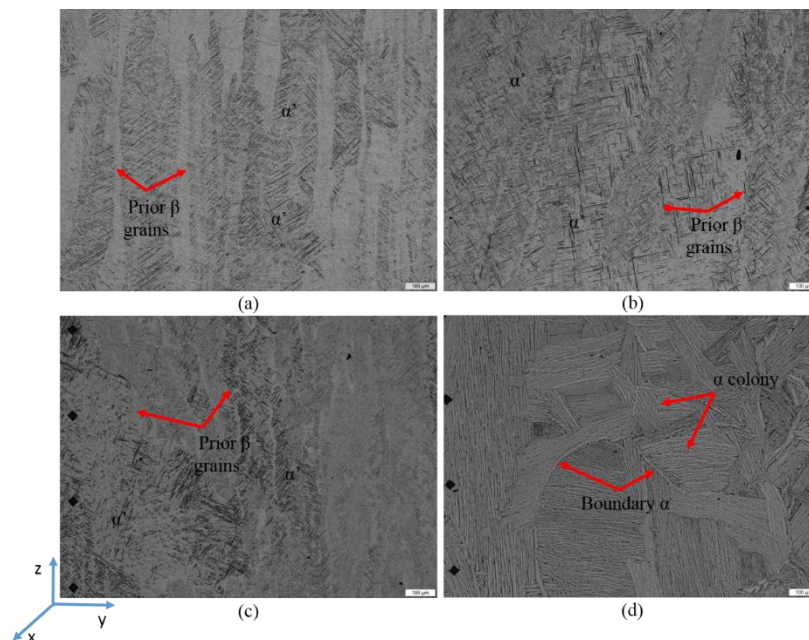
Figure 4.5: Microstructures of the sample after different cooling methods (a) As-received (b) WQ (c) AC and (d) FC after heat treatment at 1000°C and holding time of 2 hrs.
