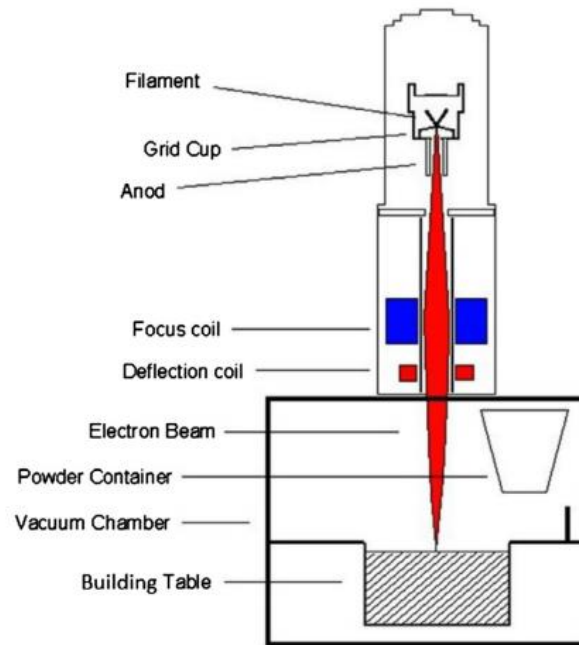
Figure 2.4: EBM process (Biamo et al. , 2010).
