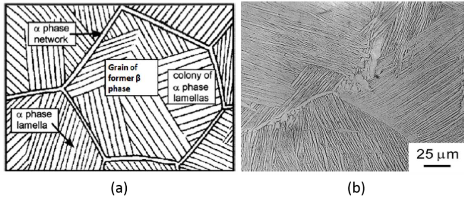
Figure 2.21: Ti6Al4V lamella microstructures (a) schematic diagram (Chraponiski and Szkliniarz, 2001), (b) Optical image (Nalla et al. , 2002).
