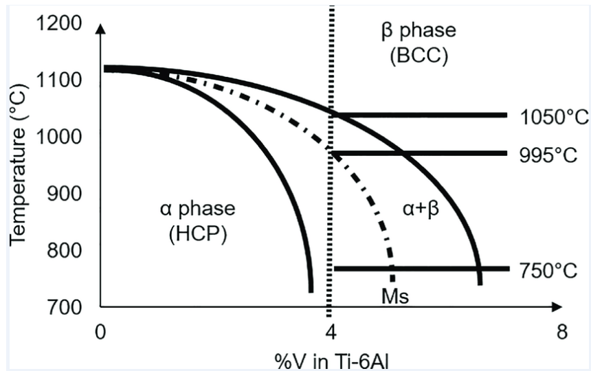
Figure 2.3: Phase diagram for Ti6Al4V (Majumdar et al , 2019).
