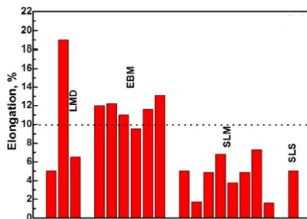
Figure 2.12: Elongation of Ti6Al4V components produced by different AM techniques (Yan and Yu, 2015).
