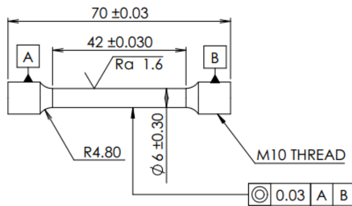
Figure 3.7: Schematic diagram of a tensile sample.
