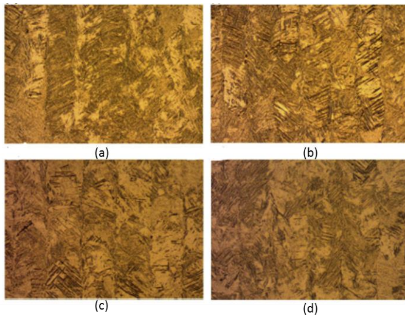
Figure 2.20: Ti6Al4V microstructures after heat treatment for 2 hrs followed by WQ (a) 800°C (b) 840°C (c) 875°C and 900°C (Wu et al. , 2016).
