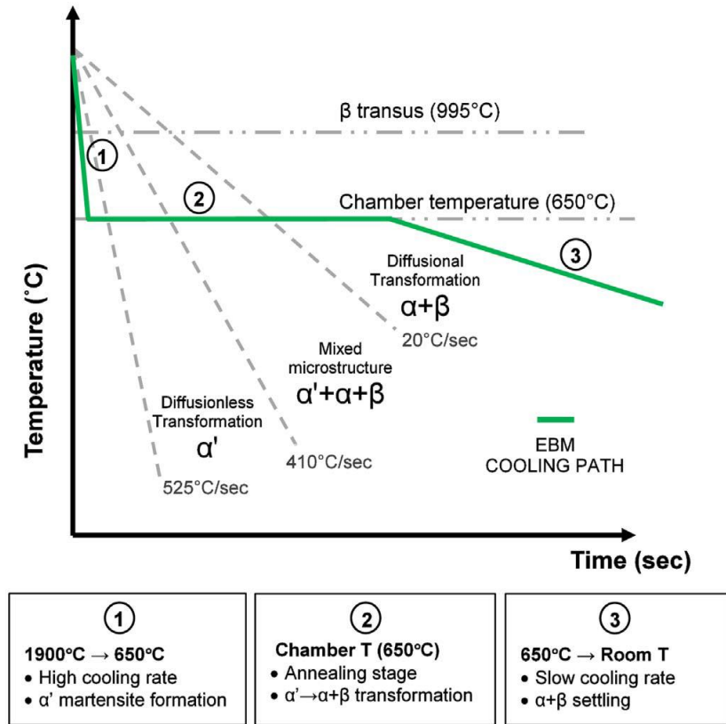
Figure 4.3: Cooling paths of Ti6Al4V (Galarraga et al. , 2017).
