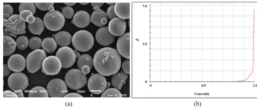
Figure 3.2: Convexity of the Ti6Al4V powder (a) SEM-SEI image, (b) Convexity curve.
