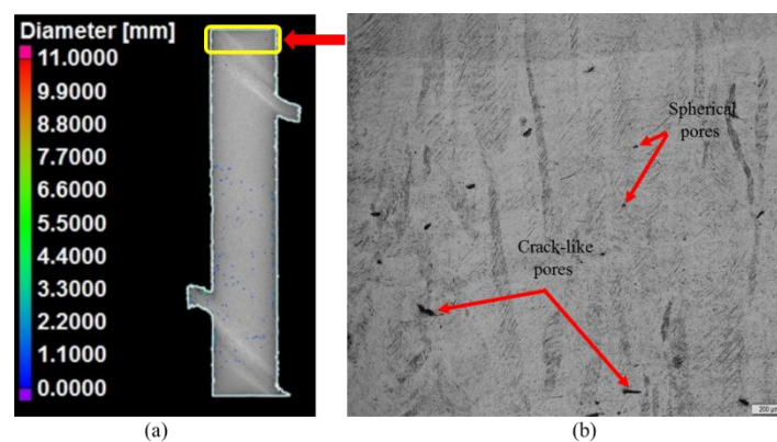
Figure 5.3: Images of the as-received Ti6Al4V sample (a) 2D micro-ct scan (b) Optical microstructure.
