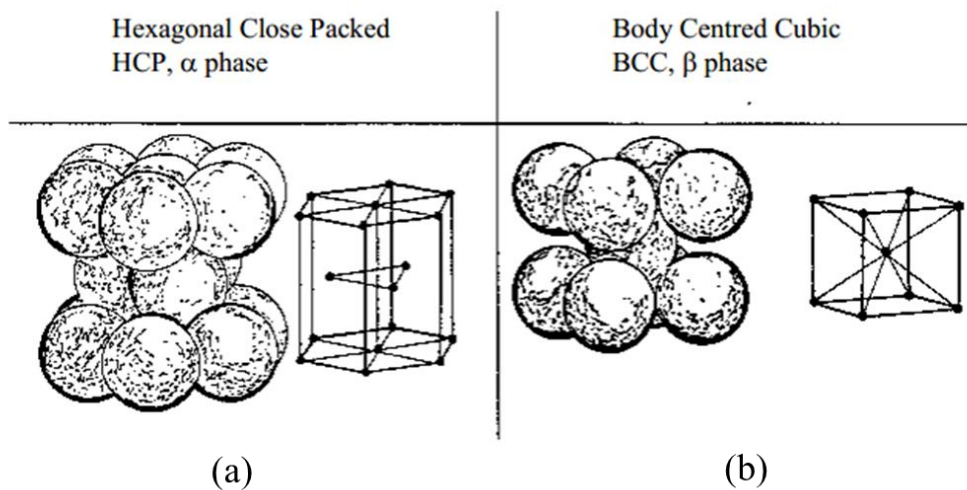
Figure 2.1: Crystal structures of titanium (a) hcp and (b) bcc (Pederson, 2002).
