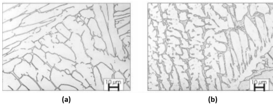
Figure 2.16: Ti6Al4V microstructures after heat treatment at 800°C (a) FC (b) WQ (Layens and Peters., 2003).
