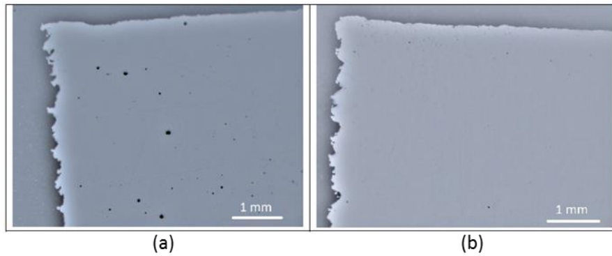
Figure 2.19: Ti6Al4V microstructures (a) As-built (b) HIPed (Eklund et al. , 2018).
