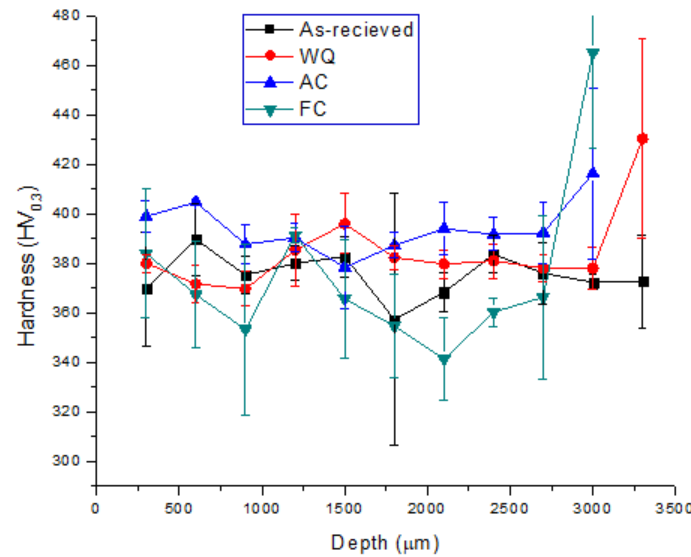
Figure 4.6: Hardness profiles of the samples after cooling with different methods.
