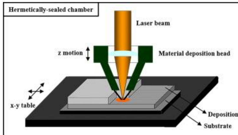
Figure 2.6: Schematic representation of LENS process (Zhai et al. , 2016).
