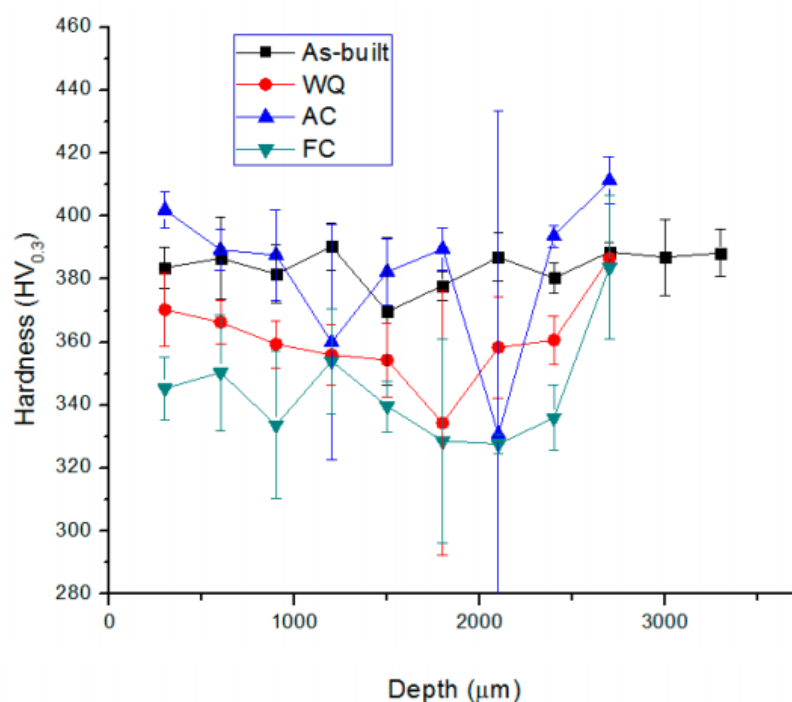
Figure 7. Hardness profiles of the as-built and heat-treated samples.
