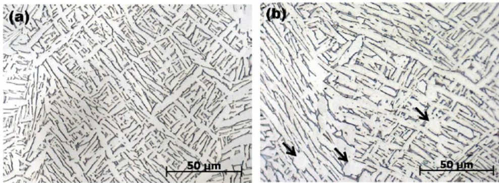
Figure 2.17: Ti6Al4V microstructures after heat treatment at 940°C for (a) 2 hrs, (b) 20 hrs (Vrancken et al. , 2012).
