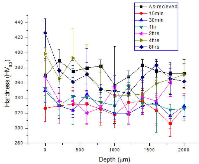
Figure 4.8: Hardness profiles of the samples after heat treatment at various residence times.
