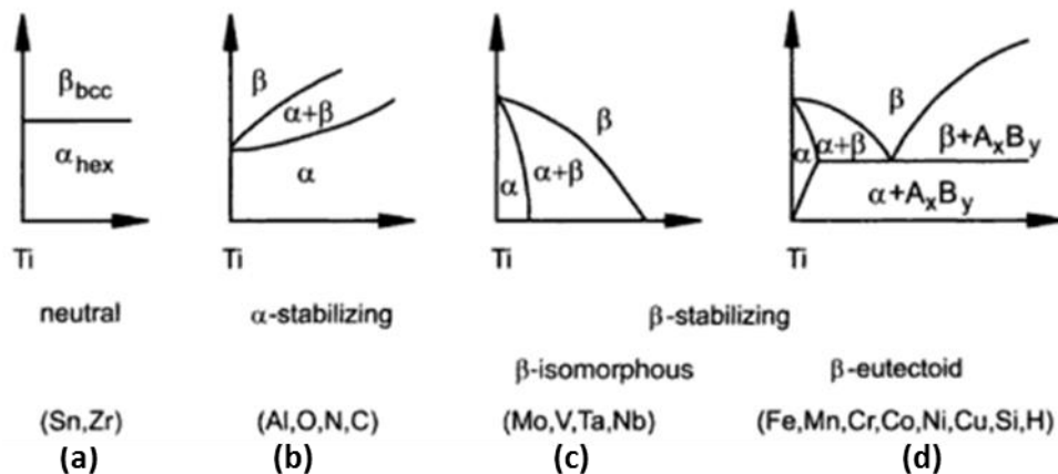
Figure 2.2: Illustration of alloying elements transformation temperatures (Leyens and Peters, 2003).
