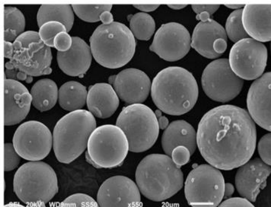
Figure 1. SEM image of the pre-alloyed Ti6Al4V Powder.
