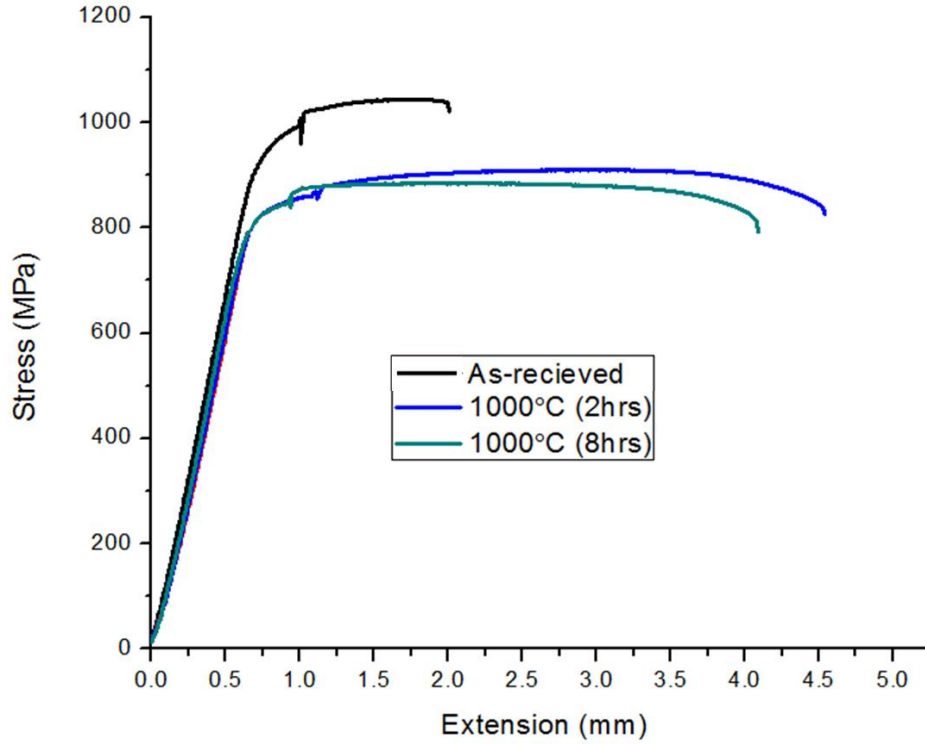
Figure 5.6: Stress versus extension curves of heat treated Ti6Al4V samples using optimized parameters.
