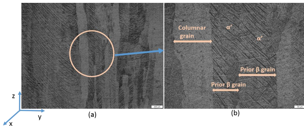
Figure 2.11: SLM produced Ti6Al4V microstructure at different magnifications (Lekoadi et al. , 2019).
