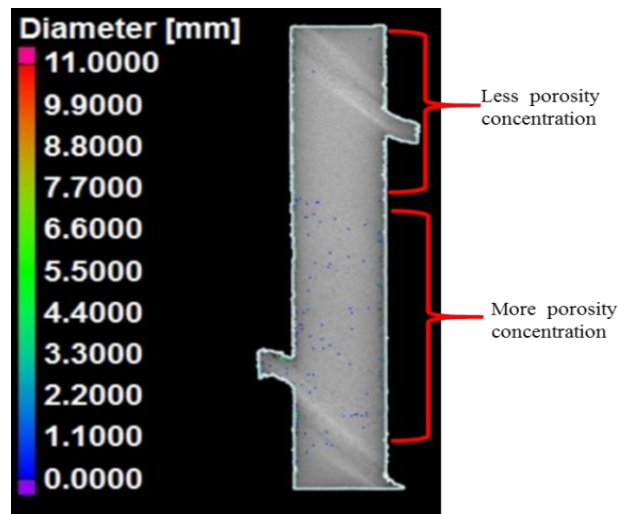
Figure 5.2: High resolution 2D micro-ct scan image of the as-received rod sample.
