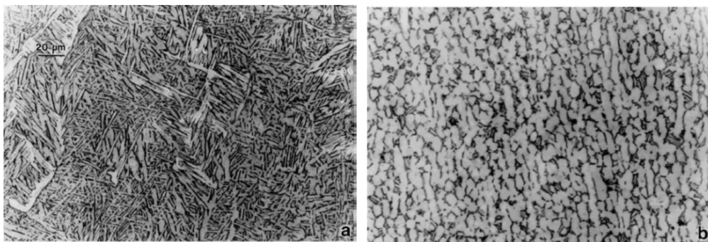
Figure 2.5: Microstructures of Ti6Al4V produced by (a) EBM and (b) Casting (Murr et al. , 2009).
