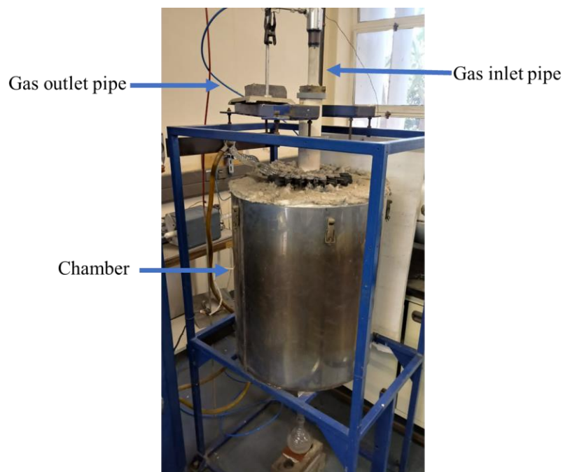
Figure 3.5: Vertical heat treatment furnace available at Pretoria University.
