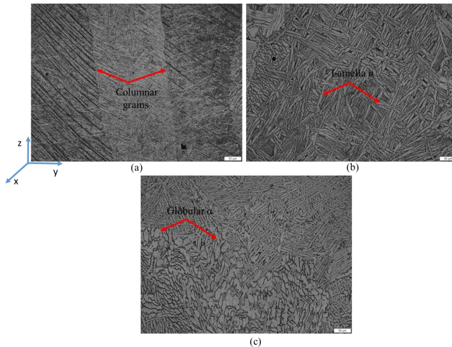
Figure 5.4: Microstructures of the as-received and heat treated samples using optimized parameters, (a) As-received (b) 1000°C for 2 hrs followed by FC and (c) 1000°C for 8 hrs followed by FC.
