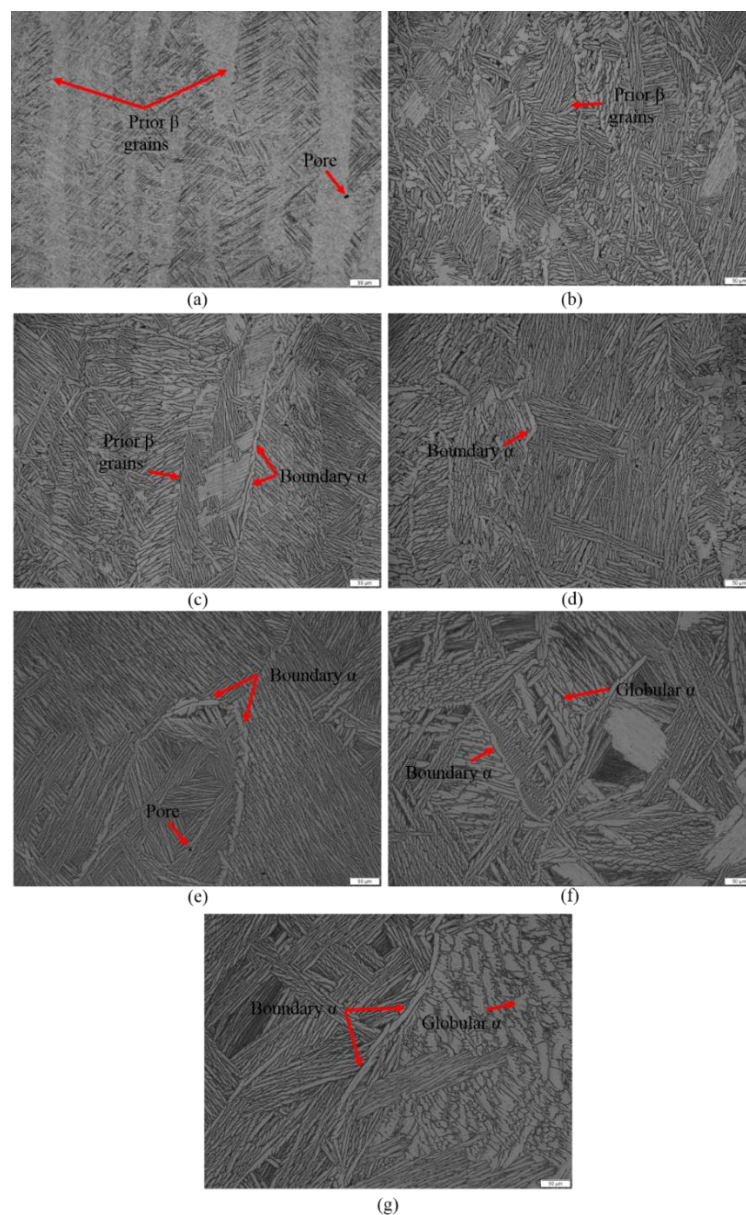
Figure 4.7: Microstructures of the samples (a) as-received, (b) 15 min, (c) 30 min, (d) 1 hr, (e) 2 hrs, (f) 4 hrs, and (g) 8 hrs.
