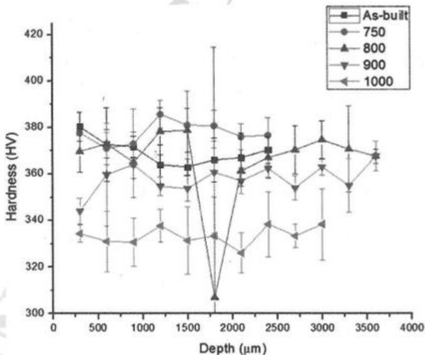
Fig. 3 Hardness profile of the as-built and heat-treated samples
