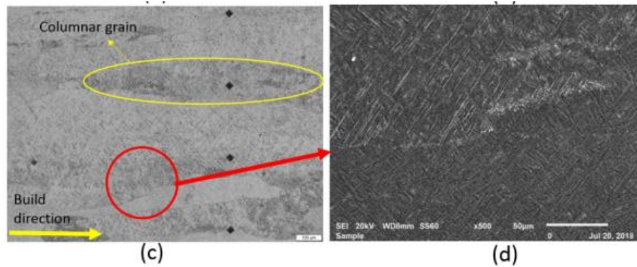
Figure 4: Micrographs of the samples after heat treated at 700 °C: (a and b) 42.41 J/mm 3 and (c and d) 78.46 J/mm 3 .
