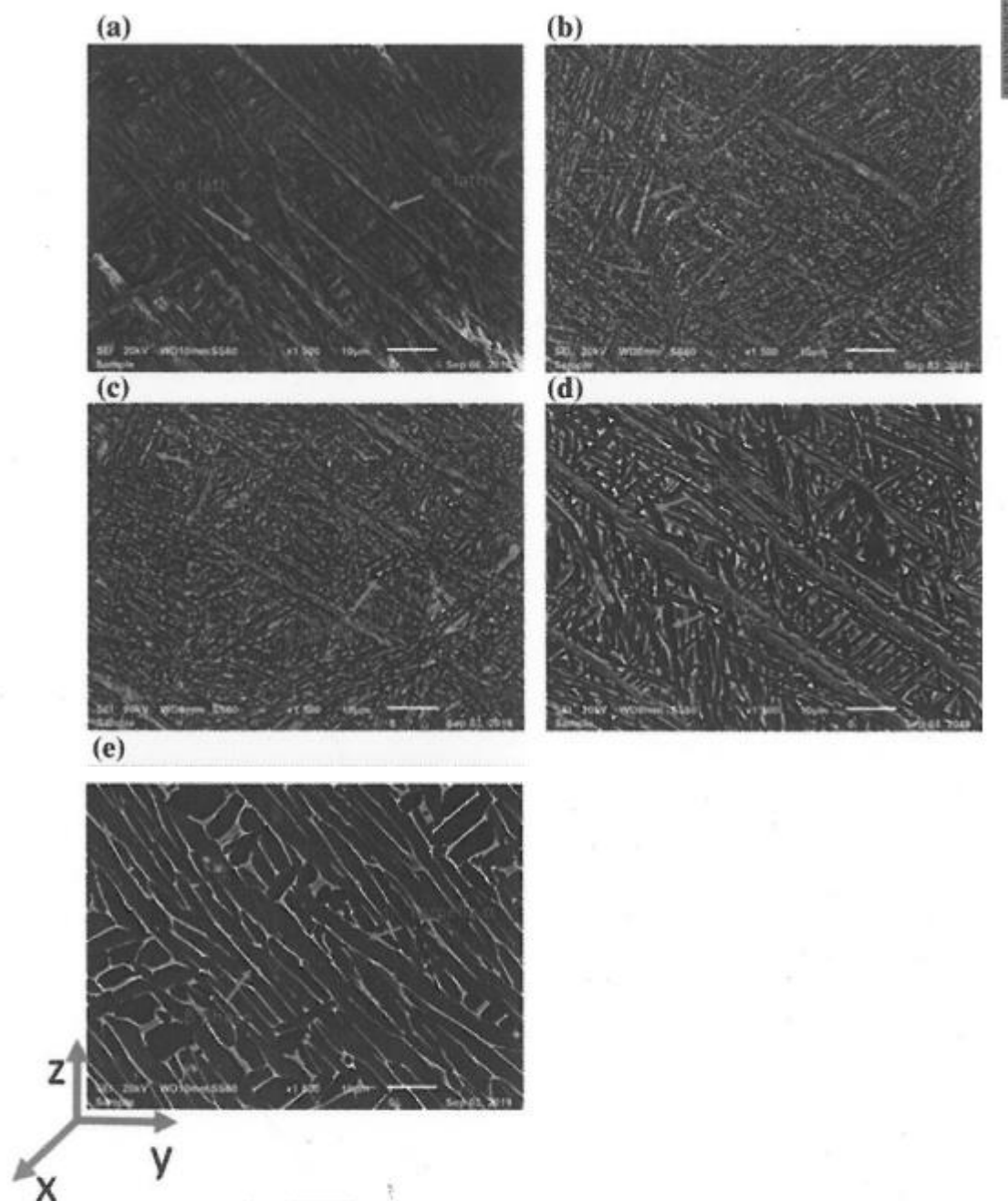
Fig. 1 SEM images of the samples a as-built, b 750 °C, c 800 °C, d 900 °C, and e 1000 °C
