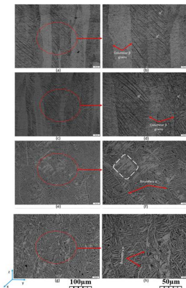
Figure 3. Optical microstructures of the samples: (a) As-built; (b) as-built zoom in; (c) 700 °C; (d) 700 °C zoom in; (e) 950 °C; (f) 950 °C zoom in; (g) 1000 °C; (h) 1000 °C zoom in.
