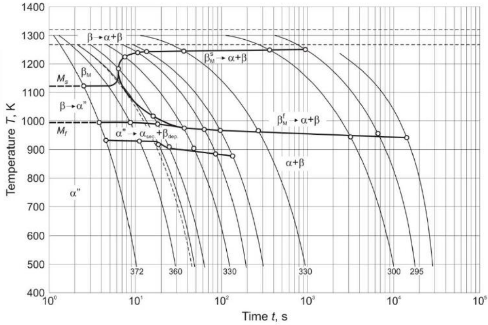
Figure 2.15: CCT diagram of Ti6Al4V (Seniawski et al. , 2013).
