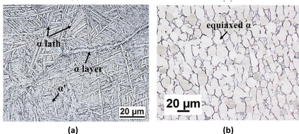
Figure 2.7: Microstructures of Ti6Al4V samples produced by (a) LENS technique (b) Wrought (Zhai et al. , 2016).
