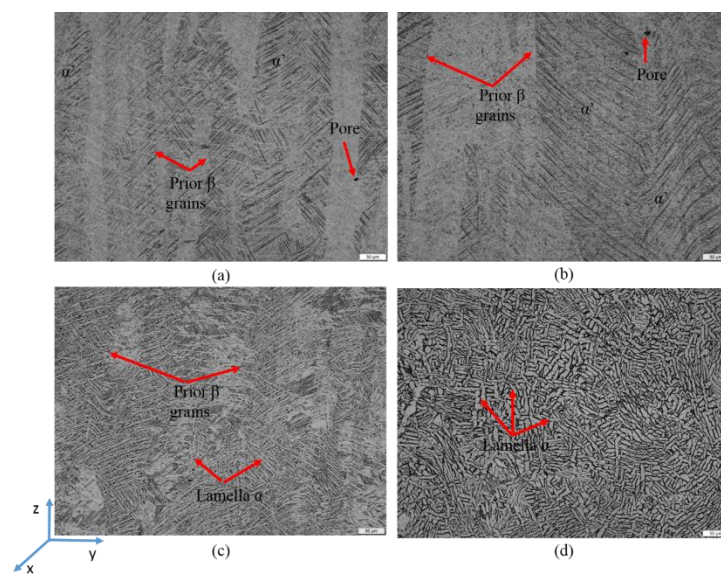
Figure 4.2: Microstructures of the sample after heat treatment at different temperatures (a) as-received, (b) 700°C, (c) 950°C and (d) 1000°C.
