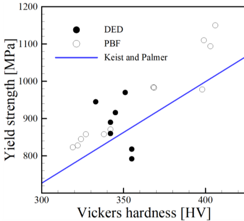
Figure 2.18: Relationship of hardness and yield strength of Ti6Al4V (Keist and Palmer, 2017).
