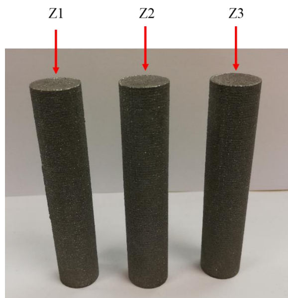
Figure 4.1: High speed SLM produced Ti6Al4V rod samples.
