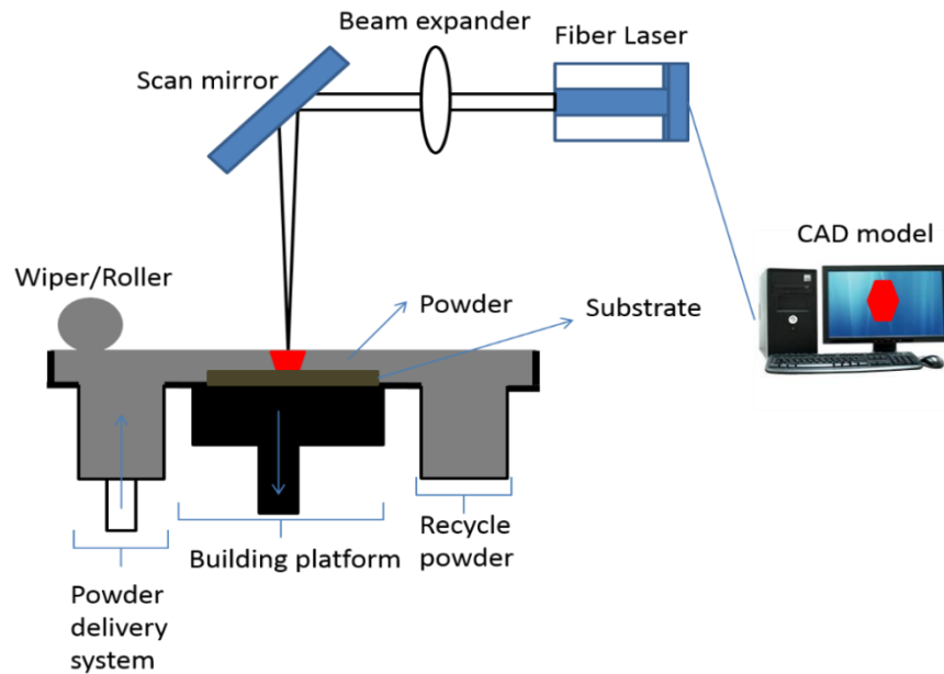
Figure 2.8: Schematic representation of SLM process.
