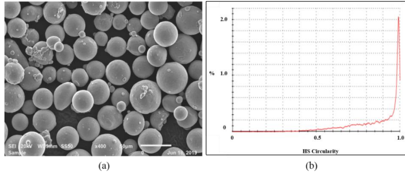
Figure 3.1: Powder morphology of the Ti6Al4V powder (a) SEM-SEI image, (b) HS circularity curve.
