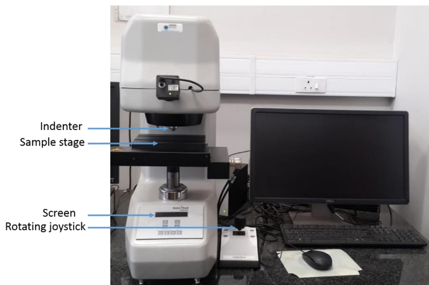
Figure 3.6: Micro-hardness testing machine available CSIR NLC.
