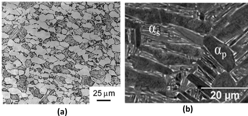
Figure 2.23: Ti6Al4V bimodal microstructures (a) Optical micrograph (Nalla et al. , 2002), (b) BSD-SE micrograph (Ter Haar et al. , 2018).
