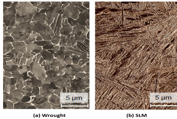
Figure 1.1: Microstructures of Ti6Al4V (a) Wrought, (b) SLM (Kasperovich et al. , 2015).
