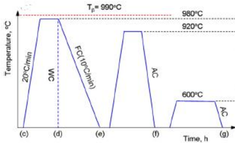
Figure 2.24: Illustration of triple heat treatment strategy (Zhao et al. , 2018).
