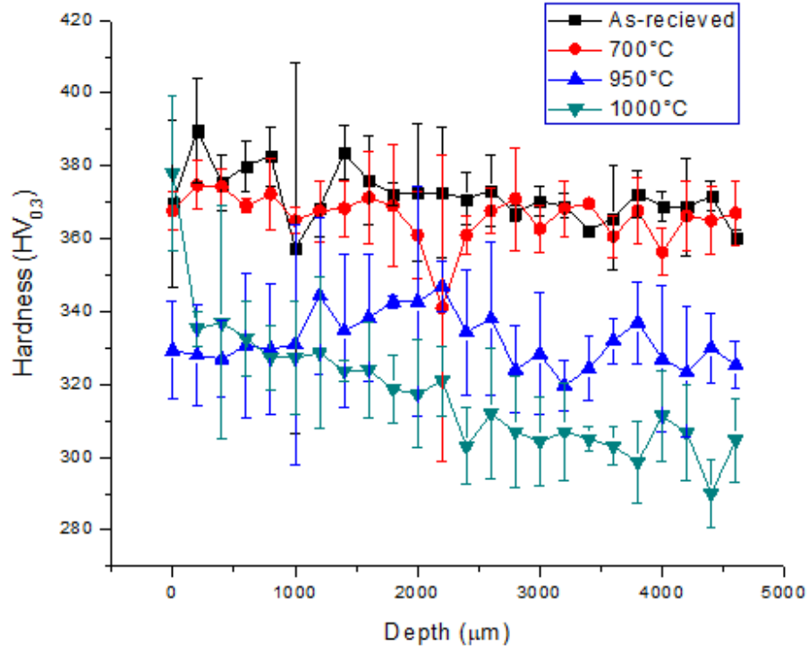
Figure 4.4: Hardness profiles of the samples after heat treatment at various temperatures.
