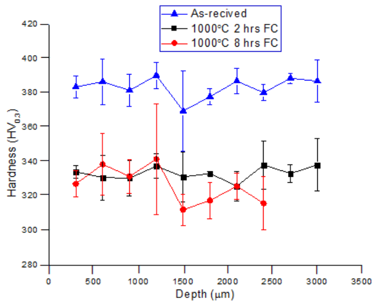
Figure 5.5: Hardness profiles of the as-received samples and the heat treated samples after heat treating using optimized parameters.
