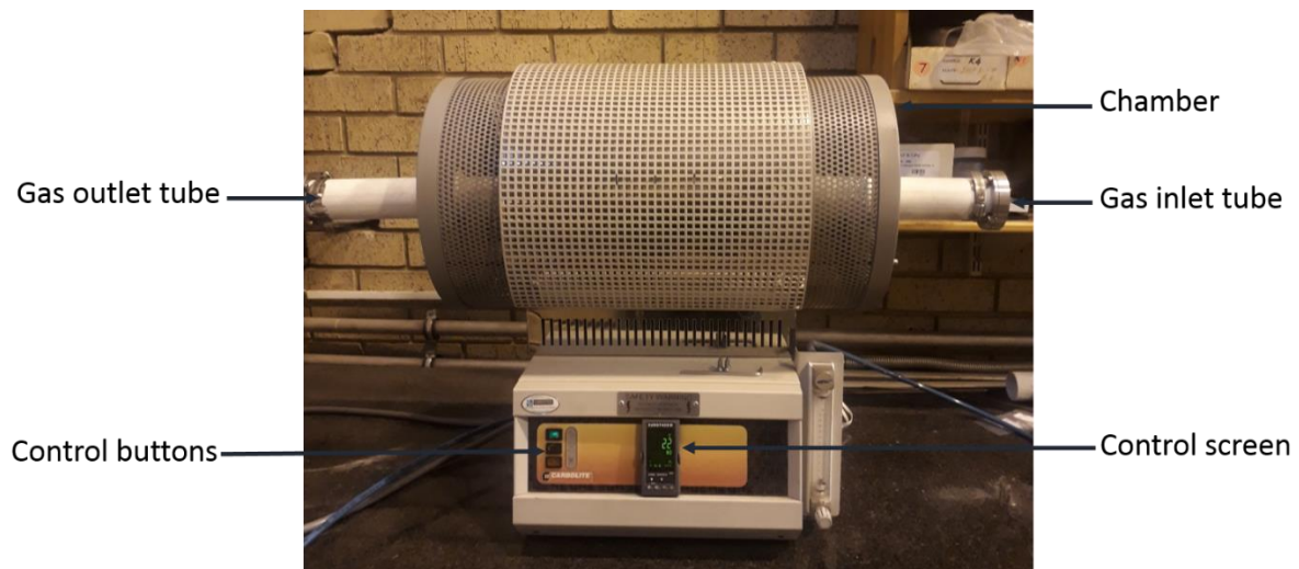
Figure 3.4: Horizontal heat treatment furnace available at the CSIR.
