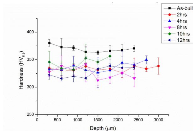
Figure 6: Average hardness profiles of the as-built and heat treated samples.
