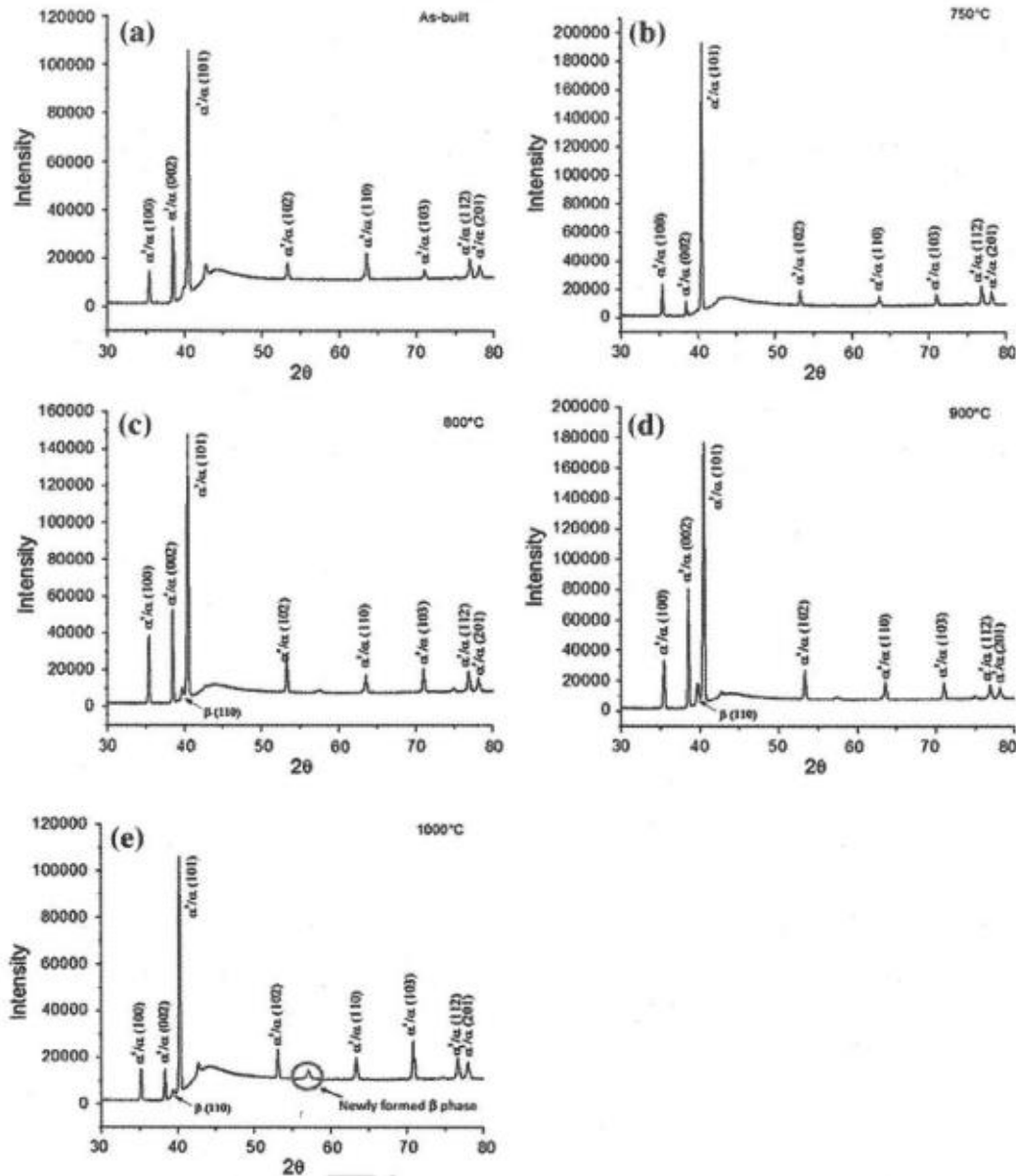
Fig. 2 XRD graphs of the as-built and heat-treated samples
