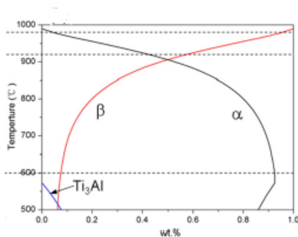
Figure 2.13: Illustration of phase fractions at elevated temperatures calculated by Thermo-Calc software (Zhao et al. , 2018).
