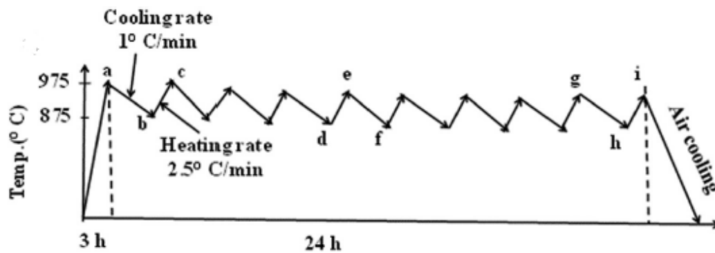
Figure 2.25: Illustration of cycling heat treatment (Sabban et al. , 2019).
