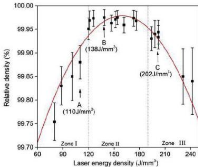
Figure 2.9: Relationship between energy density and relative density (Han et al. , 2017).
