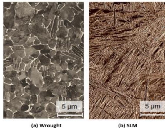
Figure 1: Microstructures of Ti6Al4V (a) Wrought, (b) SLM [14].
