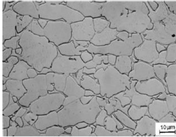
Figure 2.22: A fully equiaxed Ti6Al4V microstructure (Ivanova et al. , 2002).
