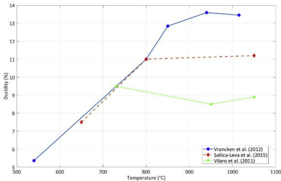
Figure 2.14: Relationship of heat treatment temperature and ductility (Shipley et al. , 2018).
