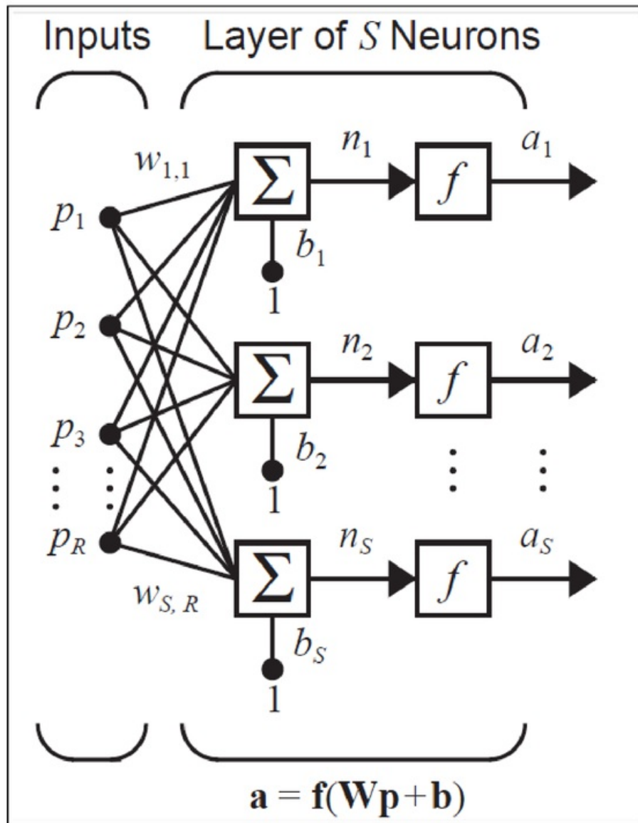
Figure 4.7: A layer of S neurons [2]
