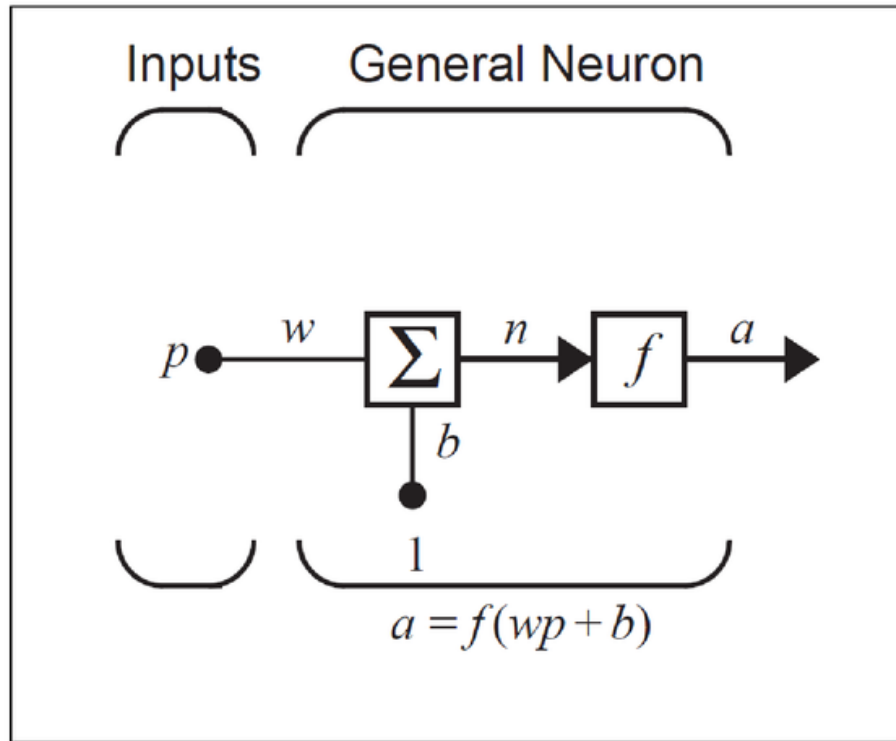
Figure 4.3: Single input neuron [2]
