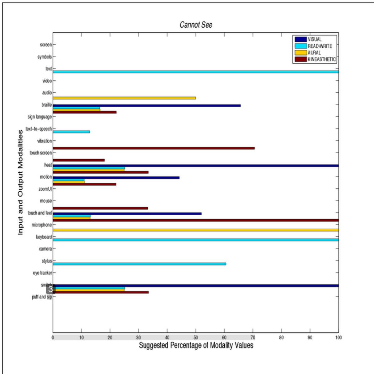
Figure 5.13: Importance values for a lazy trainee who cannot See
