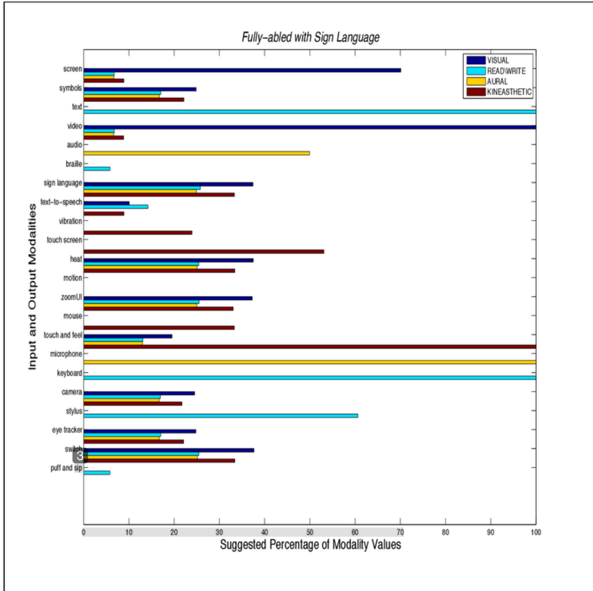
Figure 5.15: Importance values for a lazy Fully-able trainee
