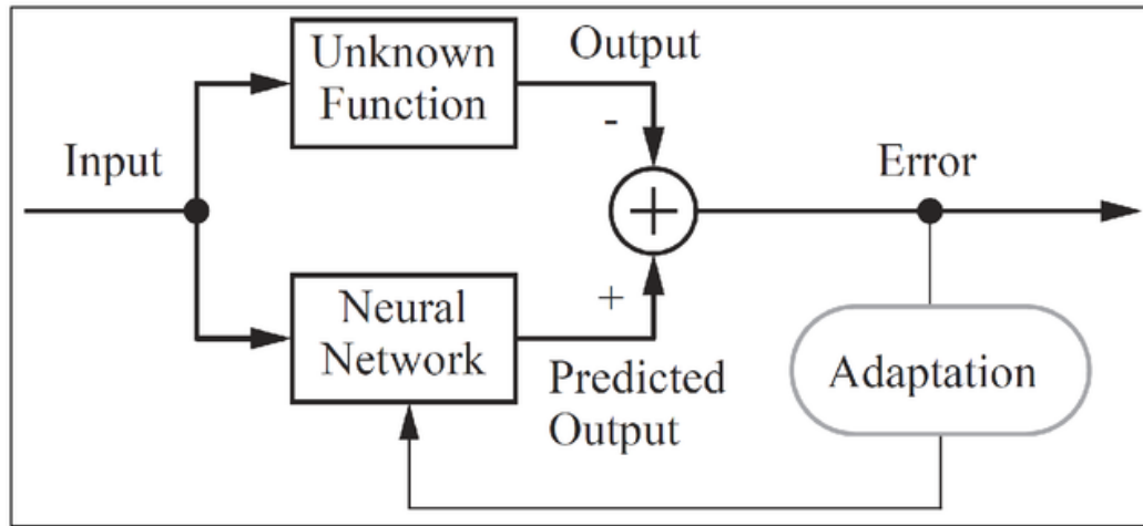
Figure 4.1: Neural Network as a function approximator [2]
