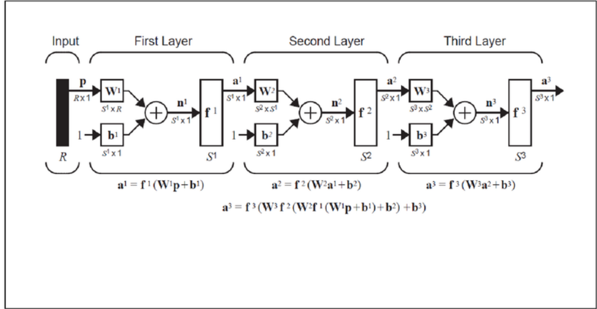
Figure 4.9: Three layer network [2]
