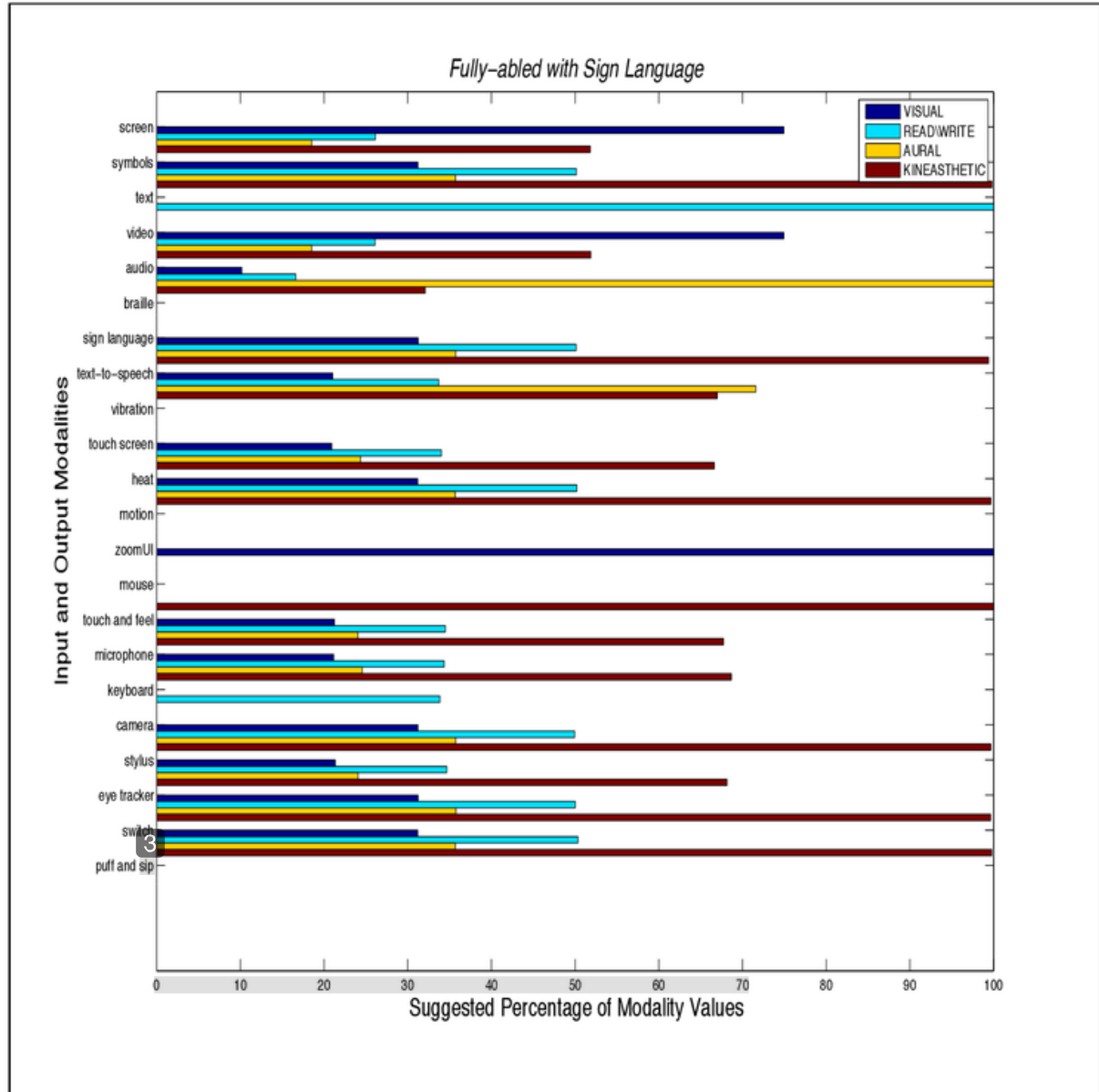
Figure 5.19: Importance values for a tired Fully-able trainee
