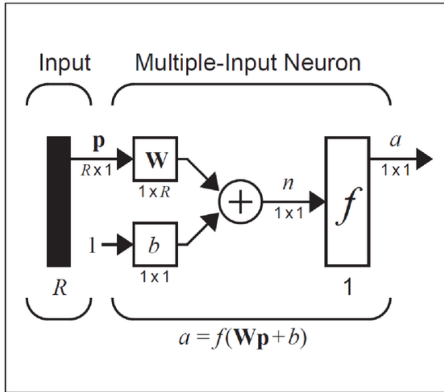
Figure 4.6: Neuron with R inputs [2]
