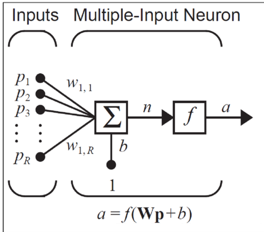
Figure 4.5: Multiple input neuron [2]
