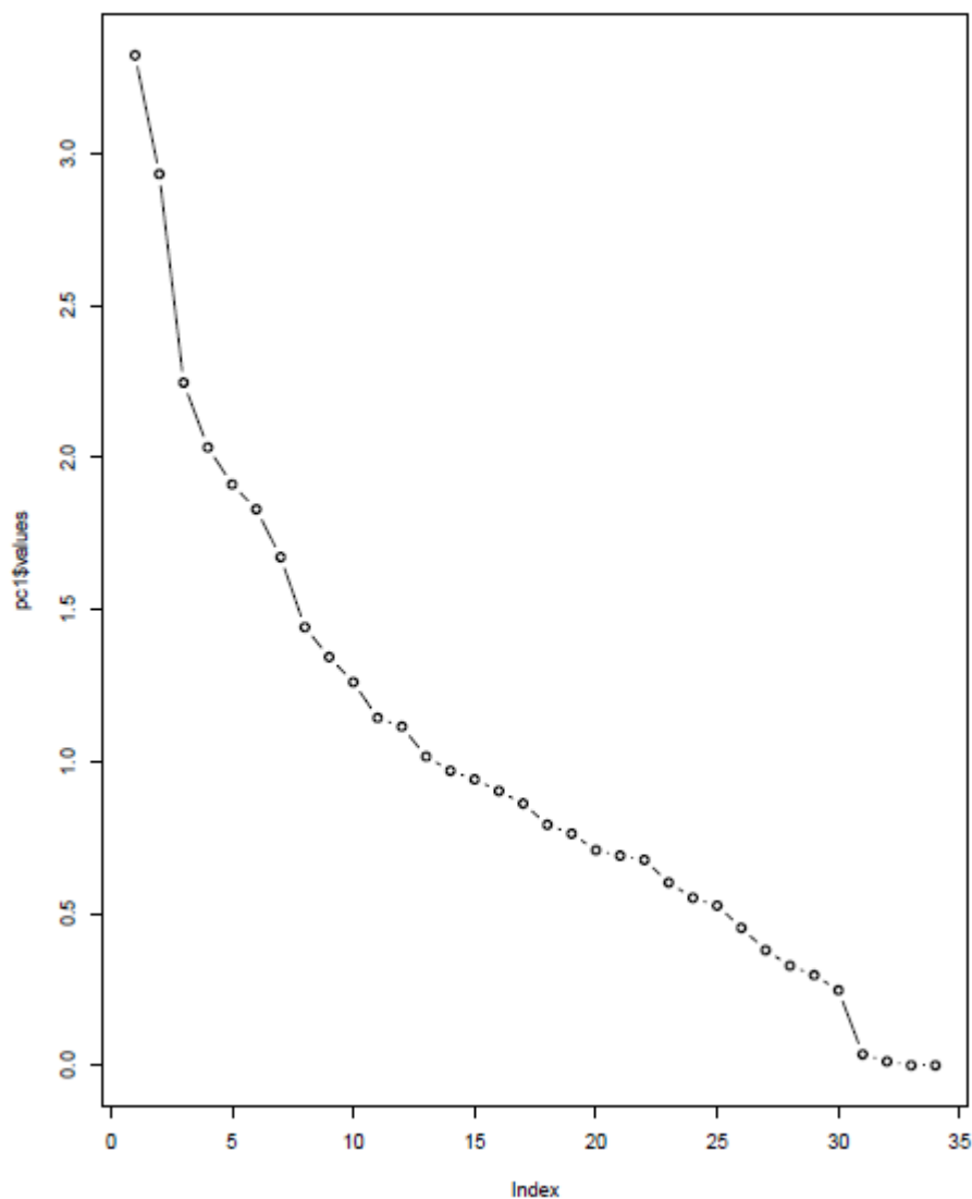
Graph 3: Scree plot
