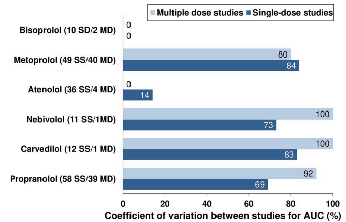
Figure 1. Variability of exposure to different \beta -blockers from a systematic review of pharmacokinetic studies. Information in parentheses next to drug names is (number of studies involving single dose [SS] administration/number of studies involving multiple dose [MD] administration to pharmacokinetic steady state). AUC, area under the plasma concentration-time curve. Note that the 100% values for nebivolol and carvedilol are based on a single available study. Drawn from data presented in reference 33 .
