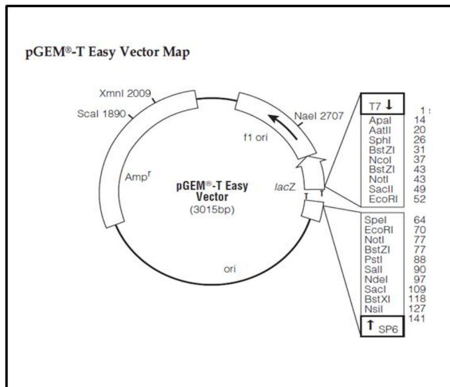
Figure 13: The p GEM® -T Easy Vector Map: pGEM®-T easy vector 3015bp in size and it is a linearized vector with a single 3'-terminal thymidine (T) at both ends. The T- overhangs at the insertion sites greatly improve the efficiency of ligation of PCR products by preventing re-circularization of the vector and providing a compatible overhang for PCR products, generated by certain thermo stable polymerases. The pGEM®-T easy vectors are high copy number vectors containing T7 and SP6 RNA polymerase promoters flanking a multiple cloning region within the \alpha - peptide coding region of the enzyme \beta -galactosidase. Insertional inactivation of the \alpha - peptide allows identification of recombinants by blue/white screening on LB agar plates with ampicillin. These vectors contained numerous restriction enzyme sites within the multiple cloning regions.
