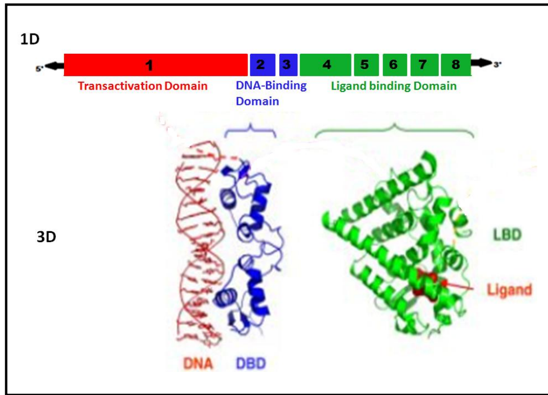
Figure 9b: Structural organization of androgen receptor. Top: Schematic 1D amino acid sequence of androgen receptor. Bottom: 3D structures of DBD bound to DNA and LBD bound to hormone regions of androgen receptor. This figure is adopted from the website ( http://en.wikipedia.org/wiki/Nuclear_receptor ).
