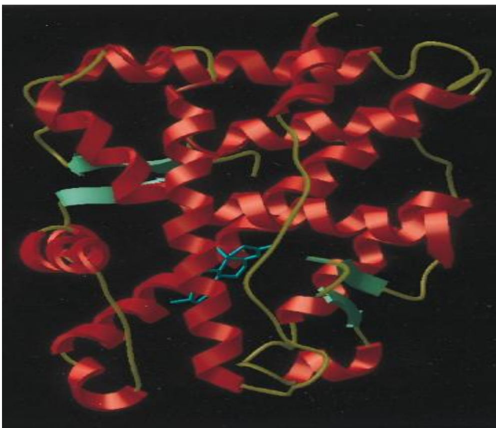
Figure 9a: The 3D-crystallographic structure of AR LBD. Reprinted with permission from Proceedings of the National Academy of Sciences, 2001, USA. (Adapted from John.S.Sack et al. , 2001).
