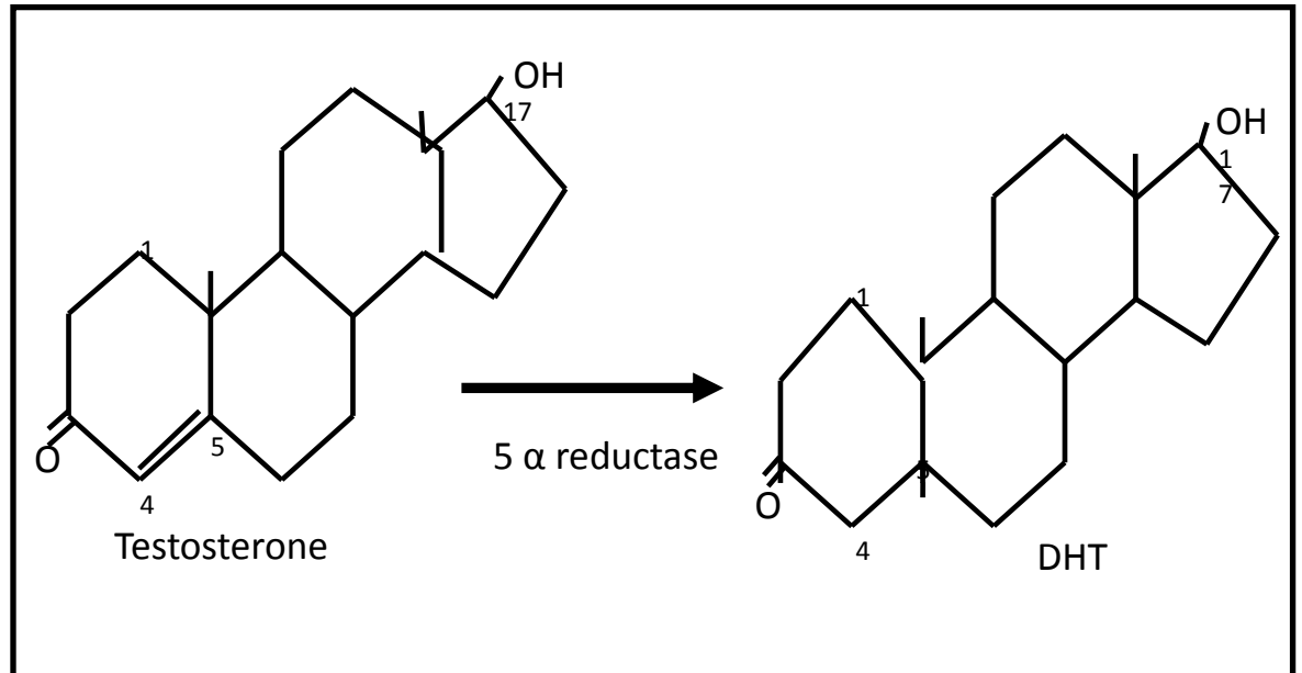
Figure 2: The chemical structure of dihydrotestosterone (DHT) and testosterone (T). The conversion of T to DHT by the enzyme 5α reductase. The double bond existing between position 4 and 5 of T is reduced to a single bond in DHT.
