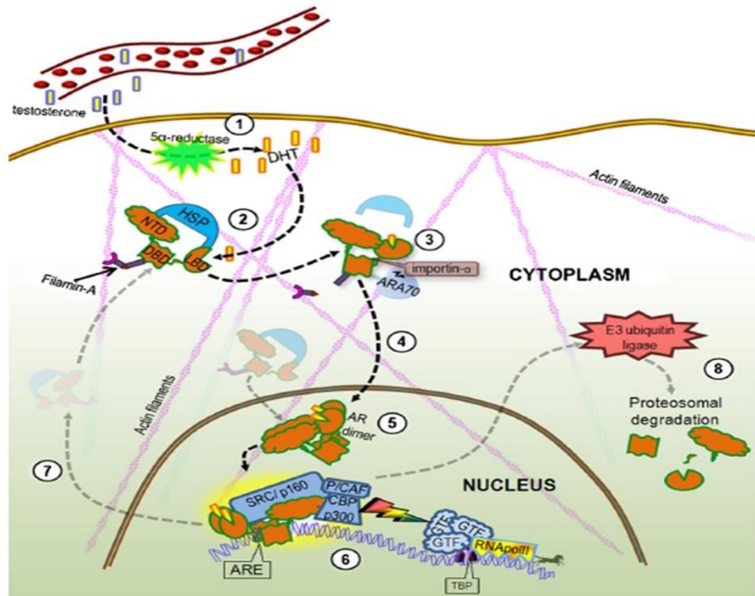
Figure 10: AR cycle. The androgen receptor (AR) (coloured orange) is illustrated as a modular protein with each of its domains represented; NTD (N-terminal transactivation domain), DBD (DNA-binding domain), the hinge and the LBD (ligand-binding domain). (1) Conversion of testosterone to DHT via the enzyme 5 \alpha -reductase in basal epithelial cells within the prostate; (2) DHT moves into the cytoplasm of epithelial cells where it is bound by AR; (3) Ligand binding to AR induces an AR conformational change, whereby proteins such as heat shock proteins (HSPs) dissociate and others such as importin- and the androgen receptor-associated protein-70 (ARA70) are recruited to help stabilise AR and (4) promote AR nuclear translocation; (5) AR dimerises in the nucleus; (6) Numerous other co-activators bind to the AR in the nucleus, then the AR-DBD facilitates nucleic acid binding at androgen response elements (ARE) which promote the recruitment of co-activators with histone acetyltransferase (HAT) activity (CBP/p300, P/CAF), via SRC/p160 co-activator family members, resulting in chromatin remodelling. This allows the binding of the TATA binding protein (TBP), followed by general transcription factors (GTF) and RNAPolII to begin transcription; (7) Non-ligand-bound AR is shuttled back to the cytoplasm and recycled in preparation for further ligand binding. (8) Alternatively, non-ligand-bound AR can be targeted for proteosomal degradation following ubiquitination by E3 ubiquitin ligase. Reprinted with permission from, the International Journal of Biochemistry and Cell Biology, 2010. (Adapted from Bennett et al. , 2009).
