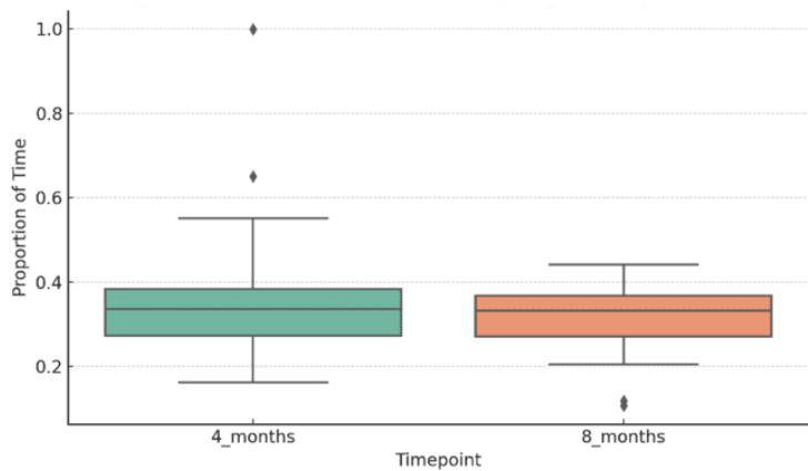
Figure 3. Proportion of time in high synchrony ( r \geq 0.50 ) at 4 and 8 months.
