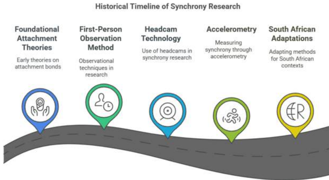
Figure 5 Timeline depicting major historical milestones in mother-infant synchrony research, tracing foundational attachment theories through contemporary methodological innovations (first-person observation, headcams, accelerometry). Special emphasis is given to advancements and adaptations within the South African research context, as discussed in Section 1.3.5.
