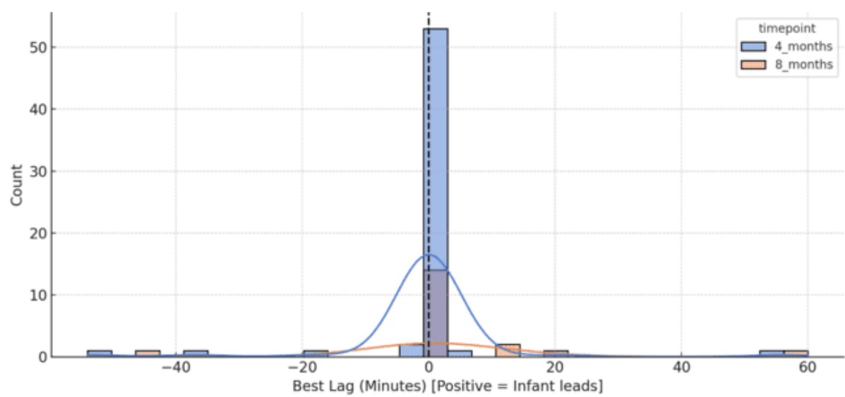
Distribution of Lead-lag in Synchrony (best_lag_minutes)
