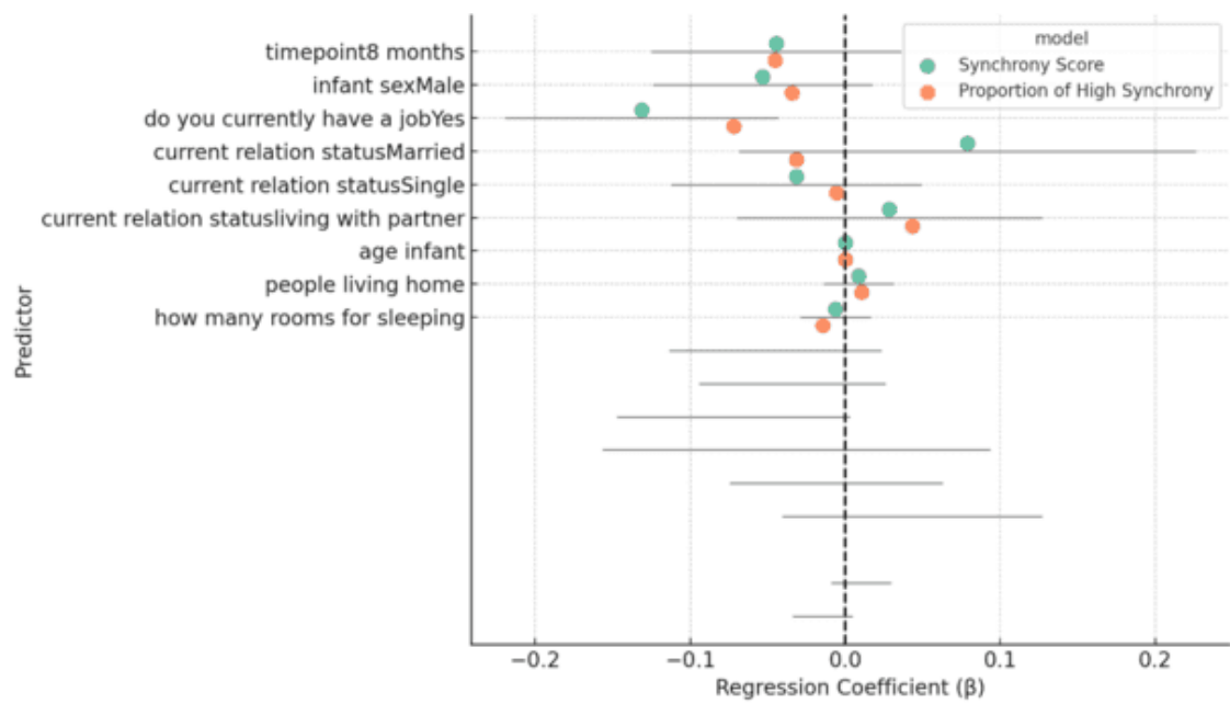
Figure 410 Coefficient Plot of Predictors of Mother–Infant Synchrony.
