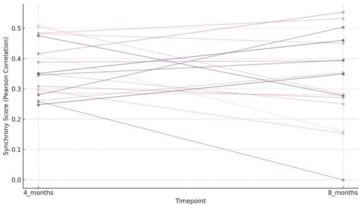
Figure 1. Change in mother–infant synchrony scores within dyads from 4 to 8 months. Lines represent dyads measured at both timepoints; trajectories illustrate within-dyad variability with no consistent directional shift.
