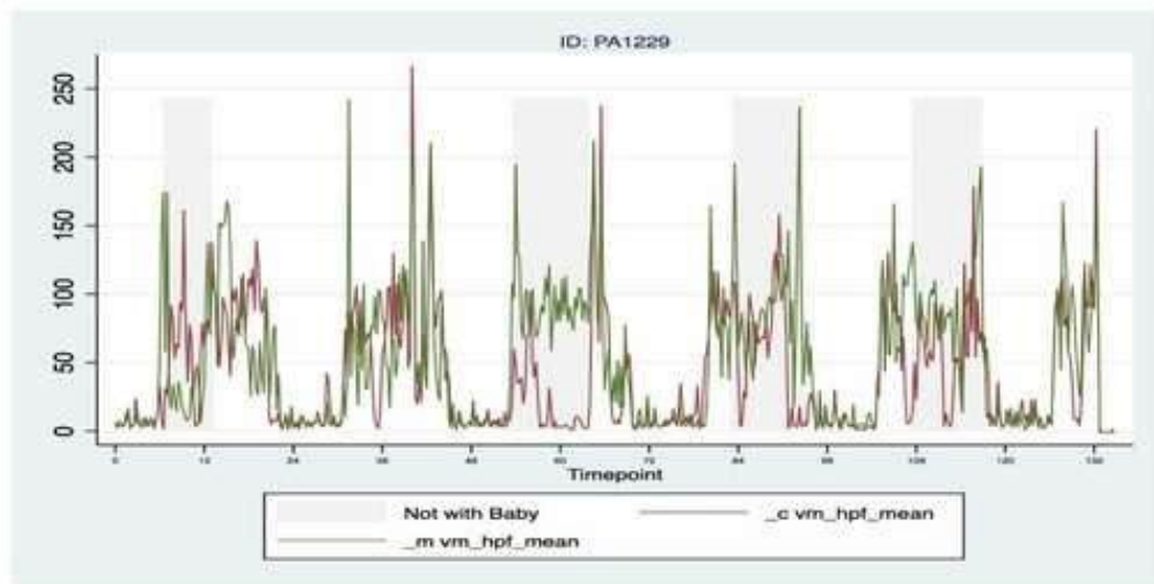
Figure 3 An example of movement time series for mother and infant 64
