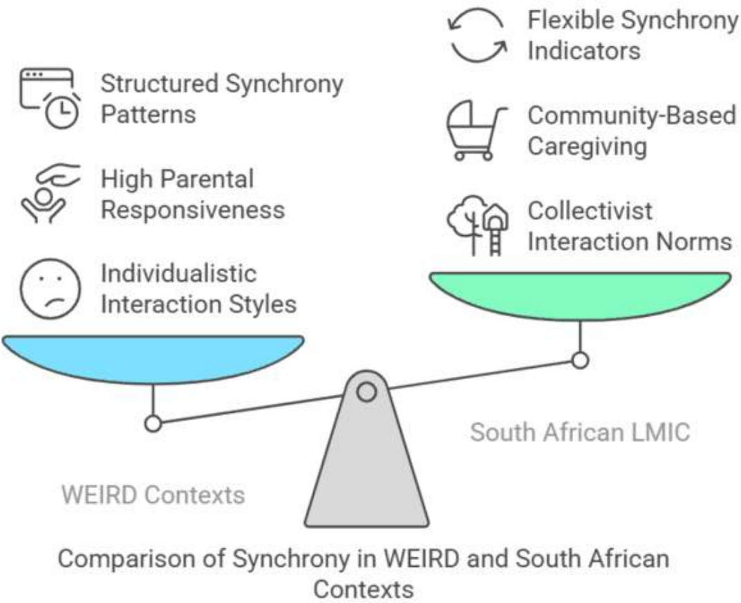
Figure 6 Comparative analysis of caregiving practices and synchrony indicators in WEIRD (Western, Educated, Industrialized, Rich, Democratic) contexts versus Low- and Middle-Income Countries (LMICs), specifically highlighting South African caregiving norms. The table emphasizes differences in interaction styles, parental responsiveness, and synchrony patterns discussed in detail in Section 1.3.5.
