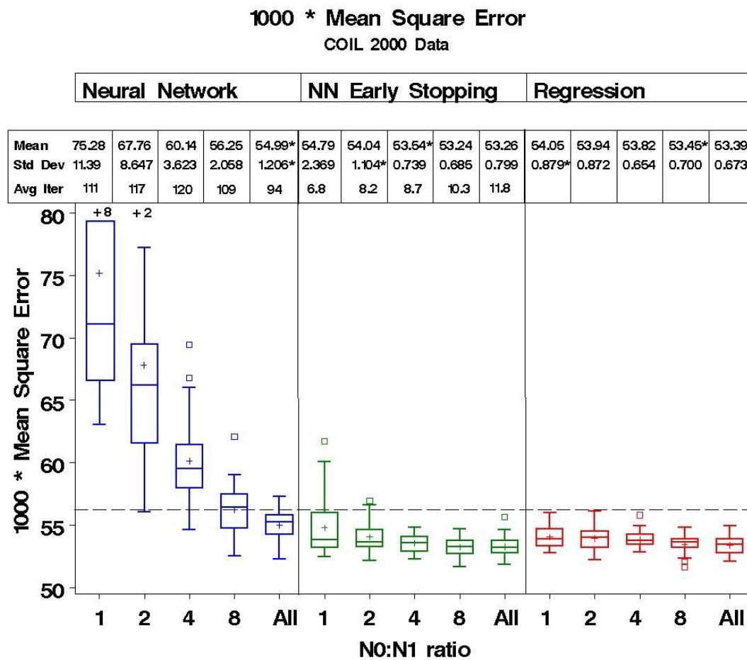
Figure 5.5: 1000 times MSE for the COIL 2000 data.
