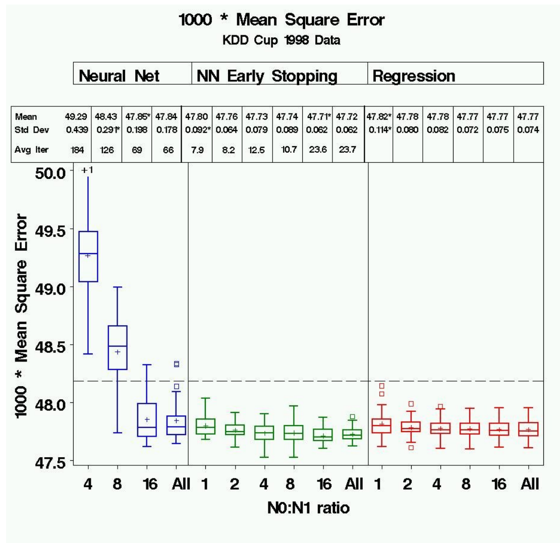
Figure 5.3: 1000 times MSE for the KDD Cup 1998 data. All runs for neural network without early stopping at ratios 1 and 2 produced values larger than the maximum value shown on the y-axis.
